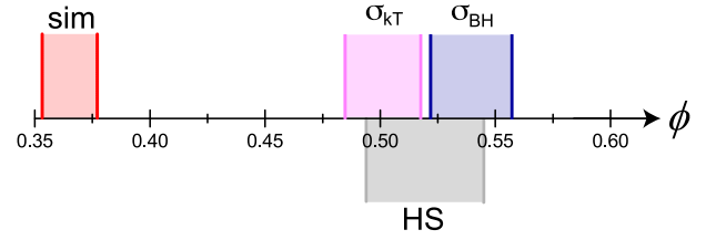
FIG. 6. Mapping the phase behavior of weakly charged hard-core colloids to pure hard spheres. The hypothetical particles have a diameter \sigma = 2 \mu\text{m} and an electrostatic charge Z = 500 . The Debye screening length of the solvent is \kappa^{-1} = 100 \text{ nm} , which is typical for nonaqueous solvents (Royall, van Roij, and van Blaaderen, 2005). The fluid-solid coexistence gap of the hypothetical charged-colloid system as a function of the packing fraction \phi is taken from simulations (red, “sim”) (Hynninen and Dijkstra, 2003) and is mapped to pure hard spheres while assuming that the effective hard-sphere diameter corresponds to the interaction potential \beta u(\sigma_{\text{KT}}) = 1 (lilac, \sigma_{\text{KT}} ) and using the mapping of Eq. (8) (blue, \sigma_{\text{BH}} ). The phase diagram of pure hard spheres (gray, HS) is shown for comparison.
