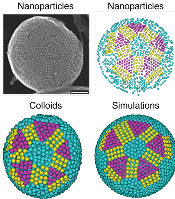
FIG. 31. Icosahedral clusters of spheres self-assembled in spherical confinement. Top row: an electron microscopy image of a cluster of nanoparticles and a reconstruction of its surface layer. Bottom left image: cluster obtained in experiments with micron-sized colloids. Bottom right image: cluster obtained in simulations of hard spheres. Adapted from de Nijs et al. , 2015 .
