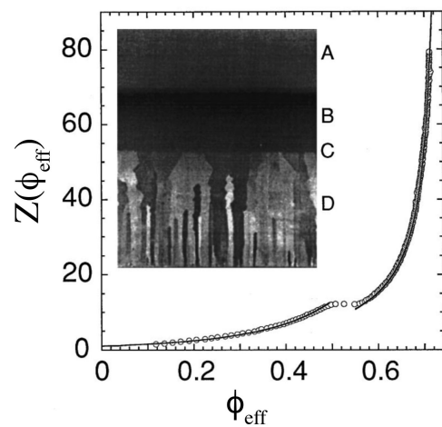
FIG. 12. Experimental determination of the EOS, i.e., Z(\phi_{\text{eff}}) = \beta P(\phi_{\text{eff}})/\rho_{\text{eff}} vs \phi_{\text{eff}} , for \sigma = 0.720 \mu\text{m} PMMA particles from the observed sedimentation-diffusion equilibrium: (A) supernatant, \phi_{\text{eff}} \approx 0 ; (B) fluid phase, 0 < \phi_{\text{eff}} \leq 0.492 ; (C) sharp interface; and (D) crystalline phase, 0.543 \leq \phi_{\text{eff}} \leq 0.74 . The lines denote the fluid and solid EOSs for true hard spheres. Inset: photograph of 1 cm of the sample. Adapted from Rutgers et al. , 1996.
