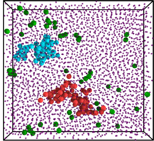
FIG. 38. Dynamical heterogeneity in real space is identified by highlighting the locations of the fastest particles (larger spheres) compared to the other particles (smaller spheres). The latter are drawn smaller for clarity; the particles all have the same physical size, which is the displayed size of the large spheres. Shown is a supercooled sample with \phi \approx 0.56 and measurement time \Delta t^* = 1000 s. The fastest particles are displaced by about 0.32\sigma . The red (pale gray) cluster contained 69 particles; the light blue cluster contained 50 particles. From Weeks et al. , 2000.
