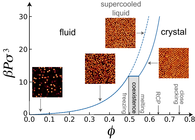
FIG. 3. Equation of state and phase diagram of hard spheres. The pressure \beta P \sigma^3 as a function of volume fraction \phi [the solid blue (dark gray) line] is approximately given by the Carnahan-Starling expression (Carnahan and Starling, 1969) for the fluid and by that of Hall (1972) for the crystal. The metastable extension of the fluid branch [the dashed blue (dark gray) line] is where slow dynamics and the hard-sphere supercooled liquids and glass transition can be found; see Sec. XII. Indicated on the x axis are the fluid and crystal phases, along with freezing volume fraction \phi_f = 0.492 , melting volume fraction \phi_m = 0.543 , and phase coexistence at pressure \beta P \sigma^3 = 11.6 ; see Sec. VII.A. Also indicated are random close packing \phi_{rcp} \approx 0.64 and crystal close packing \phi_{cp} = \pi/3\sqrt{2} = 0.740\dots . Approximate state points of the confocal microscopy images are denoted by gray arrows.
