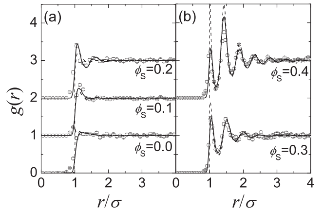
FIG. 28. Radial distribution function of large colloids in binary hard spheres at various concentrations of the smaller species for (a) low \phi_s \leq 0.25 and (b) high \phi_s > 0.25 . Monte Carlo simulation data at small colloid volume fraction \phi_s are denoted by solid lines and compared to the experimental data (circles). The dashed lines correspond to g(r) \approx \exp[-\beta u(r)] , where u(r) is the effective interaction between the large colloids consisting of the depletion interaction induced by the smaller and a residual electrostatic contribution. In addition to experimental resolution and polydispersity, MC simulations account for residual colloid charge. From Royall, Louis, and Tanaka, 2007.
