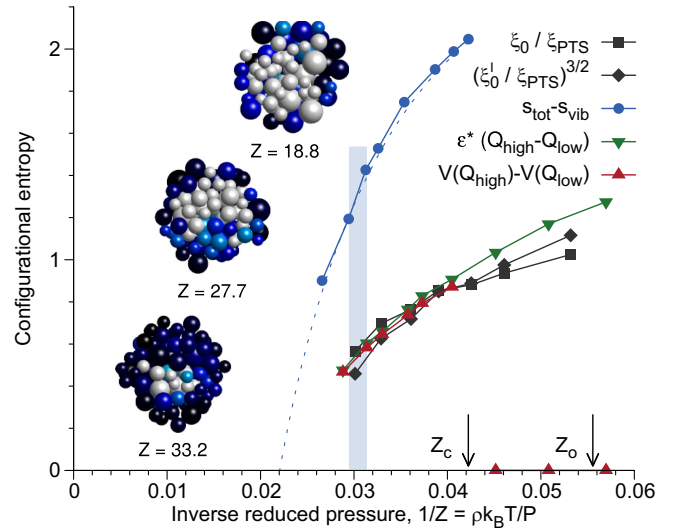
FIG. 41. Different estimators of the configurational entropy consistently extrapolate to their vanishing at a finite reduced pressure; this is congruous with the existence of a Kauzmann-type entropy crisis. Inset: depiction of the growing extent of amorphous order (dark colors) as pressure increases. From Berthier et al. , 2017.
