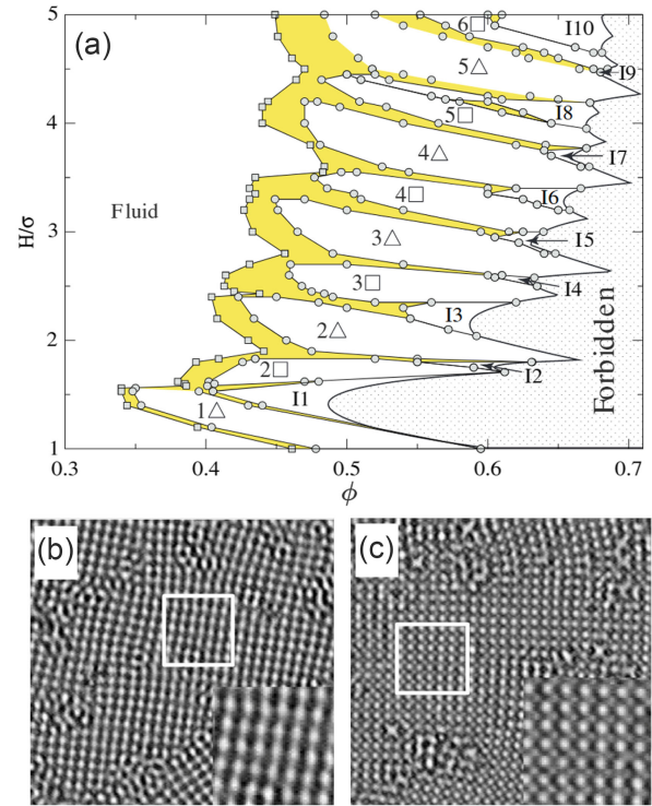
FIG. 29. (a) Equilibrium phase diagram of hard spheres confined between two parallel hard walls with plate separation H vs volume fraction representation. The white, yellow, and dotted regions indicate the stable one-phase region, the two-phase coexistence region, and the forbidden region, respectively. (a) From Fortini and Dijkstra (2006). (b),(c) Optical microscopy images of charged spheres in an aqueous system confined in a wedge geometry. Shown are both (b) a 2\Delta phase and (c) a 2\square phase. (b),(c) From Fontecha et al. , 2005.
