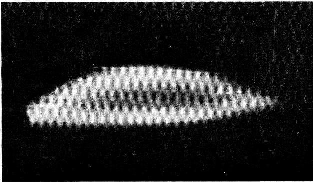
FIG. 3. Photograph of a cord discharge in deuterium with an admixture of 5% argon at high power P = 14.7 kW and high pressure p = 3.32 atm. Length of the discharge \sim 10 cm. The left edge of the discharge is blocked by the window. Oscillations of E_{01} type (1969).
