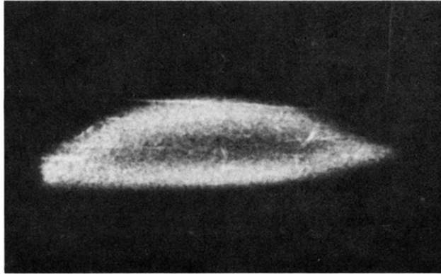
FIG. 3. Photograph of a cord discharge in deuterium with an admixture of 5% argon at high power P = 14.7 kW and high pressure p = 3.32 atm. Length of the discharge \sim 10 cm. The left edge of the discharge is blocked by the window. Oscillations of E_{01} type (1969).
