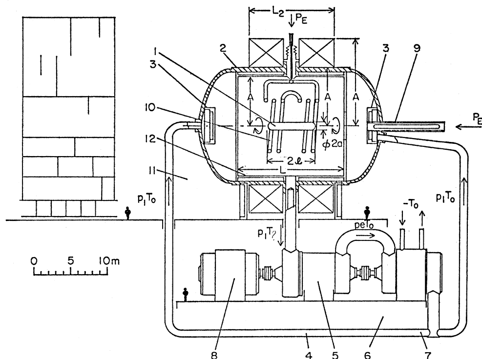
FIG. 4. Drawing of the construction of a thermonuclear reactor operating on a closed cycle. 1—cord discharge, 2—cylindrical container of the reactor, 3—inclined nozzles, 4—pipe connecting the container of the reactor with the gas turbine, 5—gas turbine, 6—isothermal compressor, 7—cooling water, 8—generator, 9—coaxial waveguide, 10—coil for the alternating magnetic field, 11—solenoid, 12—copper wall of the resonator, L —length of the resonator, L_1 —length of the solenoid, P_a —power of magnetoacoustic, P_r —high-frequency power, A —radius of the resonator, A_1 —internal radius of the winding, A_2 —external radius of the winding, 2l —length of the cord discharge, 2a —diameter of the cord discharge, h —distance between the wall of the container and the resonator.
