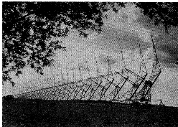
FIG. 3. Photograph of the east-west arm of the \lambda = 1.7 m instrument built in 1957, with which nearly 5000 sources were located.
