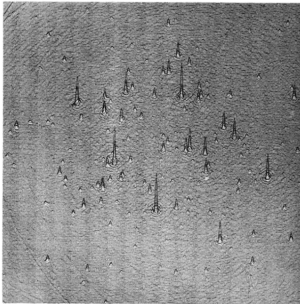
FIG. 7. Map obtained with the One-Mile telescope showing sources about 100 times fainter than had been observed before.
