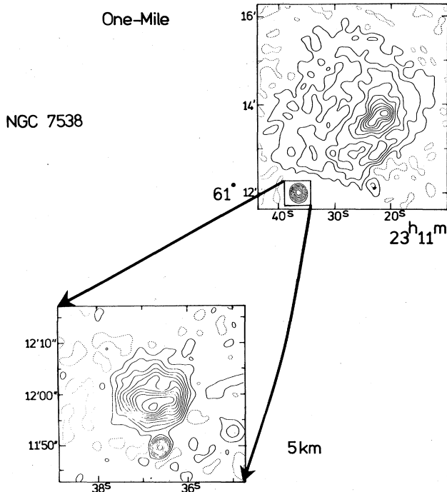
FIG. 9. The ionized hydrogen cloud NGC 7538. The upper radio map shows the large cloud associated with the optical emission, and another, compact, component to the south. This compact component is shown with greater resolution below.
