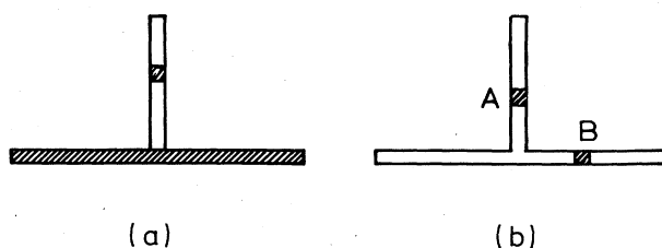
FIG. 2. (a) The arrangement used in the instrument built in 1954 by J. H. Blythe. (b) The equivalent instrument using two small elements.
