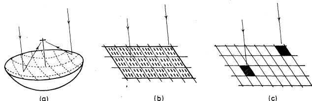
FIG. 1. The use of (a) a paraboloid, (b) an array of dipoles, or (c) the sequential sampling of the wavefront by small aerial elements to achieve a high resolving power by combining the signals from a large part of the incident wavefront.
