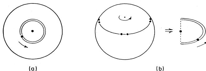
FIG. 4. (a) Two aerial elements mounted near the North Pole, observing throughout the day, are equivalent to one ring of a much larger instrument. (b) The elements may be used at other latitudes if arranged on an east-west line and used to track the chosen point for 12 h.
