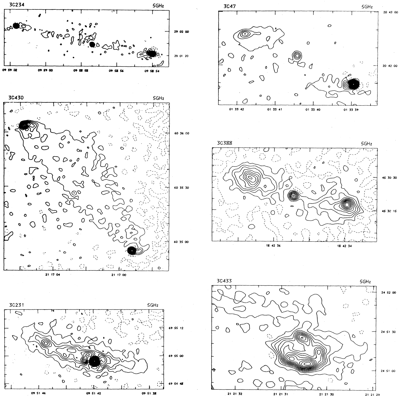
FIG. 12. Maps of six extragalactic radio sources.
