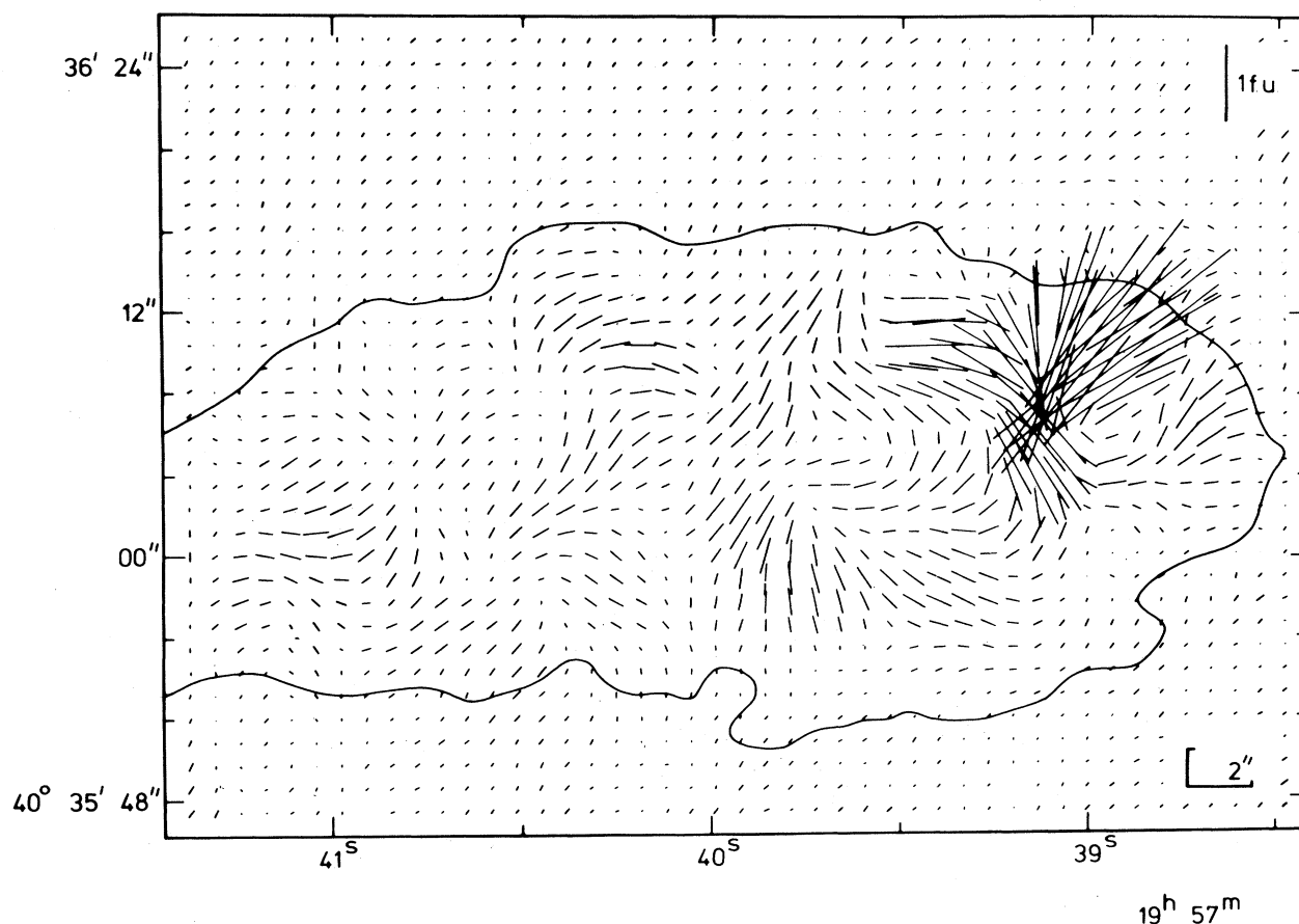
FIG. 11. The polarization of the emission from the north component of the Cygnus source, which shows the magnetic field to be turbulent on a scale \sim 10^4 light years.
