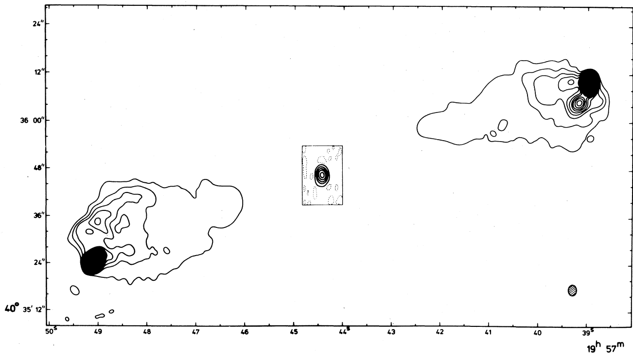
FIG. 10. The powerful radio galaxy, in the constellation of Cygnus, mapped with the 5 km telescope. The compact outer components are exceedingly bright—(31 and 41 contours). The central component—which corresponds to the nucleus of the optical galaxy—is very weak and is drawn with contours spaced at \frac{1}{5} the interval.
