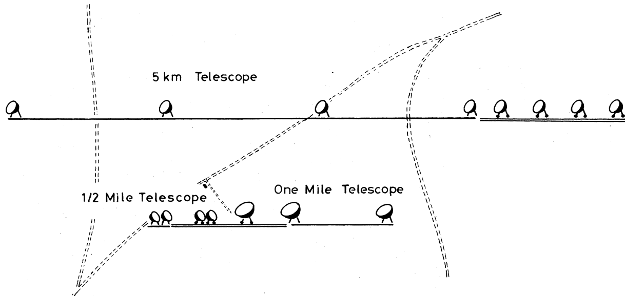
FIG. 5. Sketch map showing the arrangement of One-Mile, Half-Mile, and 5 km telescopes.
