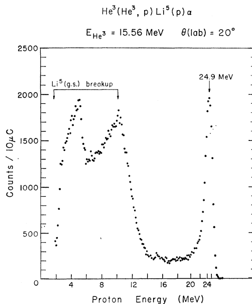
FIG. 2. Proton spectrum for a \text{He}^3 bombarding energy of 15.56 MeV and a laboratory angle of 20^\circ . See Fig. 1 and text for discussion.
