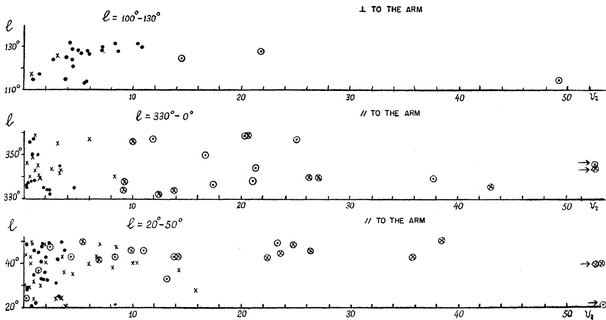
FIG. 1. Velocities from H and K lines.
