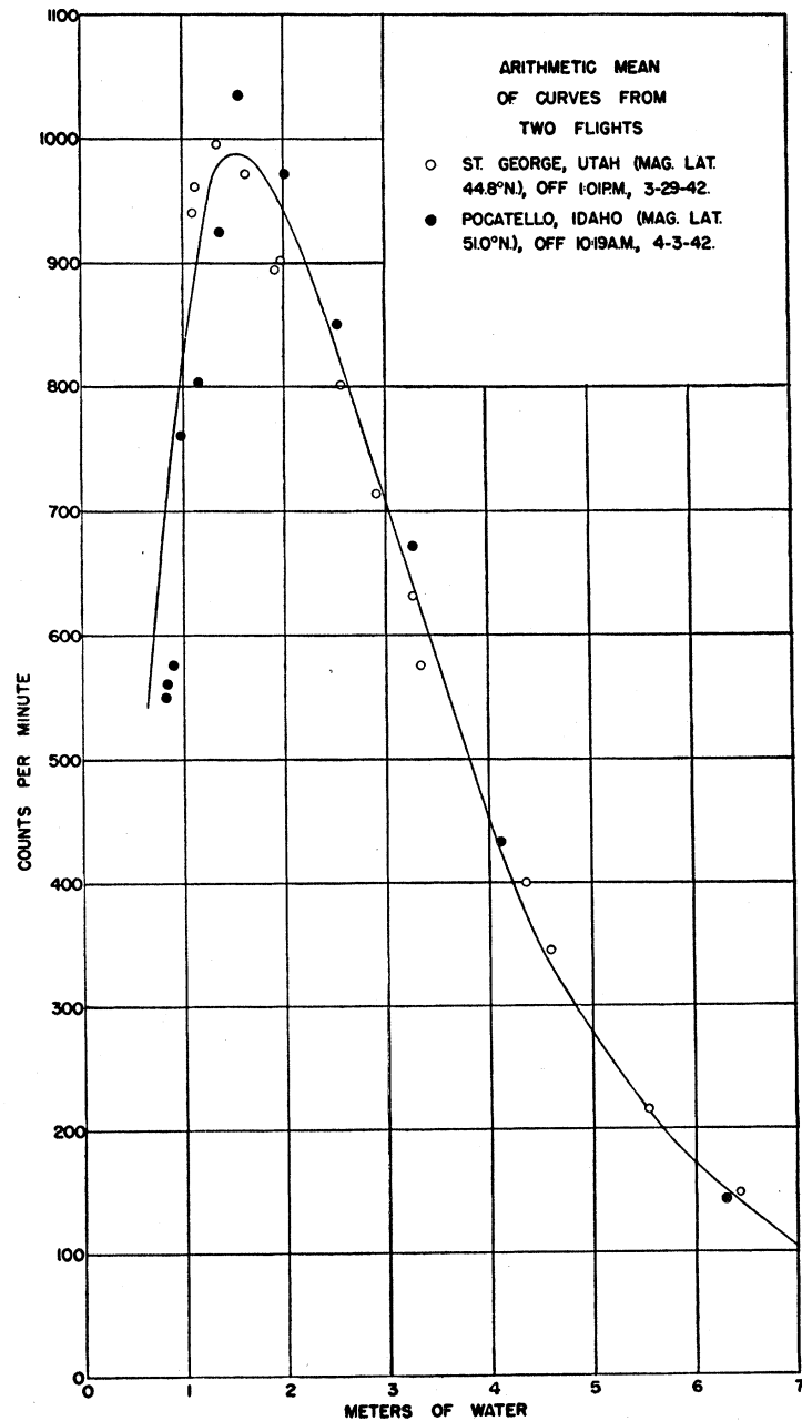
FIG. 13. Shows that there is practically no new energy entering vertically in the long latitude stretch between St. George and Pocatello, although there is clear evidence of the entrance of carbon-annihilation rays between Pasadena and St. George, Utah. Note maximum at 980 ions.
