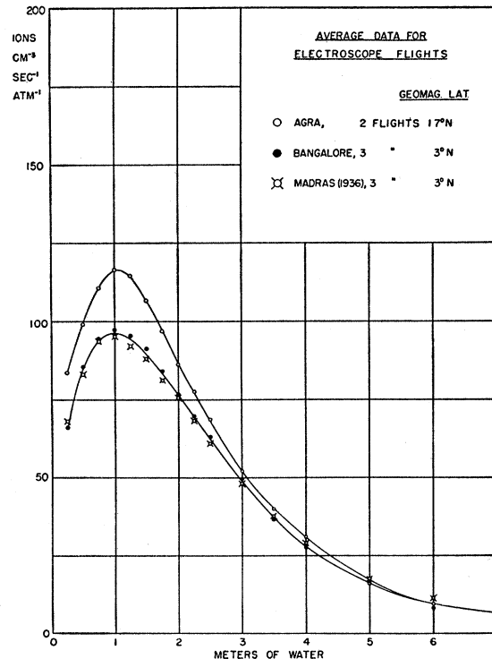
FIG. 8. Average data for electroscopes flights at magnetic latitude 17° 3' N and 3° N. Note that, though the two sets of points on the Madras-Bangalore curve, both at 3° Mag. Lat., correspond to observations taken more than three years apart, one single curve fits perfectly both series of observations. This speaks well both for the reliability of the observations and for the reproducibility of the conditions. The area under the Agra curve is here 8 percent higher than the area under the Bangalore-Madras curve, in agreement with our predictions from Fig. 6 for electroscopes readings.
