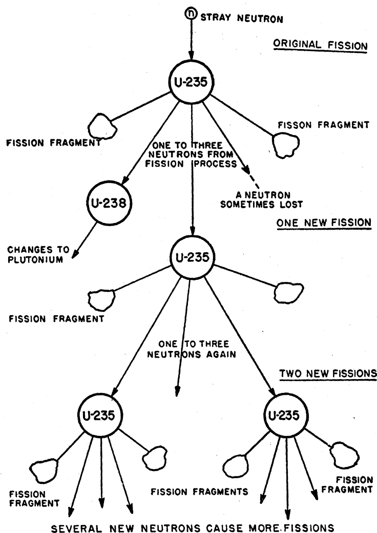
FIG. 3. Schematic diagram of chain reaction from fission, neglecting effect of neutron speed. In an explosive reaction the number of neutrons multiplies indefinitely. In a controlled reaction the number of neutrons builds up to a certain level and then remains constant.
