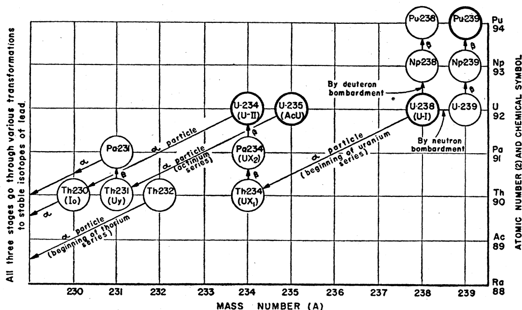
FIG. 1. The beginnings of the three natural radioactive series and the new transuranic elements, neptunium and plutonium.
