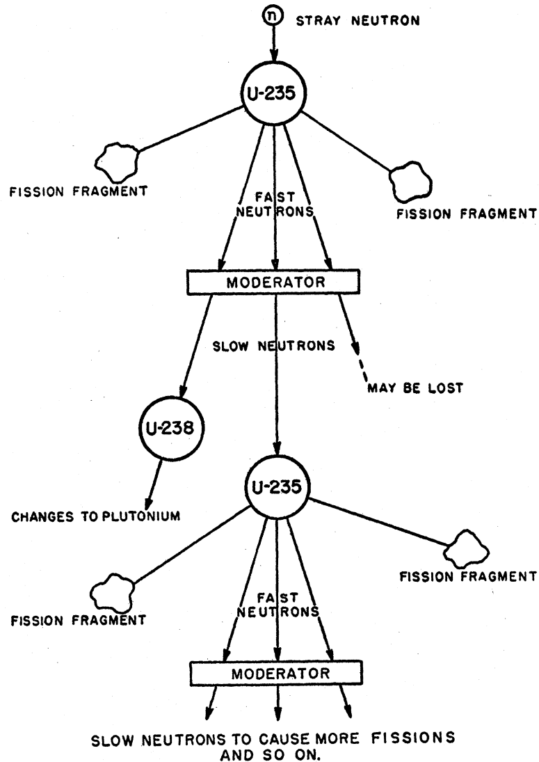
FIG. 4. Schematic diagram of fission chain reaction using a moderator to slow neutrons to speeds more likely to cause fission.
