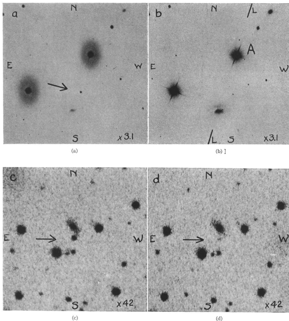
FIG. 3. (a) Shows NGC 1482 [R.A. 3^{\text{h}} 51.9^{\text{m}} , Decl. -20^{\circ} 41' (1938)] with supernova (arrow) about a month after maximum brightness m_{\text{max}} \approx 14 . The photograph, which was taken by Hubble on February 5, 1938 with the 100-inch telescope on the Mt. Wilson Observatory is of very poor quality due to poor seeing conditions. In addition imperfections of the aluminum coat of the secondary mirror caused the elliptical halos around the bright stars.
