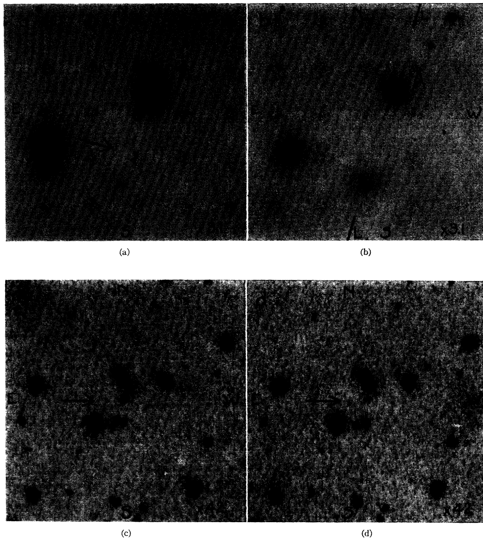
FIG. 3. (a) Shows NGC 1482 [R.A. 3^{\text{h}} 51.9^{\text{m}} , Decl. -20^{\circ} 41' (1938)] with supernova (arrow) about a month after maximum brightness m_{\text{max}} \leq 14 . The photograph, which was taken by Hubble on February 5, 1938 with the 100-inch telescope on the Mt. Wilson Observatory is of very poor quality due to poor seeing conditions. In addition imperfections of the aluminum coat of the secondary mirror caused the elliptical halos around the bright stars.
