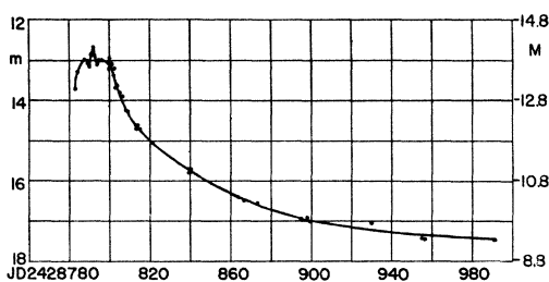
FIG. 5. Photographic light curve of supernova in NGC 1003. m and M are the apparent and the absolute magnitudes, respectively. The dates are given in Julian days. JD 2,428,780 is September 2, 1937. For a more detailed discussion of the data see W. Baade and F. Zwicky, Astrophys. J. 88 , 411 (1938).
