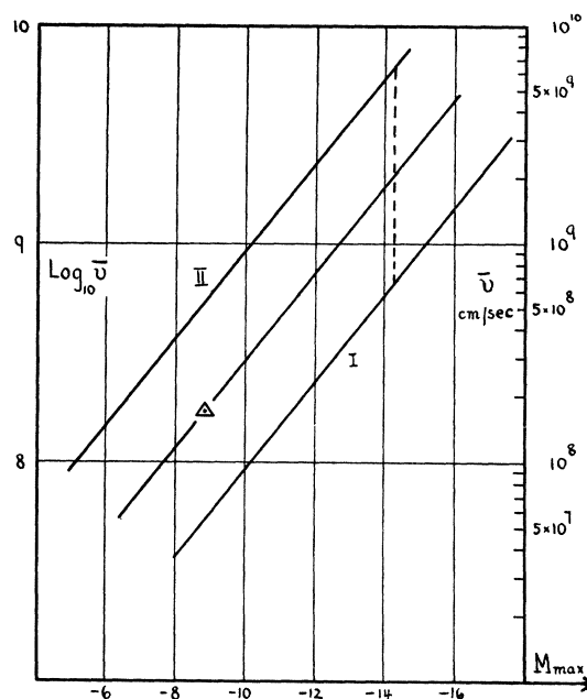
FIG. 1. Expansion-luminosity relation.
