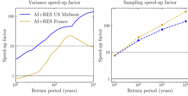
FIG. 3. Speedup factors for the AI + RES algorithm over France and the U.S. Midwest as a function of return period for reducing variance in estimated probability and producing additional samples.
