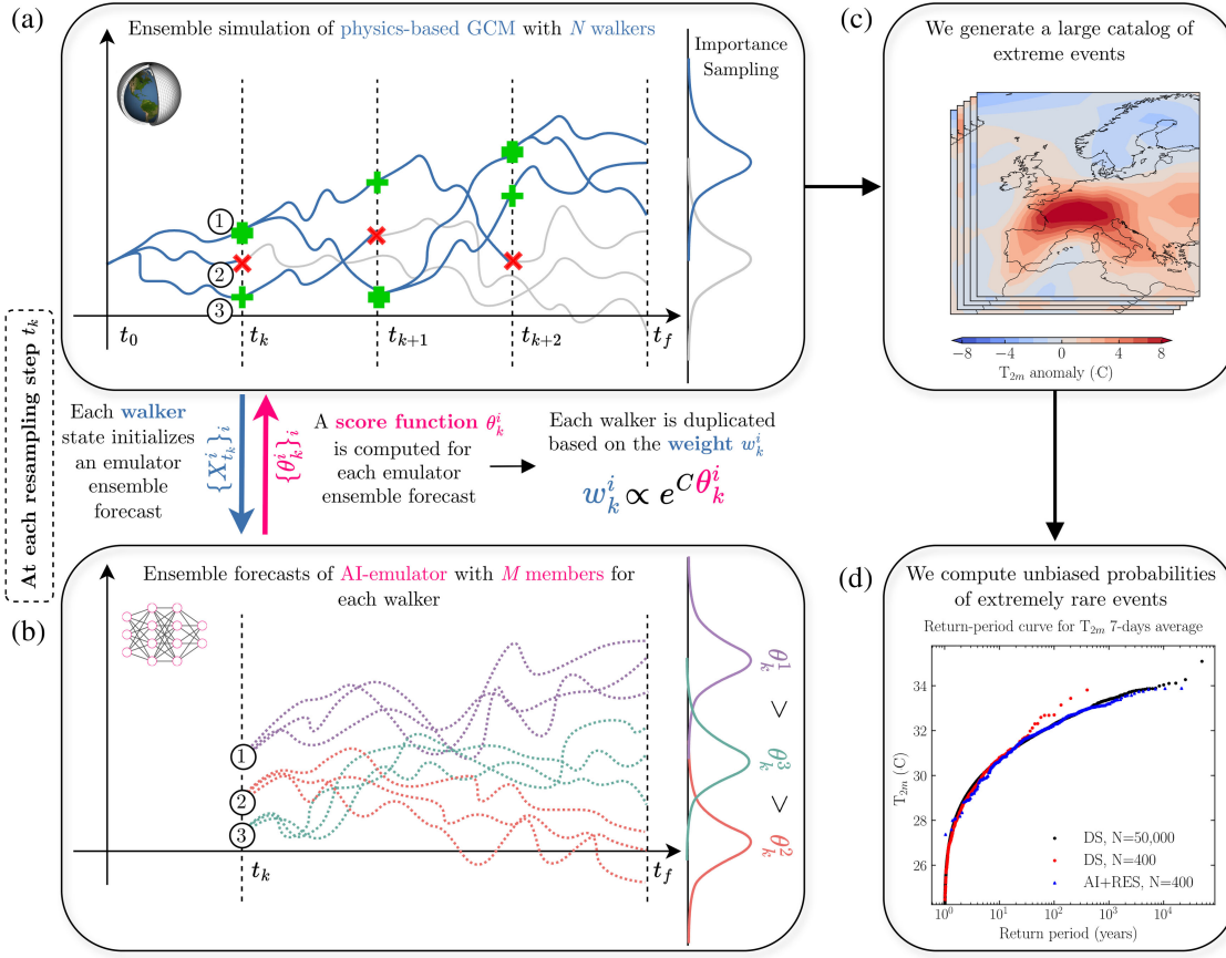
FIG. 1. Schematic of the AI + RES framework. We first train an AI weather emulator on 100 years of PlaSim GCM data and then use it to guide a rare event sampling (RES) algorithm. (a) In AI + RES, we run a PlaSim ensemble simulation with N parallel simulations, called walkers and denoted X_k^i . (b) At each resampling time t_k in the algorithm (vertical dashed lines), we perform an ensemble forecast with the AI emulator for each PlaSim walker until the target time t_f and then duplicate the more promising walkers based on these forecasts [Algorithm 1 and Eq. (C1)]. This allows us to both generate a large catalog of extreme events from physics-based simulations (c) and compute unbiased probabilities for these rare events [Eq. (B1)] (d) at a fraction of the cost of direct sampling (DS). An example of schematic (a) with actual data from an AI + RES experiment can be found in Supplemental Material (SM) Fig. S9 [46].
