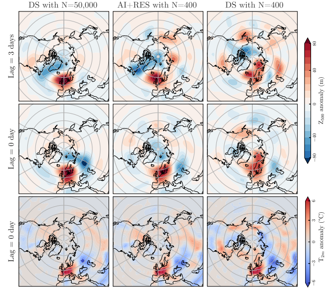
FIG. 4. Composite maps of heat waves over France with return periods exceeding 100 years. Events are defined by Eq. (A1) with L = 3 days. From top to bottom, the rows show daily mean Z_{500} anomaly composites three days before the heat wave onset, the L -day average Z_{500} anomaly composites during the heat wave, and the L -day average T_{2m} anomaly composites during the heat wave.
