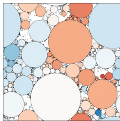
Snapshot from a simulation of ice floes (circles). The colors represent different transverse velocities. Selected for an Editors' Suggestion. [B. Shaddy, P. A. Greaney, and B. Rallabandi, Phys. Rev. Lett. 137 , 114201 (2026)]
