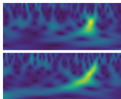
Frequency vs time image at two detectors of gravitational waves from the third observed merger of binary black holes. Selected for a Synopsis in Physics and an Editors' Suggestion. [B. P. Abbott et al. (LIGO and Virgo Collaboration), Phys. Rev. Lett. 118 , 221101 (2017)]
