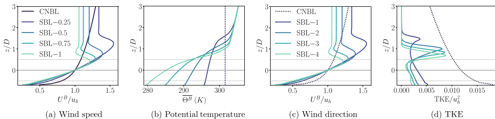
FIG. 1. Comparison of base flow quantities in the CNBL and SBLs. All quantities are averaged in time and space in the streamwise and lateral directions. The dash-dotted gray lines indicate the rotor diameter D and the solid gray line is the hub height of the rotor. Wind speed and TKE are normalized via the hub height wind speed u_h . Note that this is a subset of the vertical domain, zoomed in near the turbine.
