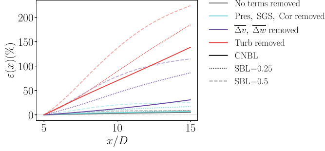
FIG. 4. Velocity deficit error in x as defined in Eq. (15) for no terms removed (—); pressure gradient, SGS, and Coriolis removed (—); \Delta v and \Delta w advection terms removed (—); and turbulence divergence removed (—). The dashed gray line shows the location of zero error.
