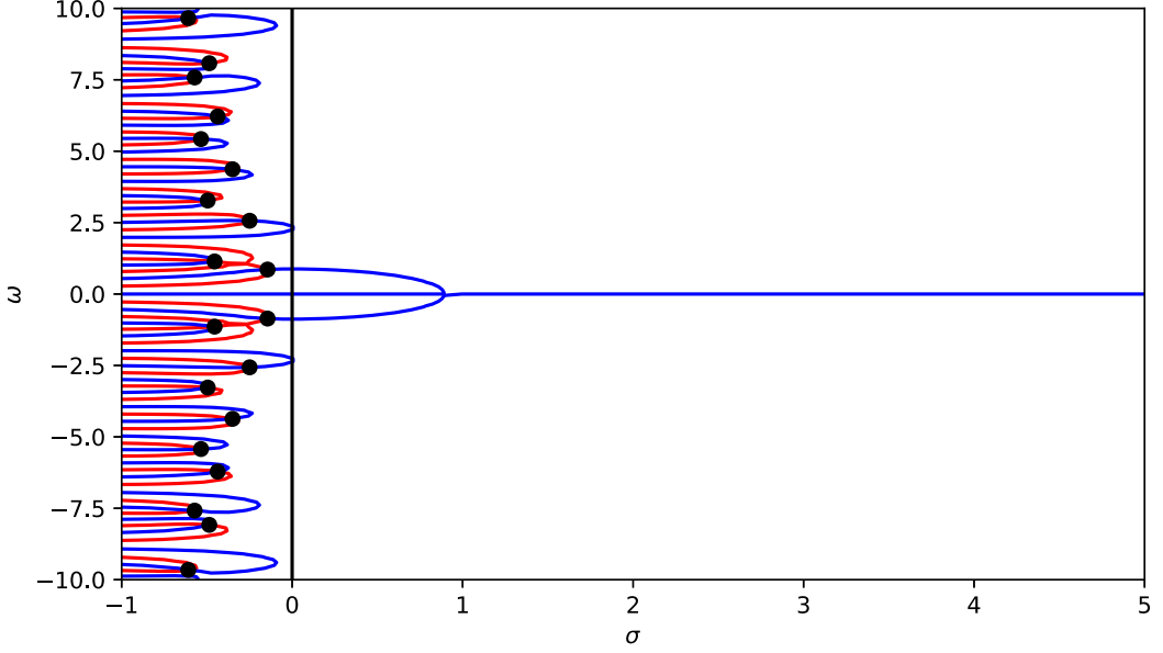
FIG. 6. Zero contours of the real (red traces) and imaginary (blue traces) parts of Eq. (13) evaluated at (V_2/V_1, V_3/V_2) \approx (1.072, 1.083) in the perturbed system of Fig. 3(b-i). Black marks indicate eigenvalues of the system.
