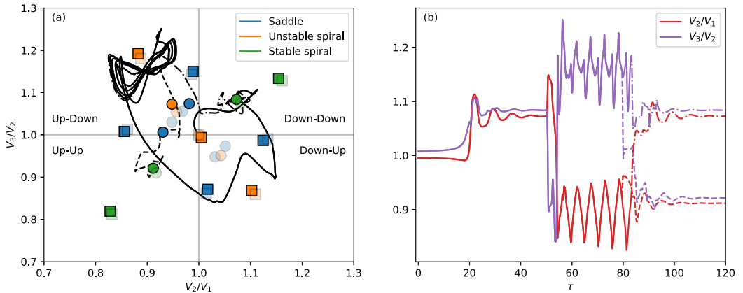
FIG. 5. (a) Stability of the equilibria supported by the symmetric networks (semitransparent marks) and perturbed networks (opaque marks) for H_D = 0.7 (circular marks) and H_D = 0.8 (square marks) with w = 11 \mu\text{m} in all cases. The traces represent the trajectories from the time domain simulations in the geometrically perturbed network shown in (b) velocity ratios are plotted as a function of normalized time \tau = t/t_0 . After ramping up, the inlet haematocrit is H_D = 0.7 for 20 < \tau < 50 , then H_D = 0.8 for 29 transits (dashed trace) or 33 transits (dot-dashed trace), before returning to H_D = 0.7 .
