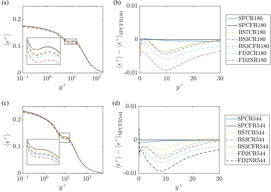
FIG. 8. Mean dissipation in (a) the \text{Re}_\tau = 180 cases and (c) the \text{Re}_\tau = 544 cases. The difference between the other cases and the SPCF cases at (b) the \text{Re}_\tau = 180 cases and (d) the \text{Re}_\tau = 544 . The solid black lines in panels (b), (d) are at 0.
