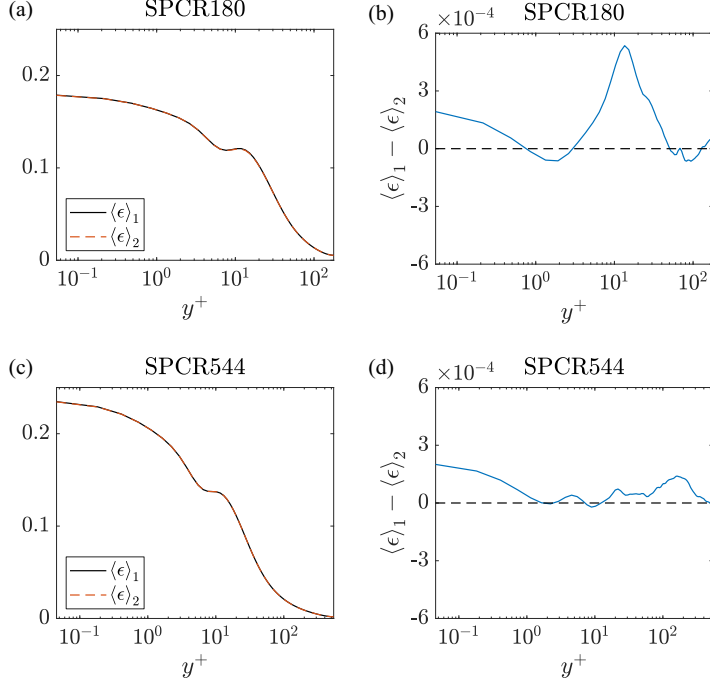
FIG. 6. Mean dissipation in (a) SPCR180 and (c) SPCR544. Here, \langle \epsilon \rangle_1 is the average over a time period of T_r , and \langle \epsilon \rangle_2 is the average over a time period of 2T_r . (b), (d) The difference between \langle \epsilon \rangle_1 and \langle \epsilon \rangle_2 .
