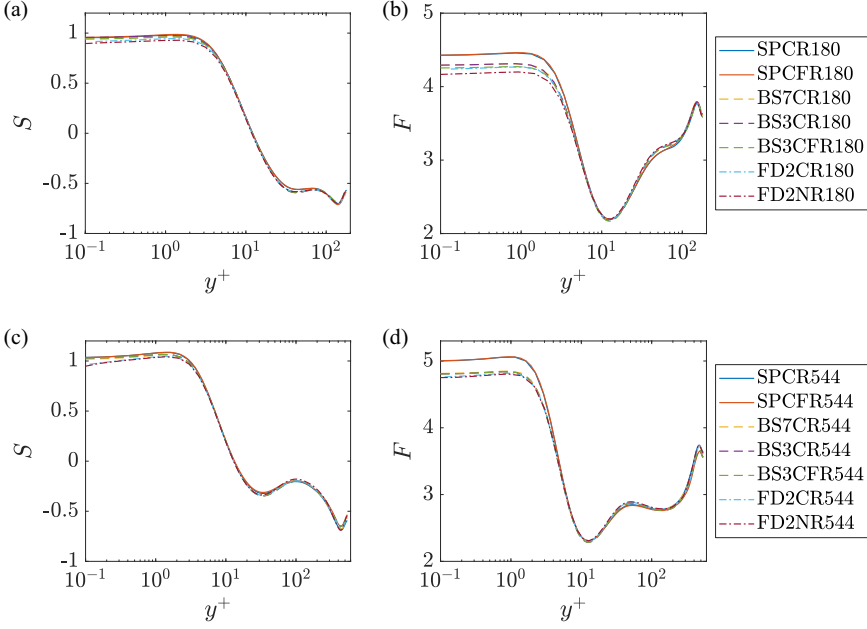
FIG. 5. Skewness of the streamwise velocity fluctuation at (a) Re_\tau = 180 and (c) Re_\tau = 544 . Flatness of the streamwise velocity fluctuation at (b) Re_\tau = 180 and (d) Re_\tau = 544 .
