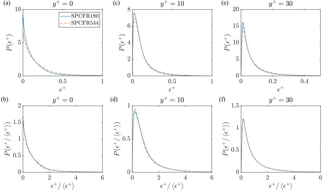
FIG. 10. PDFs of \epsilon^+ at (a) y^+ = 0 , (c) y^+ = 10 , and (e) y^+ = 30 . PDFs of \epsilon^+/\langle\epsilon^+\rangle at (b) y^+ = 0 , (d) y^+ = 10 , and (f) y^+ = 30 .
