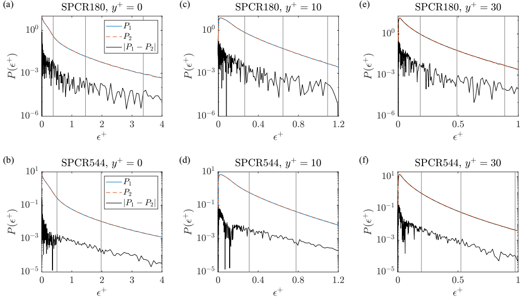
FIG. 7. Probability density function (PDF) of the instantaneous viscous dissipation at (a), (b) y^+ = 0 , (c), (d) y^+ = 10 , (e), (f) y^+ = 30 . (a), (c), (e) \text{Re}_\tau = 180 , (b), (d), (f) \text{Re}_\tau = 544 . Integrating the PDF from \epsilon^+ = 0 to the three vertical lines gives 90%, 99%, and 99.9%.
