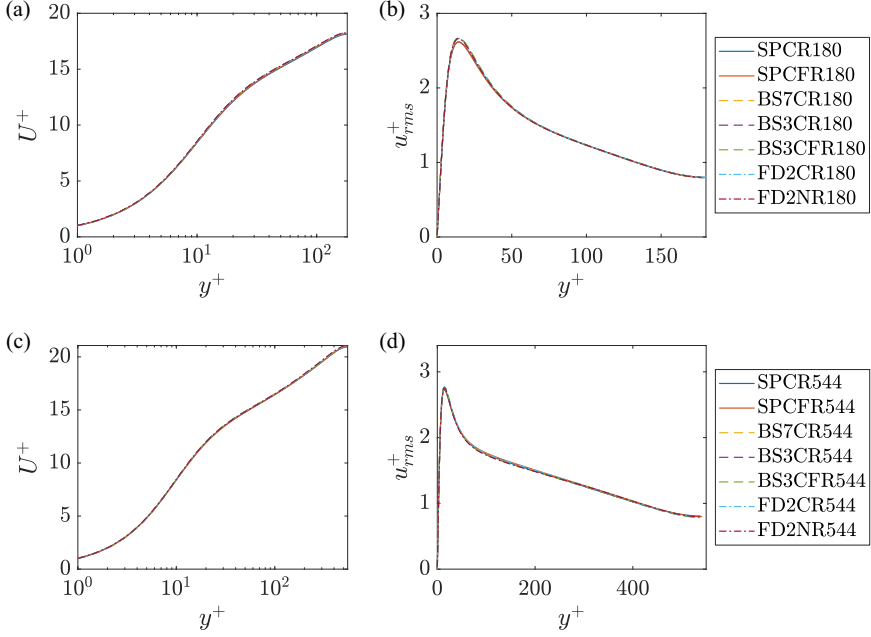
FIG. 4. Mean velocity profiles at (a) Re_\tau = 180 and (c) Re_\tau = 544 . Streamwise velocity rms at (b) Re_\tau = 180 and (d) Re_\tau = 544 .
