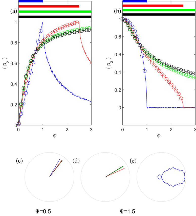
FIG. 5. Orientation in horizontal shear, \mathbf{u} = z\mathbf{i} . Horizontal (a) and vertical (b) components of orientation as a function of \Psi for different chain lengths: n = 1 ( \alpha = 0 ), blue; n = 2 ( \alpha = 0.6 ), red; n = 4 ( \alpha = 0.8824 ), green; n = 8 ( \alpha = 0.9692 ), black. The mean (solid line) is computed as the mean of the time average of each of 100 trajectories of duration T = 1000 starting from random initial orientation uniformly distributed on unit sphere, and taking the time average from t = 500 to t = 1000 , to remove the initial transient behavior. Circles indicate the stable equilibrium orientation, \theta_{\text{up}}^- , which is always globally attracting when feasible, as indicated by the thick horizontal bars. The lower plots show a polar histogram of the orientation distribution for these trajectories projected onto the x - z plane for different chain lengths for \Psi = 0.5 (left) and \Psi = 1.5 (right). (c) and (d) are for all trajectories, whereas (e) removes the data points close to the equilibrium orientation to display the distribution of orbiting trajectories.
