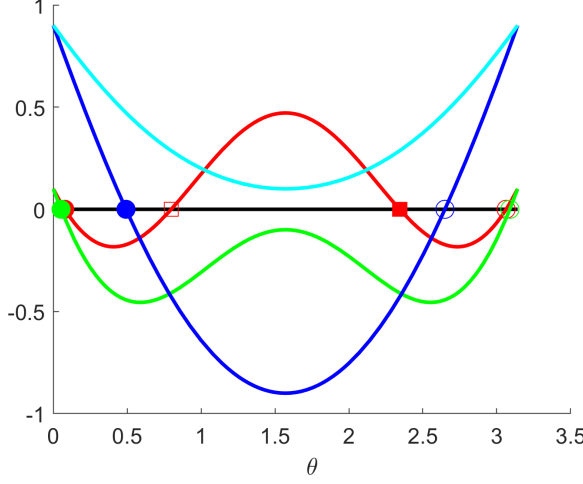
FIG. 2. Function G(\theta) for \alpha = 0.9, \sigma = 0.7 (red online, four roots, three stationary points), \alpha = 0.9, \sigma = 0.5 (green online, two roots, three stationary points), \alpha = 0.1, \sigma = 0.5 (blue online, two roots, one stationary point), \alpha = 0.1, \sigma = 1 (cyan online, zero roots, 1 stationary point). Squares are solutions \theta^+ and circles \theta^- . Filled (empty) symbols indicate (un)stable to small perturbations in \theta .
