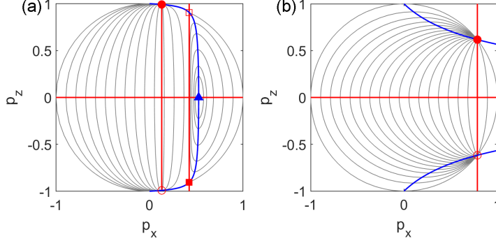
FIG. 3. Phase portrait for horizontal and vertical components of \mathbf{p} with \alpha = 0.9 and \sigma = 1 . Red lines indicate the nullclines \dot{p}_x = 0 and blue line is nullcline \dot{p}_z = 0 . As in Fig. 2, squares are E1 equilibria \theta^+ and circles \theta^- . Filled (empty) symbols indicate (un)stable to small perturbations in \theta . The E2 equilibrium is indicated by filled blue triangle. (a) Vertical shear, \mathbf{u} = -x\mathbf{k} , (b) horizontal shear, \mathbf{u} = z\mathbf{i} .
