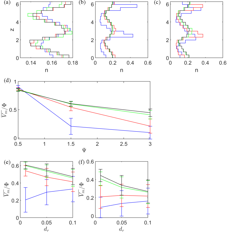
FIG. 8. Swimmers in horizontal Kolmogorov flow with addition of rotational diffusion. (a)–(c) Histogram of vertical position as Fig. 7 but with rotational diffusion d_r = 0.01 . The average vertical speed, \overline{V}_m , calculated as in Fig. 7 is plotted as (d) a function of \Psi for fixed d_r = 0.01 and as a function of d_r for fixed (e) \Psi = 1.5 and (f) \Psi = 3 .
