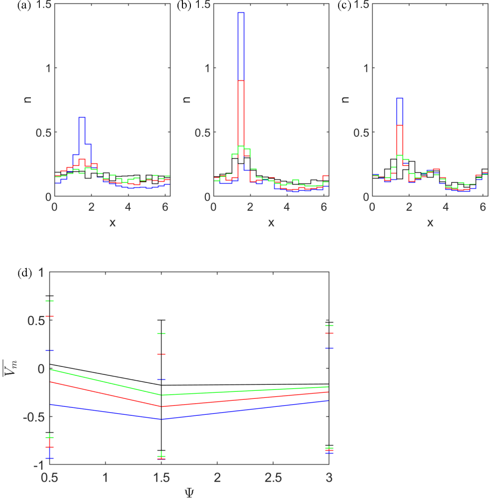
FIG. 6. Swimmers in vertical Kolmogorov flow. (a)–(c) Histogram of horizontal position [probability distribution, n(x) ], modulo 2\pi , over a trajectory for N = 1000 particles of duration T = 50 with \Phi = 0.1 , \Psi = 0.5 (a), 1.5 (b), 3 (c) for different chain lengths: n = 1 ( \alpha = 0 ), blue; n = 2 ( \alpha = 0.6 ), red; n = 4 ( \alpha = 0.8824 ), green; n = 8 ( \alpha = 0.9692 ), black. Particle initial positions, x and z , are randomly sampled from U(0, 2\pi) , and initial orientation is randomly sampled from unit sphere. The histogram is normalized as a probability density function. (d) The average vertical speed, \overline{V}_m , calculated as average vertical displacement of trajectory divided by duration, T , is plotted against \Psi for different chain lengths. Error bars indicate standard deviation.
