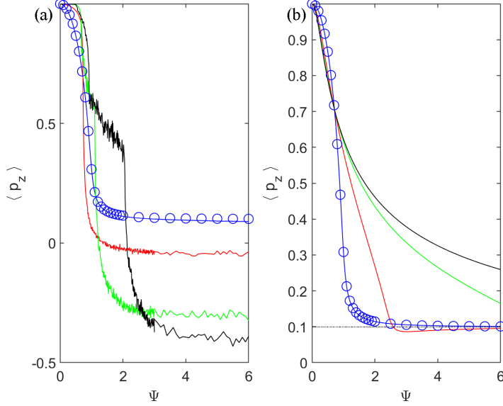
FIG. 10. Vertical component of orientation with small component of vertical vorticity, \mathbf{u} = -\epsilon\mathbf{y}\mathbf{i} , for \epsilon = 0.1 , as a function of \Psi for different chain lengths: n = 1 ( \alpha = 0 ), blue; n = 2 ( \alpha = 0.6 ), red; n = 4 ( \alpha = 0.8824 ), green; n = 8 ( \alpha = 0.9692 ), black. (a) Modification of vertical shear \mathbf{u} = -x\mathbf{k} , with the mean (solid line) computed as the mean of the time-average of each of 1000 trajectories of duration T = 1000 starting from random initial orientation uniformly distributed on unit sphere. Circles indicate the stable equilibrium orientation determined analytically for spheres, \alpha = 0 . (b) Modification of horizontal shear, \mathbf{u} = z\mathbf{i} . The solid lines are the equilibrium orientation attained by cells (note that for spheres this is the same for both the left and right panels). The large \Psi equilibrium orientation, p_z = \cos \theta = \epsilon / (\sqrt{\epsilon^2 + 1}) \approx 0.995 , which is independent of \Psi and \alpha , is indicated by dotted black line.
