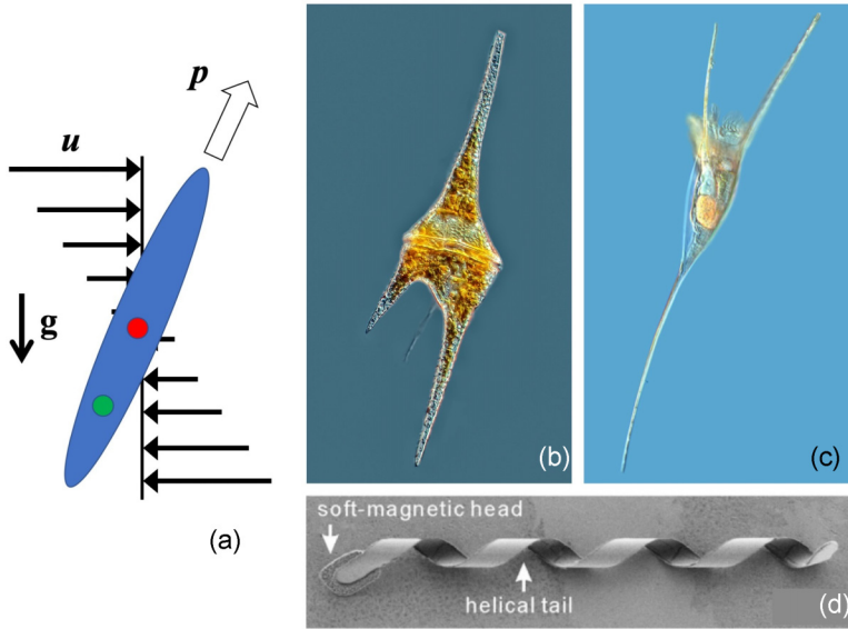
FIG. 1. Both motile planktonic organisms and engineered microswimmers can have highly elongated morphologies. (a) We idealize elongated swimmers as a prolate spheroid with aspect ratio n , whose center of mass (green circle) is separated from their center of buoyancy (red circle). This gives rise to a stabilizing torque which tends to orient their swimming direction, \mathbf{p} , in a direction parallel to gravity, \mathbf{g} . However, flow (black arrows) also exerts a viscous torque that reorients swimming in other directions. (b), (c) The toxic marine phytoplankton Ceratium furca and rotifer Kellicottia longispina both perform diel vertical migrations and possess long spines that dramatically increase their effective aspect ratio. Ceratium furca is approximately 100\ \mu\text{m} long, while Kellicottia longispina is approximately 500\ \mu\text{m} long. (d) An engineered microswimmer, inspired by bacteria, has a magnetic head that can be actuated to drive rotation about its long axis for propulsion, as well to actively guide steering. This microswimmer is approximately 50\ \mu\text{m} in length. Panel (b) was provided by Rogelio Moreno Gill [12], panel (c) was kindly provided by Antonio Guillén (Proyecto Agua), and panel (d) was reprinted from [13], with the permission of AIP Publishing.
