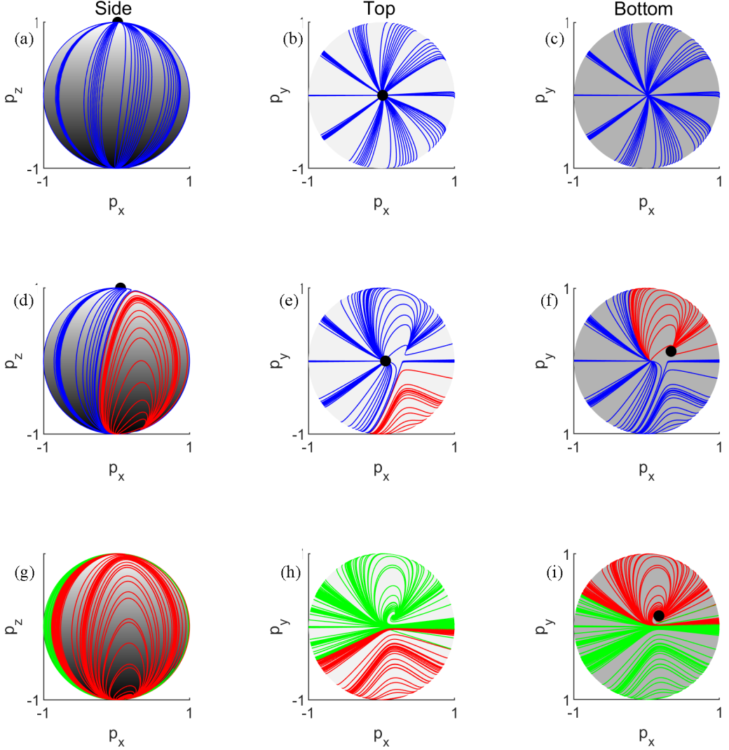
FIG. 9. Phase portrait of \mathbf{p} with n = 8(\alpha = 0.9692) for vertical shear and an additional small component of vertical vorticity \mathbf{u} = -x\mathbf{k} - \epsilon y\mathbf{i} , for \epsilon = 0.1 , as a function of \Psi : (a)–(c) \Psi = 0.5 , (d)–(f) \Psi = 1.5 , (g)–(i) \Psi = 3 . Blue (red) lines indicate trajectories which attain an upward (downward) equilibrium orientation and green lines indicate trajectories which do not attain an equilibrium. Black dots indicate the equilibrium orientation.
