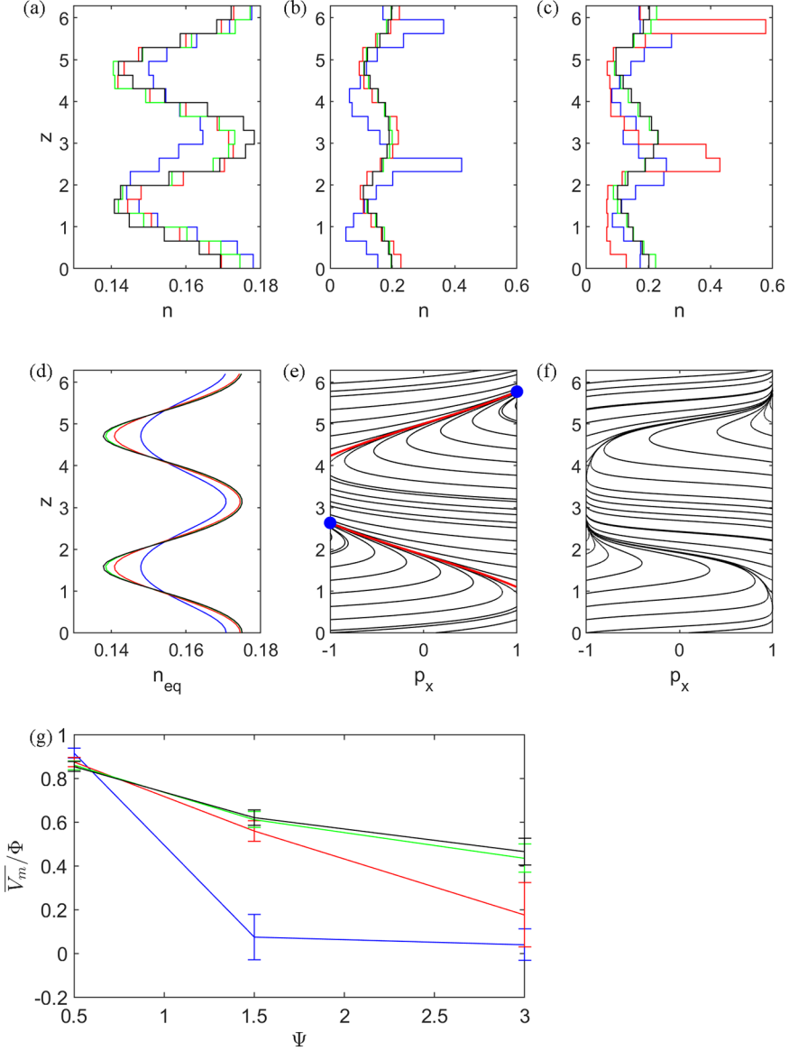
FIG. 7. Swimmers in horizontal Kolmogorov flow. (a)–(c) Histogram of vertical position (probability distribution, n(z) ), modulo 2\pi , over a trajectory for N = 1000 particles of duration T = 50 with \Phi = 0.1 , \Psi = 0.5 (a), 1.5 (b), 3 (c) for different chain lengths: n = 1 ( \alpha = 0 ), blue; n = 2 ( \alpha = 0.6 ), red; n = 4 ( \alpha = 0.8824 ), green; n = 8 ( \alpha = 0.9692 ), black. Particle initial positions, x and z , are randomly sampled from U(0, 2\pi) , and initial orientation is randomly sampled from unit sphere. The histogram is normalized as a probability density function. (d) The equilibrium distribution, computed as inversely proportional to the average swimming velocity, p_z , for \Psi = 0.5 . (e), (f) Phase portrait in p_x - z space for (e) n = 1 ( \alpha = 0 ), \Psi = 1.5 and (f) n = 2 ( \alpha = 0.6 ), \Psi = 3 , indicating how swimmers move upward and are trapped when they encounter sufficient shear to generate tumbling. Red lines indicate attracting manifold [Eq. (40)], blue circles the transition to tumbling (equation 41). (g) The average vertical speed, \bar{V}_m , calculated as average vertical displacement of trajectory divided by duration, T , normalised by swimming speed, \Phi , is plotted against \Psi for different chain lengths. Error bars indicate standard deviation.
