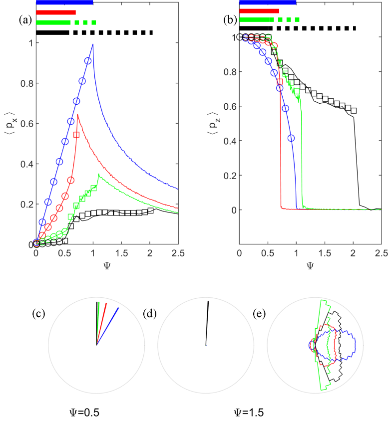
FIG. 4. Orientation in vertical shear, \mathbf{u} = -x\mathbf{k} . Horizontal (a) and vertical (b) components of orientation as a function of \Psi for different chain lengths: n = 1 ( \alpha = 0 ), blue; n = 2 ( \alpha = 0.6 ), red; n = 4 ( \alpha = 0.8824 ), green; n = 8 ( \alpha = 0.9692 ), black. The mean (solid line) is computed as the mean of the time average of each of 1000 trajectories of duration T = 1000 starting from random initial orientation uniformly distributed on unit sphere. The thick horizontal bars indicate the range where there exists a stable and globally attracting equilibrium, and circles indicate the stable equilibrium orientation, \theta_{\text{up}}^- . The horizontal dashed lines indicate the range for which the stable equilibrium is not globally attracting, and squares indicate the expected average orientation for this range of \Psi , see Eqs. (32) and (33). The lower plots show a polar histogram of the orientation distribution for these trajectories projected onto the x - z plane for different chain lengths for \Psi = 0.5 (left) and \Psi = 1.5 (right). (c) and (d) are for all trajectories, whereas (e) removes the data points close to the equilibrium orientation to display the distribution of orbiting trajectories.
