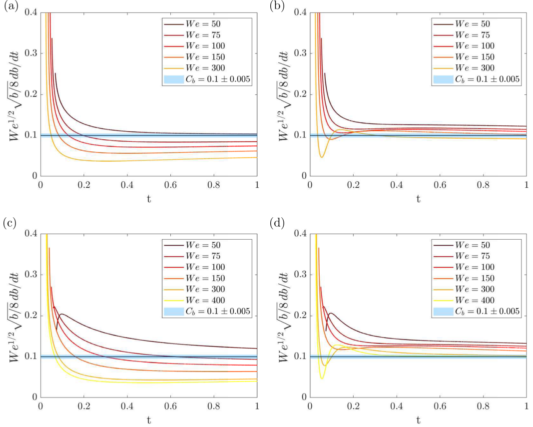
FIG. 8. The ratio C_b = We^{1/2} \sqrt{b/8} db/dt defined in Eq. (2) is calculated solving the system of Eqs. (3) and (4) subjected to the initial conditions given in Eqs. (8) and (10) for different values of We and two values of \lambda and Oh : (a) Oh = 3 \times 10^{-3} and \lambda = 0 , (b) Oh = 3 \times 10^{-3} and \lambda = 1 , (c) Oh = 9 \times 10^{-3} and \lambda = 0 and (d) Oh = 9 \times 10^{-3} and \lambda = 1 . The critical Weber number for splashing, We^* , is calculated as the minimum value of We for which the curves cross the horizontal line C_b = We^{1/2} \sqrt{b/8} db/dt = 0.1 \pm 0.005 . Notice that We^* increases with Oh and \lambda , namely, as the shear stress with the substrate increases.
