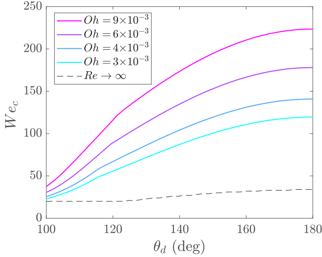
FIG. 11. Values of the critical Weber numbers as a function of the advancing contact angle \theta_d obtained solving Eqs. (3), (4), (8), and (10) for the case in which the term -2We^{-1} in Eq. (3) is replaced by -(1 - \cos \theta_d) We^{-1} with \lambda = 1 and different values of Oh .
