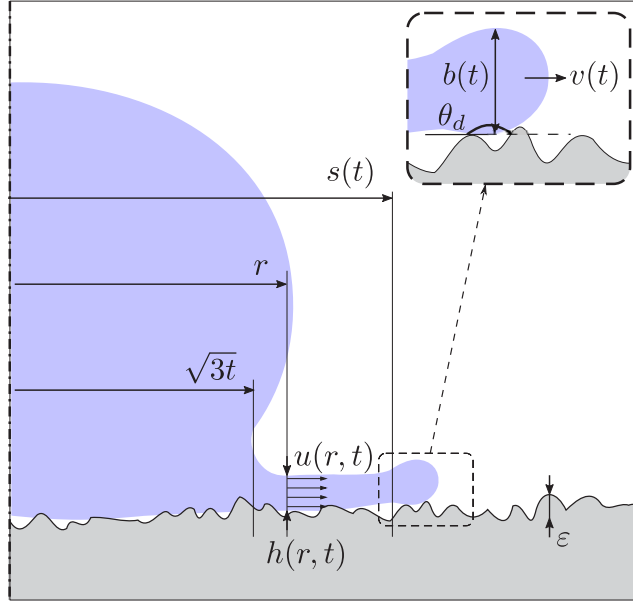
FIG. 7. Sketch illustrating the definitions of the different dimensionless variables used in the model, s(t) , v(t) , b(t) , u(r, t) , and h(r, t) [34], which are defined using as characteristic values of length, time and pressure, R , R/V , and \rho V^2 , with R , V , and \rho denoting, respectively, the drop radius, the impact velocity and the liquid density. The value for the dynamic advancing contact angle is taken here as \theta_d = \pi .
