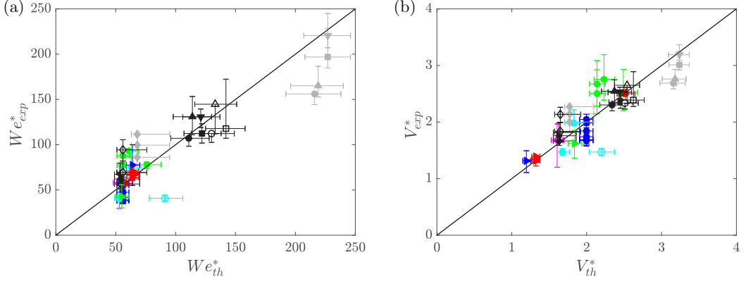
FIG. 10. Comparison between the experimental values of (a) the critical Weber number and (b) the critical velocity for splashing given or deduced from Tables III and IV and the corresponding values calculated solving the system of Eqs. (3) and (4) complemented with Eq. (7) for \lambda(\epsilon) using \epsilon_0 = 0.02 , see also Figs. 8 and 9. Notice that \lambda = 0 for the case of drops impacting in the Leidenfrost regime and also for the superhydrophobic substrates created by depositing one (SH2), two (SH1) or three (SH0) layers of NeverWet over a glass substrate, see Tables II and III.
