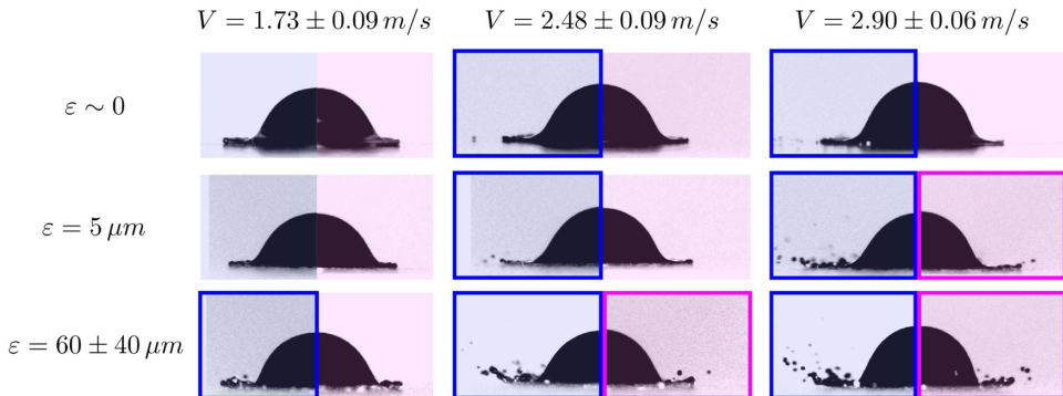
FIG. 3. Images showing the impact with different velocities of drops of radius R = 1.44 \pm 0.05 mm of either water (blue background) or of a 30% water-sugar mixture with a viscosity of three times that of water (pink background) over three different types of superhydrophobic substrates with increasing roughnesses. The blue or pink boxes are used to highlight the occurrence of splashing. The value of the advancing contact angle is the same, \theta_{\text{adv}} \approx 158^\circ , for the cases of Teflon \varepsilon \approx 0 \mu\text{m} , and for the case of glass covered with three layers of NeverWet , \varepsilon = 60 \pm 40 \mu\text{m} , see Table II. The images are represented at t = T V/R = 0.8 \pm 0.08 , with T the instant of time after the drop first touches the substrate.
