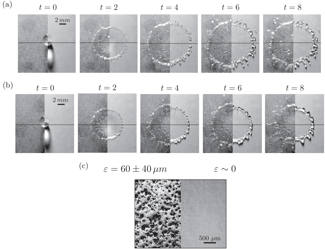
FIG. 4. Spreading of a drop of radius R = 1.45 \pm 0.03 mm of either water (a) or a 30% sugar-water mixture (b) impacting with a velocity V = 2.89 \pm 0.05 \text{ms}^{-1} over two different types of superhydrophobic substrates with different rugosities. (c) At the left of each of the images in panels (a) and (b), drops impact against glass coated with several layers of NeverWet , ( \varepsilon = 60 \pm 40 \mu\text{m} ) and, at the right, drops impact over PTFE (Teflon, \varepsilon \approx 0 \mu\text{m} ). For both values of the liquid viscosity, the maximum expansion of the drop is attained for the case of the superhydrophobic substrate with the larger value of \varepsilon (left images). Here, t = TV/R , with T the instant of time after the drop first touches the substrate.
