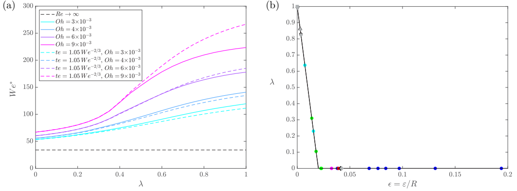
FIG. 9. (a) The values of We^* calculated following the procedure illustrated in Fig. 8 using either Eq. (8) (continuous lines) or the approximate value in the low- Oh limit in Ref. [14] t_e = 1.05 We^{-2/3} (dashed lines), are represented as a function of \lambda for four different values of Oh . The value of We^* corresponding to the potential flow case, Re \rightarrow \infty , is indicated with a horizontal black dashed line. The results in this figure clearly show that We^* increases with Oh and \lambda , namely, as the shear stress with the substrate increases. (b) The friction factor \lambda is calculated as a function of the values of \epsilon given in Tables III and IV by means of Eq. (7) using \epsilon_0 = 0.02 (black continuous line).
