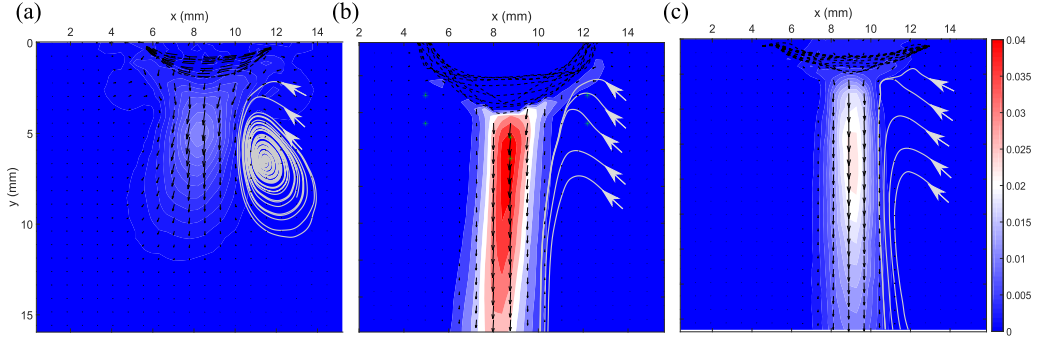
FIG. 6. Mean velocity contour associated with an oscillating bulged-out interface (a) 20 Hz, (b) 30 Hz, and (c) 50 Hz. The 30-Hz case has the fastest streaming velocity. The streamlines (gray arrow curves) demonstrate the different streaming patterns and entrainment processes.
