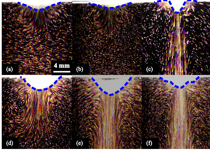
FIG. 5. Flow pathlines (in 1 s) showing the steady streaming motions induced by the different dynamic oscillations, with the same panel labeling as Fig. 3. The outmost boundary of the oscillating interface is highlighted by the blue dashed lines. The observed streaming patterns include small-scale streaming vortex and large-scale streaming jet as well as a transitional streaming vortex in between.
