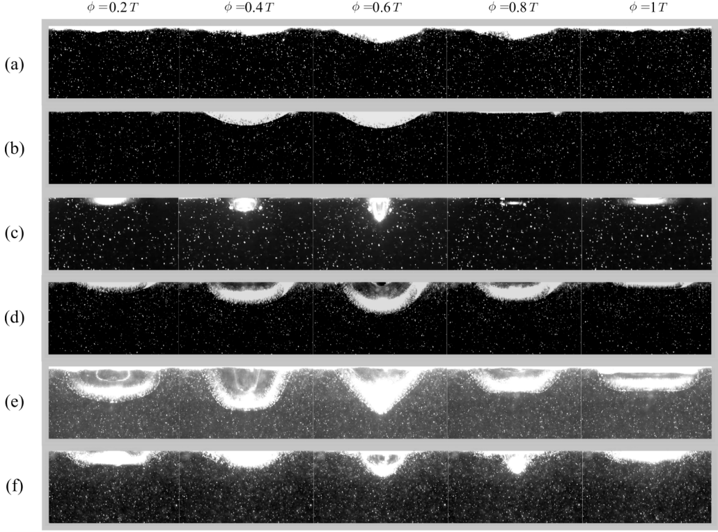
FIG. 3. Snapshots of the dynamic free-slip surface at five equally spaced phases ( \phi ) over the period of one oscillation cycle ( T ). The static interface was either flat [(a), (b), and (c)] or bulged-out [(d), (e), and (f)]. The modulation frequency was 20 Hz [(a) and (d)], 30 Hz [(b) and (e)], and 50 Hz [(c) and (f)].
