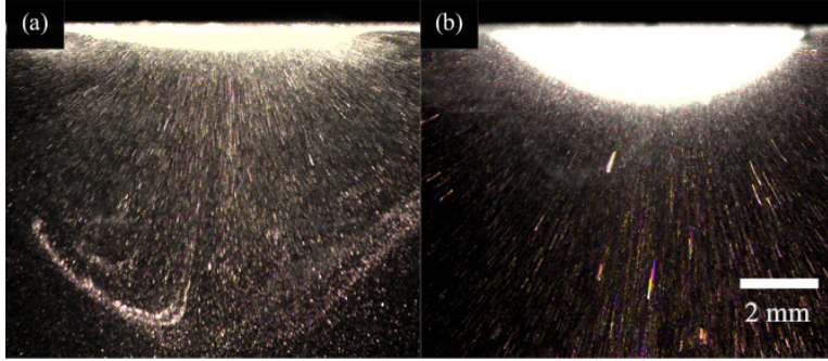
FIG. 13. Flow pathlines over the period of three oscillation cycles for a 50-Hz oscillating no-slip elastic membrane under (a) low-power modulation and (b) high-power modulation.
