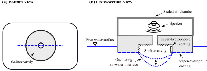
FIG. 1. Schematic drawing of an oscillating free-slip air-water interface with a fixed contact line boundary condition. The contact line of the air-water interface is fixed at the edge of a surface cavity by applying superhydrophobic and superhydrophilic material coating in different regions of the surface cavity. The static and dynamic curvature of the interface is controlled by regulating the static and dynamic pressure inside the surface cavity. The dashed line in panel (b) marks the location of the experiment measurement plane.
