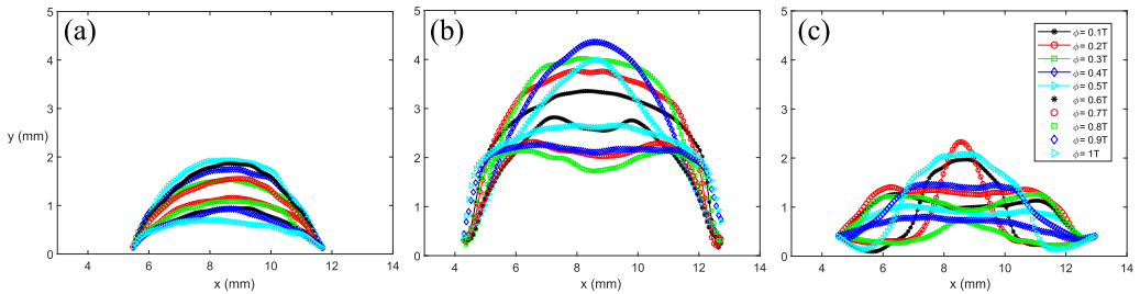
FIG. 4. The phase-varying profiles of a bulged-out interface oscillating at (a) 20 Hz, (b) 30 Hz, and (c) 50 Hz. The dynamic oscillations resemble the different modes of the Bessel function. The oscillation-amplitude peaks at 30 Hz among the selected frequencies.
