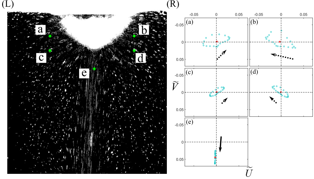
FIG. 12. Panel (L): Flow pathlines near a 30-Hz oscillating bulged-out interface over the period one oscillation cycle. In the circumferential entrainment regions [e.g., labeled as (a)–(d)], the flow pathlines are closed-loop circles. In the jetting region, the flow pathlines are vertical straight lines. Panel (R): Phase-plane plots for the phase-averaged velocity vector (\tilde{u}, \tilde{v}) at locations labeled as (a)–(e) in panel (L). Blue circles: (\tilde{u}, \tilde{v}) ; red dots: (\bar{u}, \bar{v}) ; arrows: visual representation of the time-averaged velocity vector (\bar{u}, \bar{v}) . The dashed arrows in panels (a)–(d) are amplified 10 times, whereas the solid arrow in panel (e) is not amplified.
