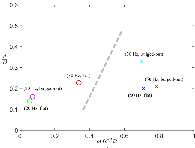
FIG. 7. Phase diagram of the different streaming patterns based on the nondimensional amplitude ( R = \frac{d}{D} ) and the Weber number ( We = \frac{\rho(f d)^2 D}{\gamma} ). Circle: streaming vortex; cross: streaming jet. Gray dashed line: an approximate boundary of streaming pattern change.
