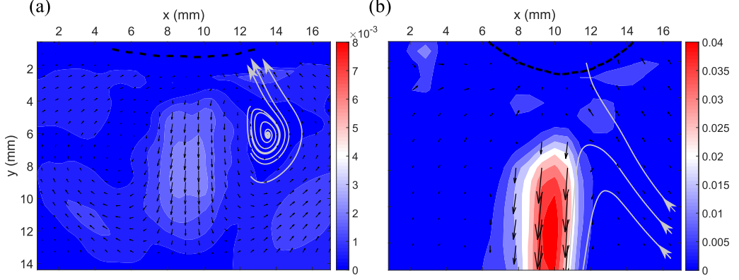
FIG. 14. Time-averaged velocity contour for the 50-Hz oscillating no-slip elastic membrane under (a) low-power modulation and (b) high-power modulation. Note that the contour scales are different in the two panels.
