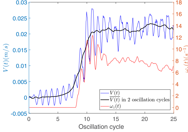
FIG. 9. Synchronized time series of the vertical velocity [V(t)] and the transverse vorticity [\omega_z(t)] measured at the (x, y) location of (7.7 \text{ mm}, 10 \text{ mm}) , which is along the symmetry axis and far away from the oscillating interface. The streaming jet is created and sustained because the accumulated \overline{\omega_z} induces a steady vertical velocity following the Biot-Savart law.
