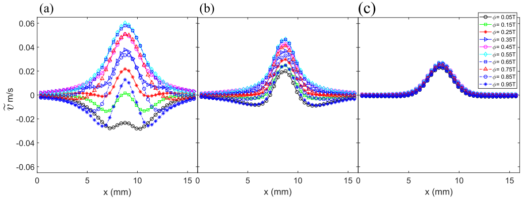
FIG. 11. Phase-averaged vertical velocity \tilde{v} measured at (a) y = 5 mm, (b) y = 13 mm, and (c) y = 20 mm. The near-field velocity exhibits features of a steep traveling wave whereas the far-field velocity reflects a steady current.
