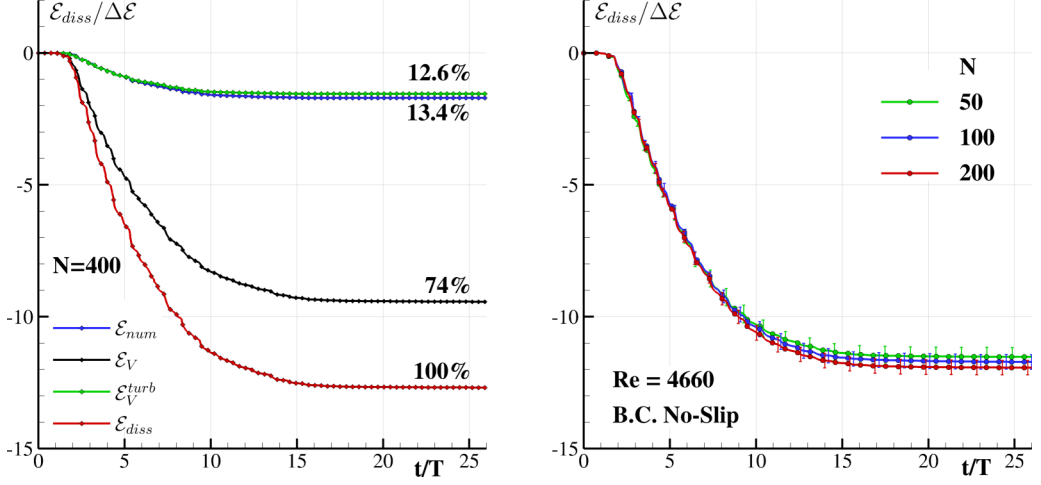
FIG. 11. Left: Time history of the energy components defined in Sec. III: resolved viscous dissipation \mathcal{E}_V , modeled turbulent viscous dissipation \mathcal{E}_V^{turb} , numerical diffusion \mathcal{E}_N , total energy dissipation \mathcal{E}_{diss} for the case N = 400 and Re = 4660 . Right: Ensemble average of the energy dissipation \mathcal{E}_{diss} time history for resolutions N = 50 , N = 100 , N = 200 ; error bars refer to the computed standard deviation.
