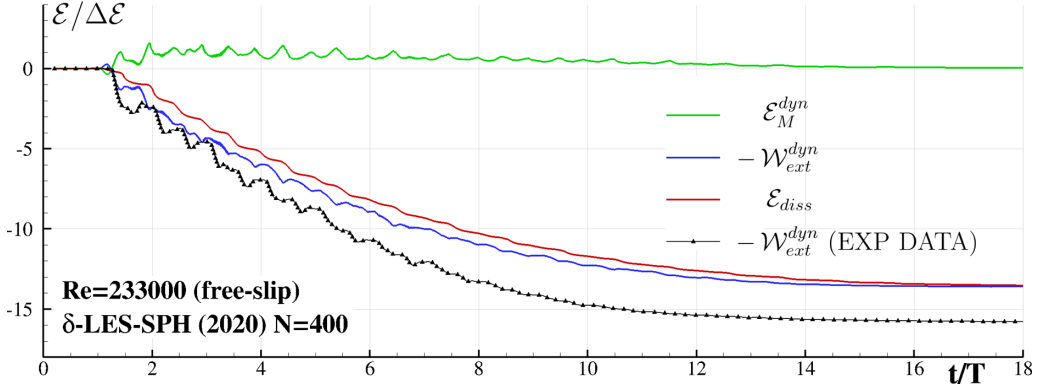
FIG. 16. SPH simulation at N = 400 and Re = 233\,000 . Time history of the mechanical energy \mathcal{E}_M^{dyn} , the dissipated energy \mathcal{E}_{diss} , the external work \mathcal{W}_{ext}^{dyn} . The solid line with \Delta symbols represents \mathcal{W}_{ext}^{dyn} as computed through the experimental data.
