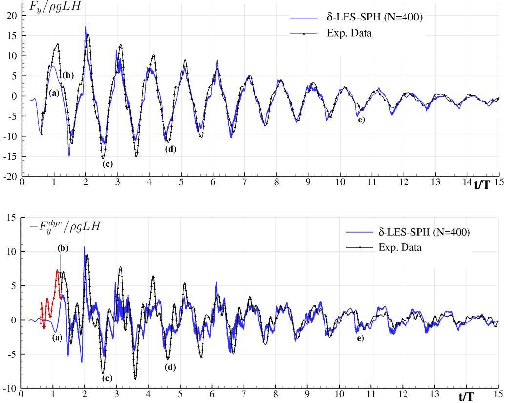
FIG. 13. Force comparison between the experimental data and the SPH simulation at N = 400 and Re = 233\,000 : total force (top) and F_y^{\text{dyn}} component (bottom). On the bottom plot the initial part of the experimental F_y^{\text{dyn}} is colored in red where incorrect overestimation of the force is linked to the release mechanism.
