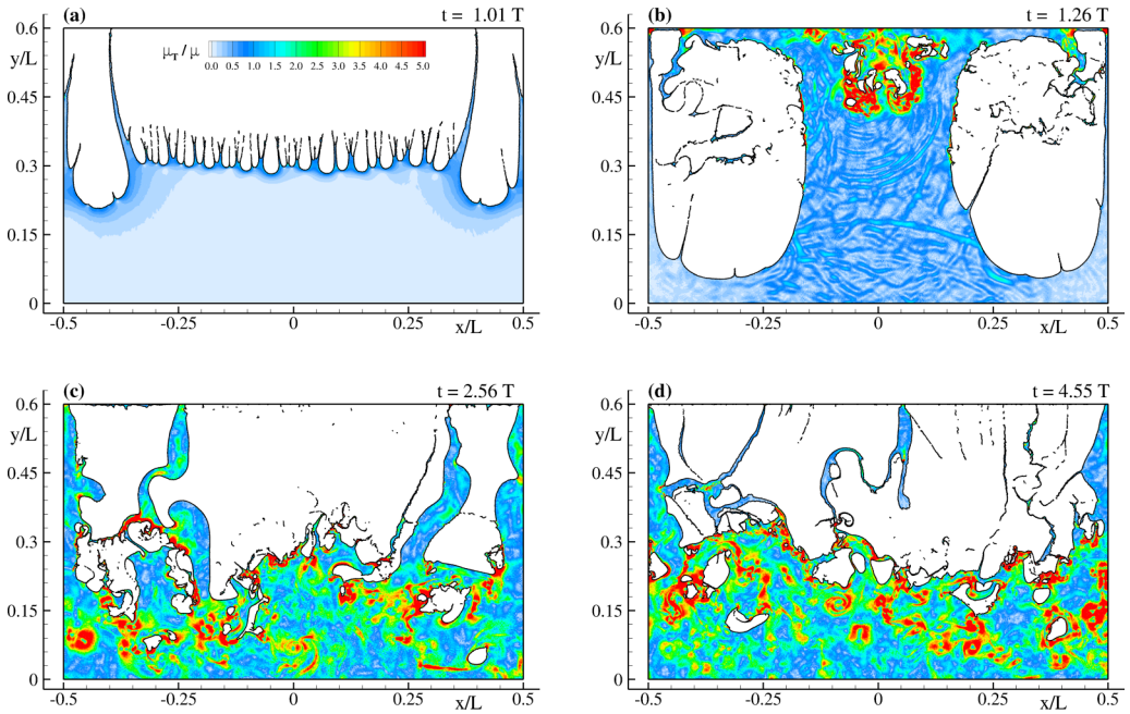
FIG. 6. Four representative instants of the flow evolution obtained by the SPH simulation at N = 400 for the Re = 233\,000 case. Contours refer to turbulent viscosity ratio \mu_T/\mu . See the Supplemental Material [19].
