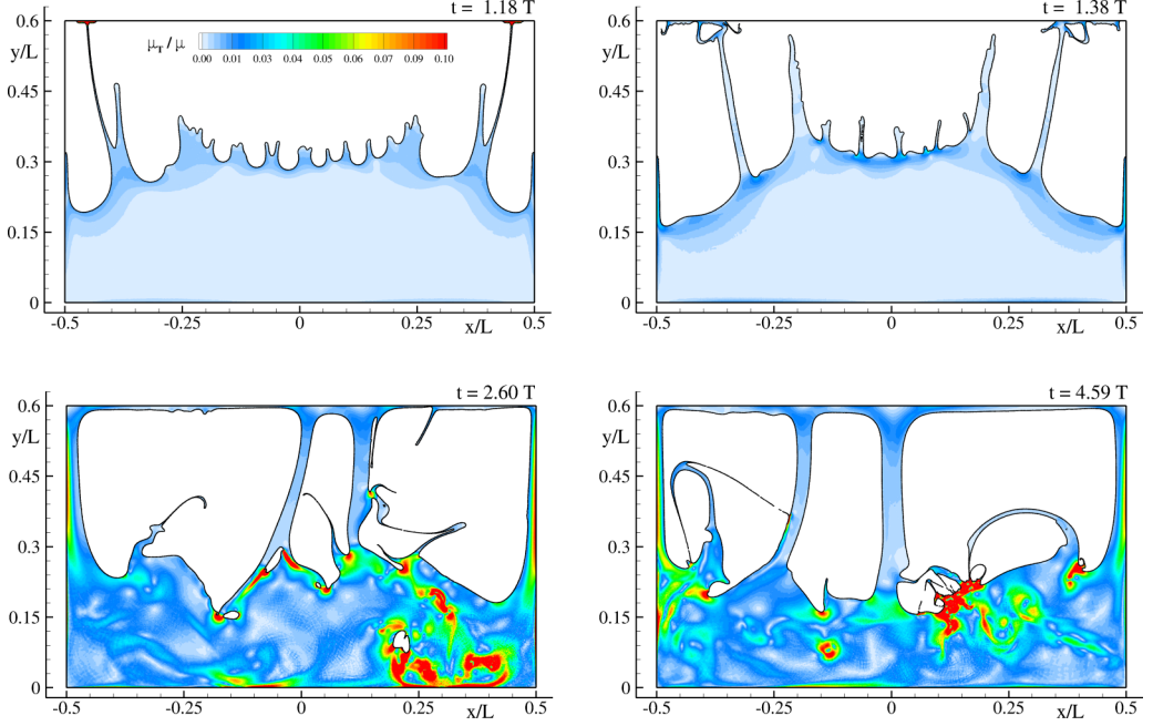
FIG. 9. Four representative instants of the flow evolution obtained by the SPH simulation at N = 400 for the Re = 4660 case. Contours refer to turbulent viscosity ratio \mu_T/\mu . See the Supplemental Material [19].
