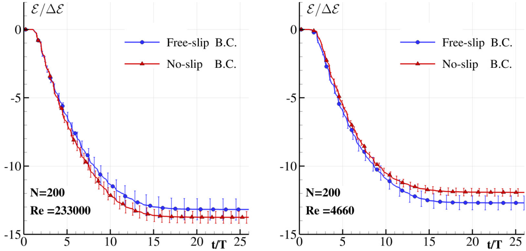
FIG. 20. Time history of the ensemble average of the energy dissipation \mathcal{E}_{\text{diss}} for resolutions N = 200 using free-slip and no-slip conditions on the solid boundaries. Error bars refer to the computed standard deviation. Left: \text{Re} = 233\,000 for water case. Right: \text{Re} = 4660 for oil case.
