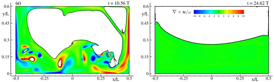
FIG. 10. SPH simulation at N = 400 for the Re = 4660 case: vorticity contour at the same time instants of Fig. 7. See the Supplemental Material [19].
