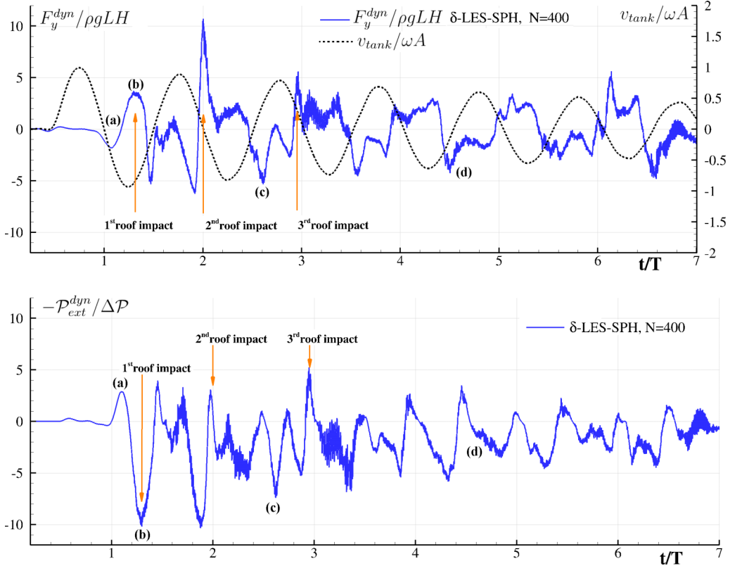
FIG. 14. SPH simulation at N = 400 and Re = 233\,000 . Top plot: total force against the tank velocity; bottom plot: time history of the power -\mathcal{P}_{ext}^{dyn} (see definition in the text).
