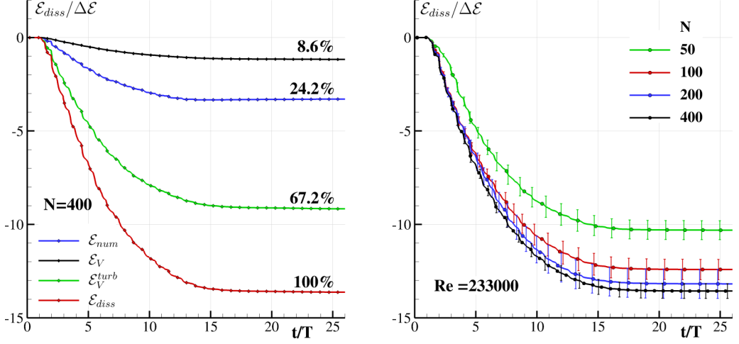
FIG. 8. Left: time history of the energy components defined in Sec. III: resolved viscous dissipation \mathcal{E}_V , modeled turbulent viscous dissipation \mathcal{E}_V^{turb} , numerical diffusion \mathcal{E}_{\mathcal{N}} , total energy dissipation \mathcal{E}_{diss} for the case N = 400 and Re = 233\,000 . Right: ensemble average of the energy dissipation \mathcal{E}_{diss} time history for resolutions N = 50 , N = 100 , N = 200 , and N = 400 ; error bars refer to the computed standard deviation.
