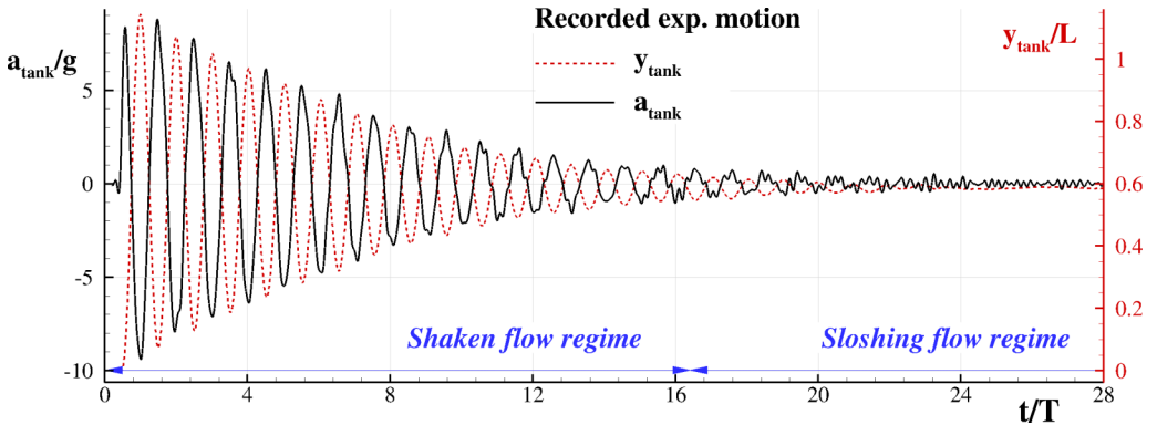
FIG. 4. Tank motion recorded in the experiment of [2] plotted in terms of elevation (dashed line) and acceleration of the tank (solid line).
