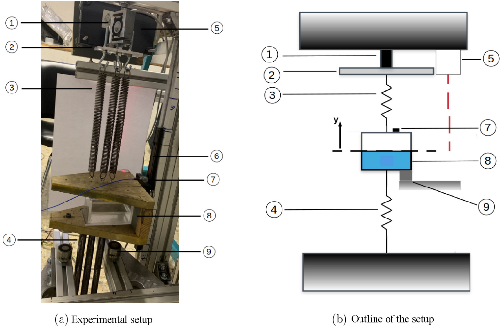
FIG. 1. Experimental setup and outline. (1) Load cell, (2) metallic plate with mass m_p = 0.06 kg, (3) upper set of springs with stiffness constant k_1 = 2154.17 N/m, (4) lower set of springs with stiffness constant k_2 = 2154.17 N/m, (5) laser sensor, (6) mechanical guide, (7) accelerometer, (8) methacrylate tank and C-shaped wooden structure with mass m_s = 2.403 kg, (9) pair of solenoids acting as release mechanism.
