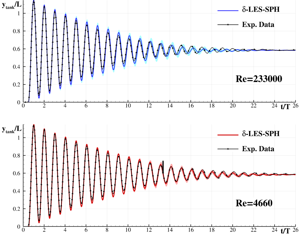
FIG. 18. Evolution of the vertical position of the tank over time obtained from the FSI-SPH simulation at N = 200 . Top figure corresponds to Re = 233\,000 for water and bottom figure to Re = 4660 for oil. The experimental signal obtained from the accelerometer is plotted for comparison. Variability of the numerical outcome, represented in terms of standard deviation, is plotted in lighter color (light blue on the top plot and pink on the bottom one).
