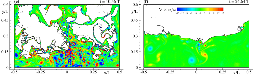
FIG. 7. SPH simulation at N = 400 for the Re = 233\,000 case: vorticity contour at t/T = 10.56 (left plot) and t/T = 24.64 (right plot). See the Supplemental Material [19].
