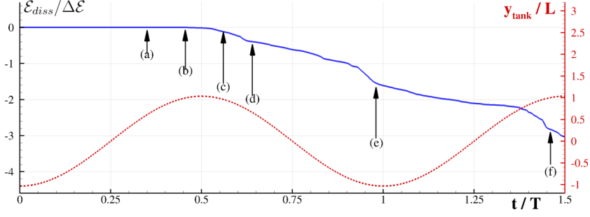
FIG. 3. Dissipated energy \mathcal{E}_{\text{diss}} (solid line) and corresponding tank elevation (dashed line). Labels (a) to (f) are related to plots of Fig. 2.
