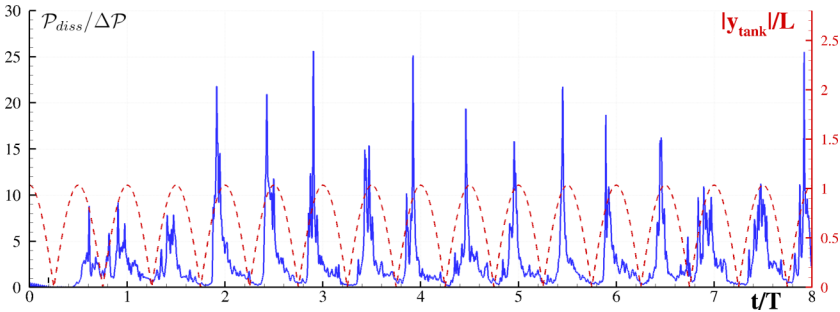
FIG. 9. Time history of the nondimensional time derivative of the dissipated energy, \mathcal{P}_{\text{diss}}/\Delta\mathcal{P} (solid line) and of the absolute value of the tank displacement (dashed line).
