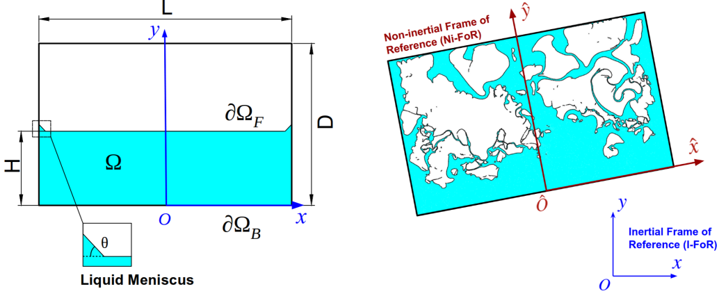
FIG. 1. Left: Sketch of the problem geometry. Right: Example of the tank motion and consequent flow evolution.
