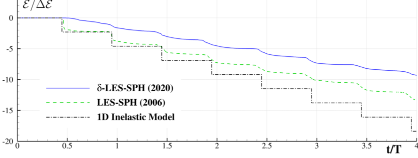
FIG. 8. Comparison of the energy dissipated in the LES-SPH scheme (dashed line), in the present \delta -LES-SPH scheme (solid line) and in the 1D analytical model (dash-dotted line).
