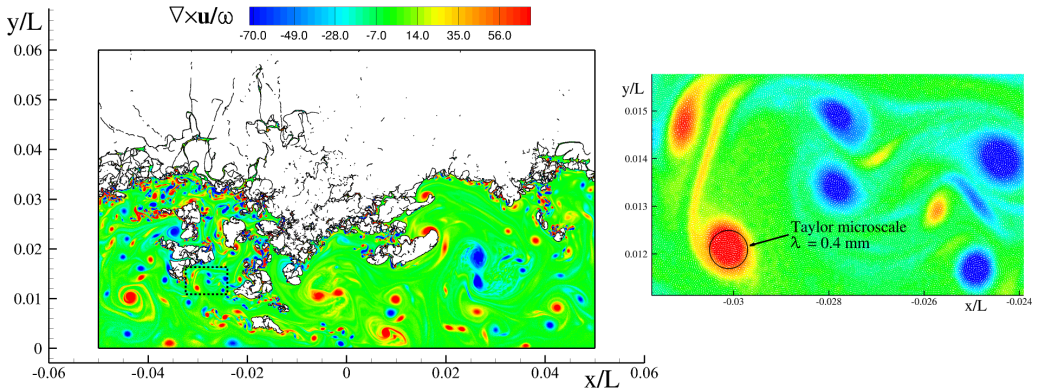
FIG. 11. SPH vorticity field at t/T = 1.25 using a spatial resolution N = 800 . On the right plot an enlargement of the field is depicted comparing the vortices size with the evaluated Taylor microscale.
