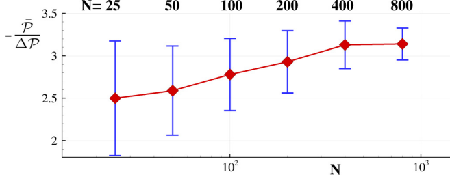
FIG. 19. Average dissipation rates \bar{P} for resolutions N = 25, 50, 100, 200, 400, 800 . The error bars refer to the computed standard deviation for \bar{P} evaluated at each semiperiod of the tank oscillation. For the higher resolution N = 400 and 800 , because of the too high CPU costs, only 20 oscillations are simulated.
