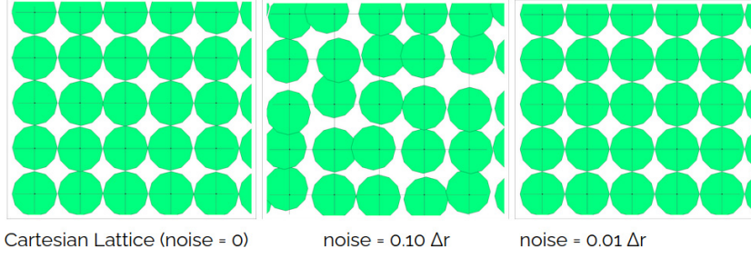
FIG. 16. Sketch of different levels of random noise applied on the initial particle lattice. The right plot shows the 1% noise configuration adopted for the simulations.
