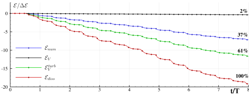
FIG. 13. Time history of the energy components defined in Sec. VI: resolved viscous dissipation \mathcal{E}_V , modeled turbulent viscous dissipation \mathcal{E}_V^{\text{turb}} , numerical diffusion \mathcal{E}_N , total energy dissipation \mathcal{E}_{\text{diss}} . Spatial resolution is N = 200 .
