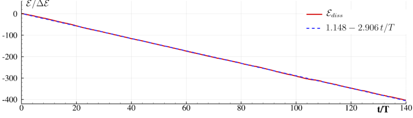
FIG. 14. Energy dissipation over the simulation time duration, that is, 140 periods of oscillation. The solid line represents the raw simulation data, whereas the related regression line is drawn with the dashed line.
