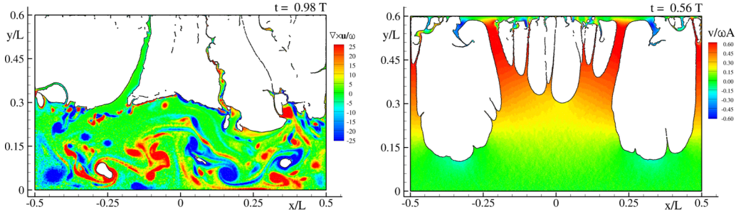
FIG. 4. Left: Vorticity contour at t/T = 0.98 , corresponding to plot (e) of Fig. 2. Right: Contour plot of the vertical component of the velocity field at t/T = 0.56 corresponding to plot (c) of Fig. 2.
