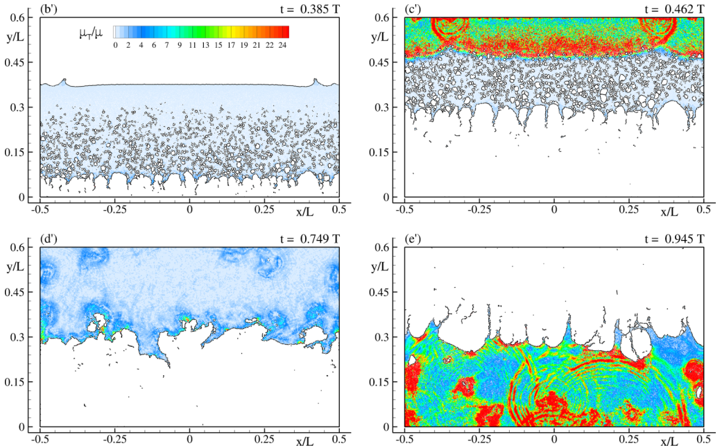
FIG. 5. Flow evolution obtained by LES-SPH. Colors refer to the ratio \mu_T/\mu . Plot sequence is from top to bottom and from left to right. Spatial resolution N = 200 .
