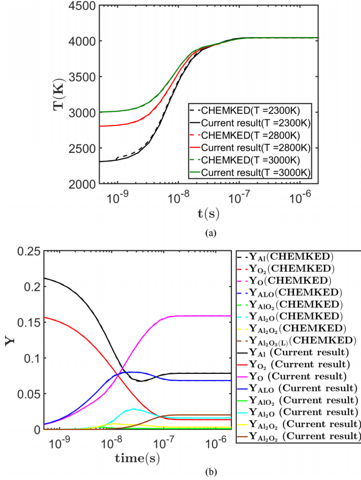
FIG. 3. (a) The temperature rises during the constant volume reaction of the stoichiometric mixture of Al vapor and air, initiated at 2300, 2800, and 3000 K. (b) The evolution of the species mass fraction during constant-volume reaction of Al vapor and air initiated at 2800 K.
