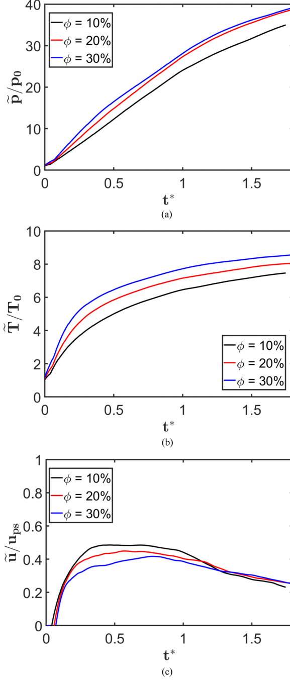
FIG. 12. The comparison of the Favre averaged (a) pressure ( \tilde{p}/p_0 ), (b) temperature ( \tilde{T}/T_0 ), and (c) axial velocity ( \tilde{u}/u_{ps} ) of the gas phase within the particle clusters with \phi = 10\% , 20\% , and 30\% during the interaction with M_s = 3.5 shock. The initial diameter of the particles is 3.844 \mu\text{m} and the corresponding \text{Re}_D is 1000. p_0 = 101\,325.0 \text{ Pa} , and T_0 = 293.54 \text{ K} .
