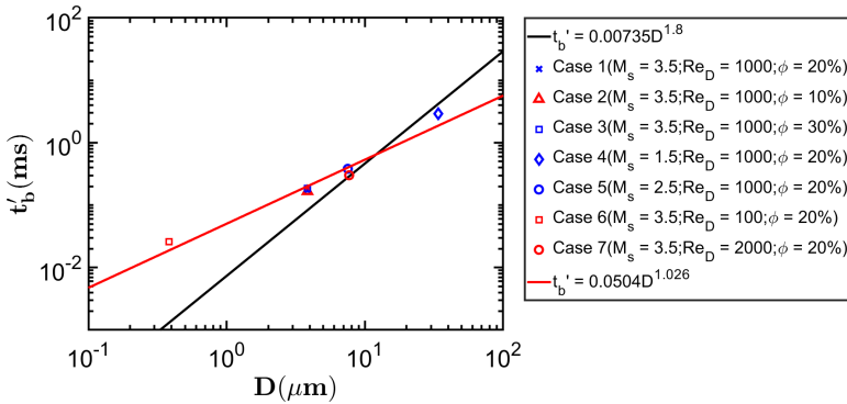
FIG. 17. The scaled burn time ( t'_b ) of the Al particles in the cluster obtained from the current calculations is plotted against the corresponding initial particle diameter ( D ). Current results are compared with the empirical correlation between t'_b and D obtained by Beckstead [7] from experimental data. The black line shows the empirical correlations obtained from experiments in [7]. The symbols show the burn time of Al particle clusters in shocked flows obtained from the current calculations. The red line is a linear least-square fit to the \log_{10} t'_b versus \log_{10} D .
