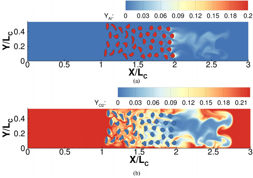
FIG. 10. The contours of (a) Y_{Al} and (b) Y_{O_2} at t^* = 1.8 obtained from the reactive calculation of M_s = 3.5 shock interaction with a cluster of Al particle ( \phi = 20\% , Re_D = 1000 ).
