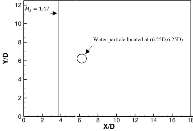
FIG. 1. A schematic diagram of computational setup for the calculation of M_s = 1.47 shock interaction with a cylindrical water particle of 4.8 mm in diameter.
