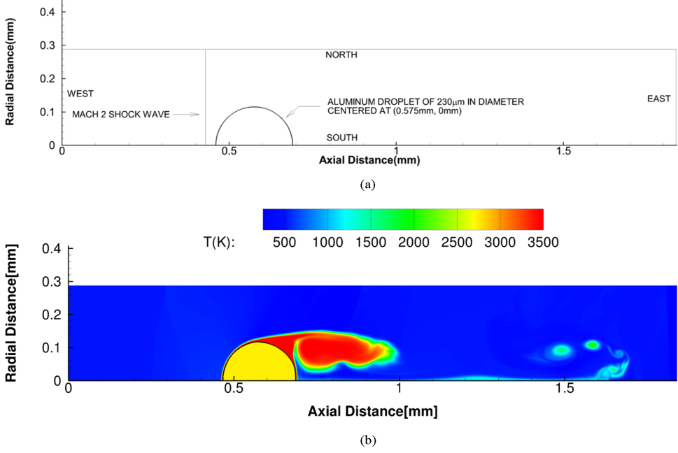
FIG. 4. (a) The initial conditions for the axisymmetric calculation of the combustion of an aluminum particle of 230 \mu\text{m} in diameter during the interaction with an incoming Mach 2 shock. (b) Temperature contours at 2 \mu\text{s} obtained from the axisymmetric calculation of Al particle combustion under the influence of Mach 2 shock.
