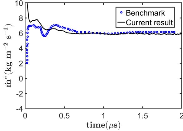
FIG. 5. Comparison of the \dot{m}'' of the burning Al particle of 230 \mu\text{m} in diameter during interaction with the Mach 2 shock obtained from the current calculation and the benchmark result [35].
