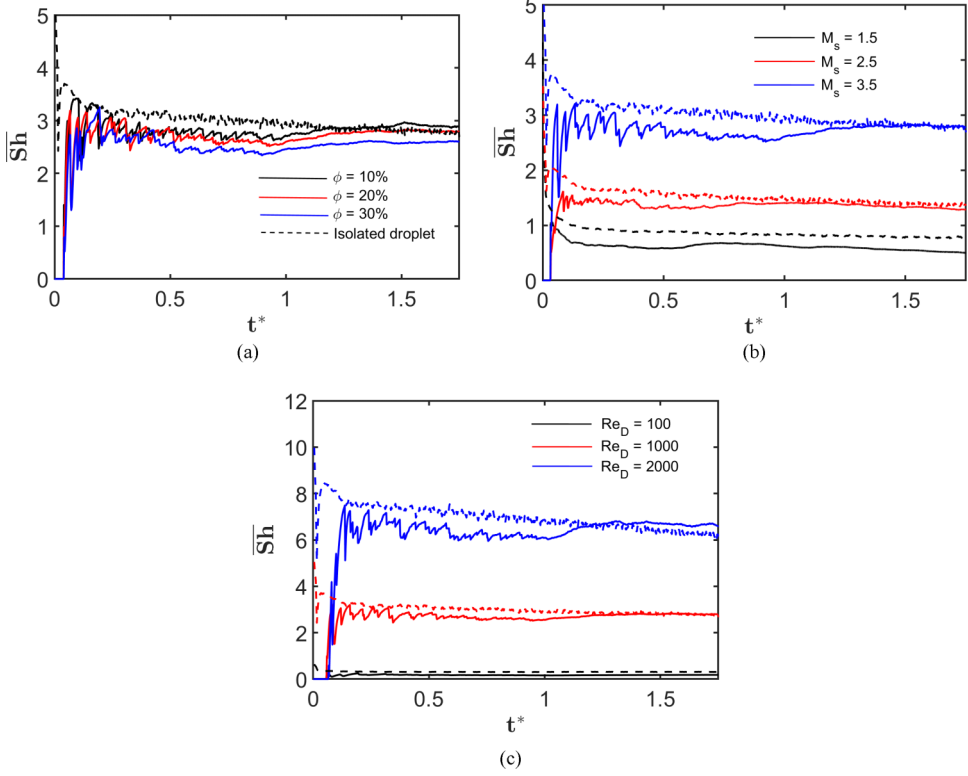
FIG. 14. \overline{Sh} of the particles in the clusters are compared with the Sh of isolated particles in (a), (b), and (c) for different flow conditions characterized by M_s , Re_D , and \phi . (a) shows the comparison of \overline{Sh} for \phi = 10\% , 20\% , and 30\% with an isolated particle at M_s = 3.5 and Re_D = 1000 . (b) shows how \overline{Sh} in a cluster of particles vary with M_s . The \overline{Sh} in a particle cluster for M_s = 1.5 , 2.5 , and 3.5 are compared with an isolated particle subjected to the respective M_s . Re_D = 1000 and \phi = 20\% in these calculations. (c) shows the effect of Re_D on the \overline{Sh} of the particles. Re_D = 100 , 1000 , and 2000 are selected for this comparison. M_s = 3.5 and \phi = 20\% in these calculations. In (b) and (c), solid lines show the \overline{Sh} of the particle cluster and the dashed lines of the same color show the Sh of an isolated particle for the respective M_s and Re_D .
