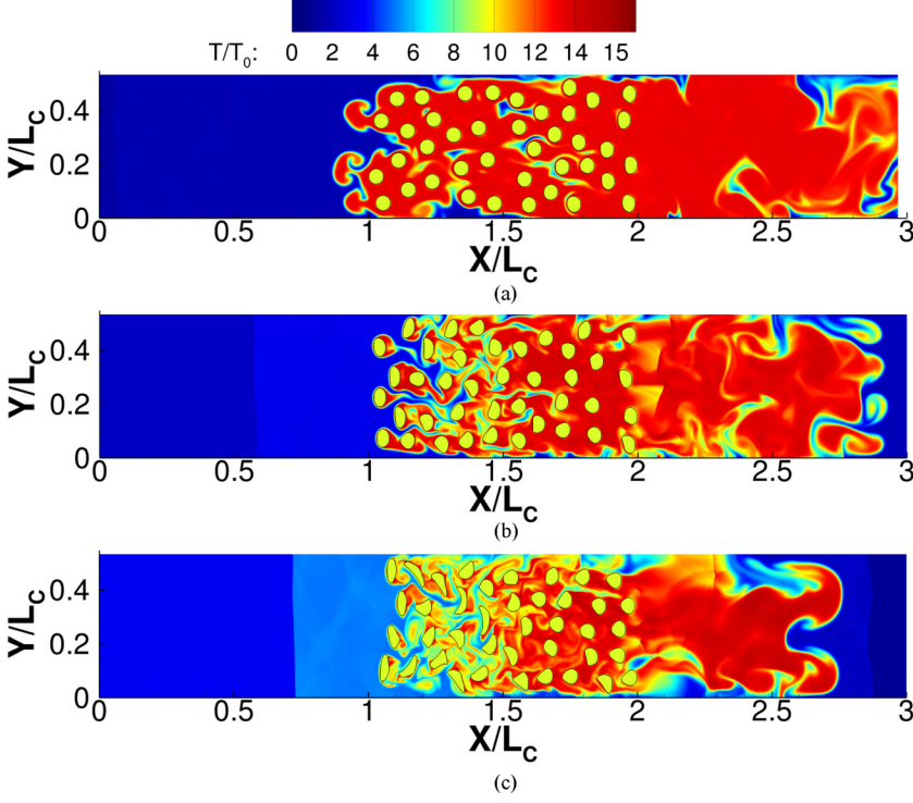
FIG. 15. The temperature contours during the (a) M_s = 1.5 , (b) M_s = 2.5 , and (c) M_s = 3.5 shock interaction with cluster of particles of volume fraction \phi = 20\% at t^* = 1.73 . Re_D = 1000 for all three cases. T_0 = 293.54 K.
