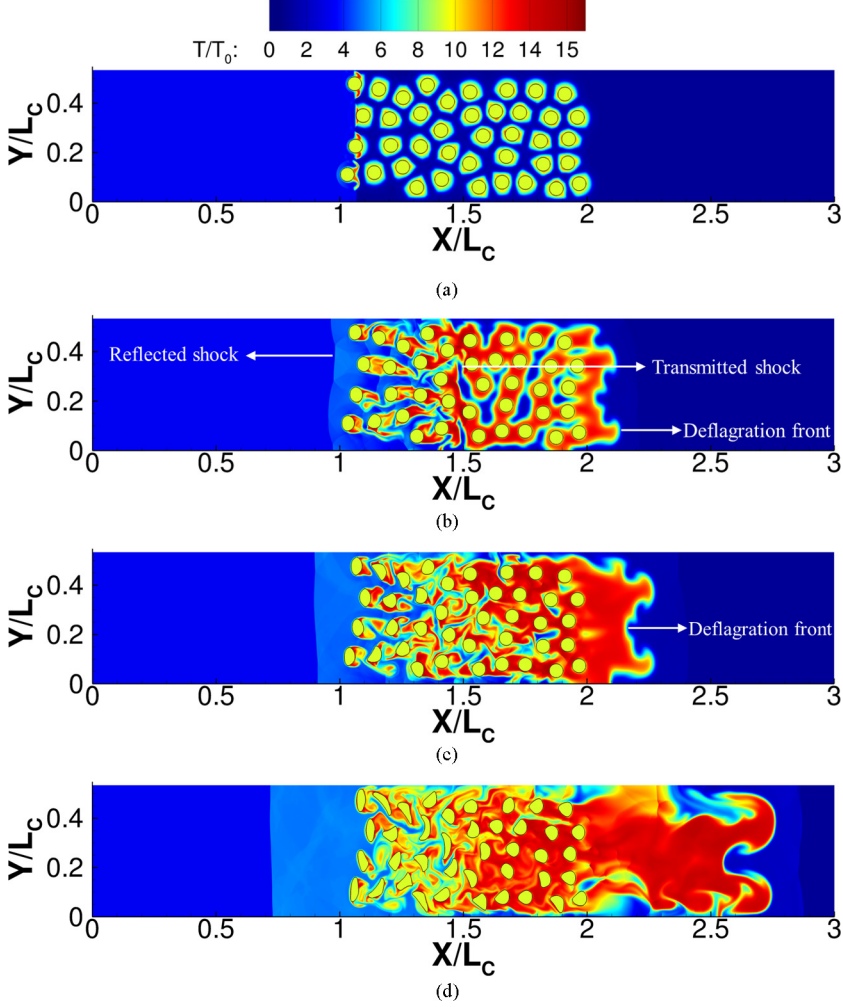
FIG. 8. A sequence of the temperature contours obtained from the reactive calculation of M_s = 3.5 shock interaction with an Al particle cluster of \phi = 20\% . The diameter of the particles is selected 3.844 \mu\text{m} to ensure \text{Re}_D = 1000 . T_0 = 293.54 \text{ K} .
