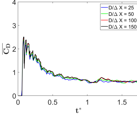
FIG. 7. \overline{C_D} of the particles in the cluster during interaction with a M_s = 3.5 shock at Re_D = 1000 , obtained using four different grid resolutions.
