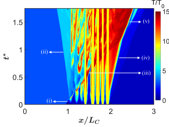
FIG. 9. The x - t^* plots of the temperature extracted from \frac{y}{L_c} = 0.25 in the computational domain during the combustion of Al particle cluster of \phi = 20\% under influence of an incoming M_s = 3.5 shock at Re_D = 1000 . Legends: (i) Incoming M_s = 3.5 shock, (ii) reflected shock, (iii) transmitted shock, and (iv) diffusion flame front (v) deflagration front. p_0 = 101325.0 Pa and T_0 = 293.54 K.
