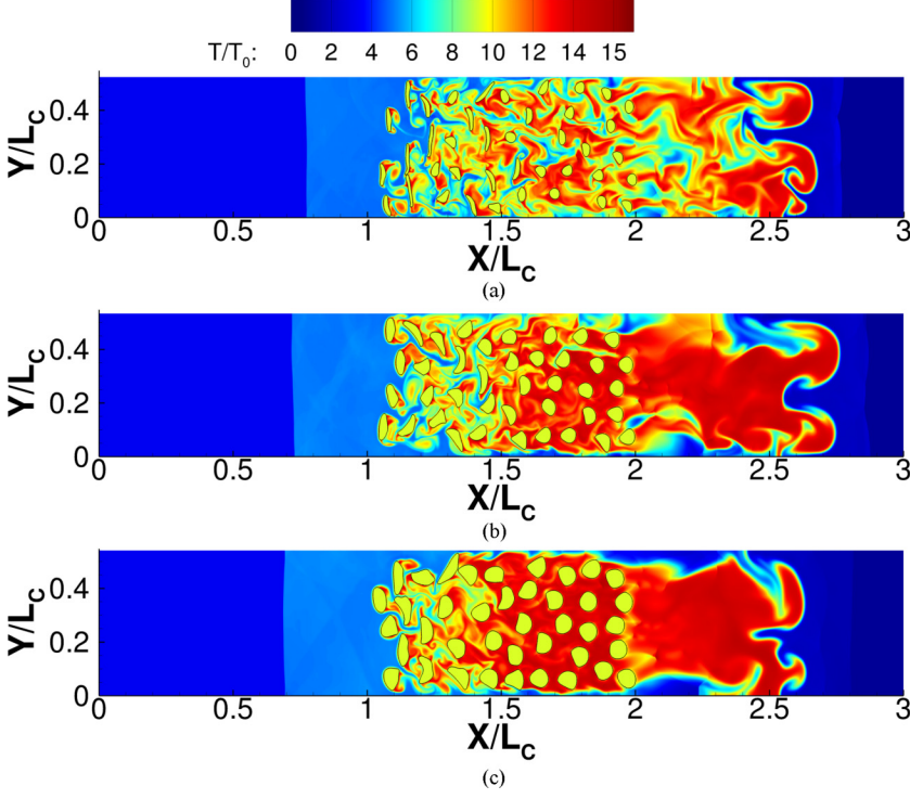
FIG. 13. The temperature contours during the M_s = 3.5 shock interaction with cluster of particles of volume-fractions (a) \phi = 10\% , (b) \phi = 20\% , and (c) \phi = 30\% at t^* = 1.73 . The initial diameters of the particles are 3.844 \mu\text{m} . T_0 = 293.54 \text{ K} .
