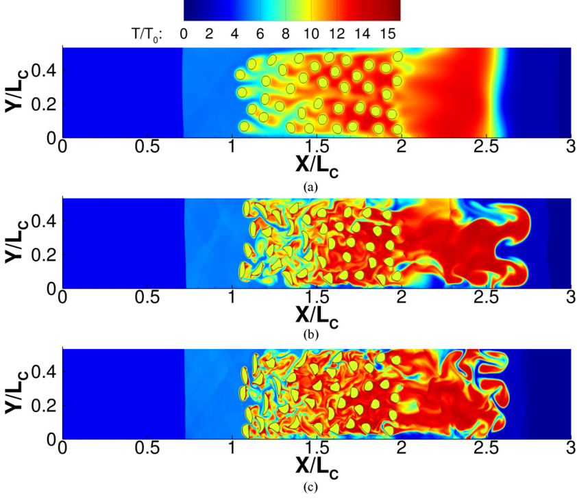
FIG. 16. The temperature contours during M_s = 3.5 shock interaction with particles clusters of \phi = 20\% and (a) Re_D = 100 , (b) Re_D = 1000 , and (c) Re_D = 2000 at t^* = 1.73 . T_0 = 293.54 K.
