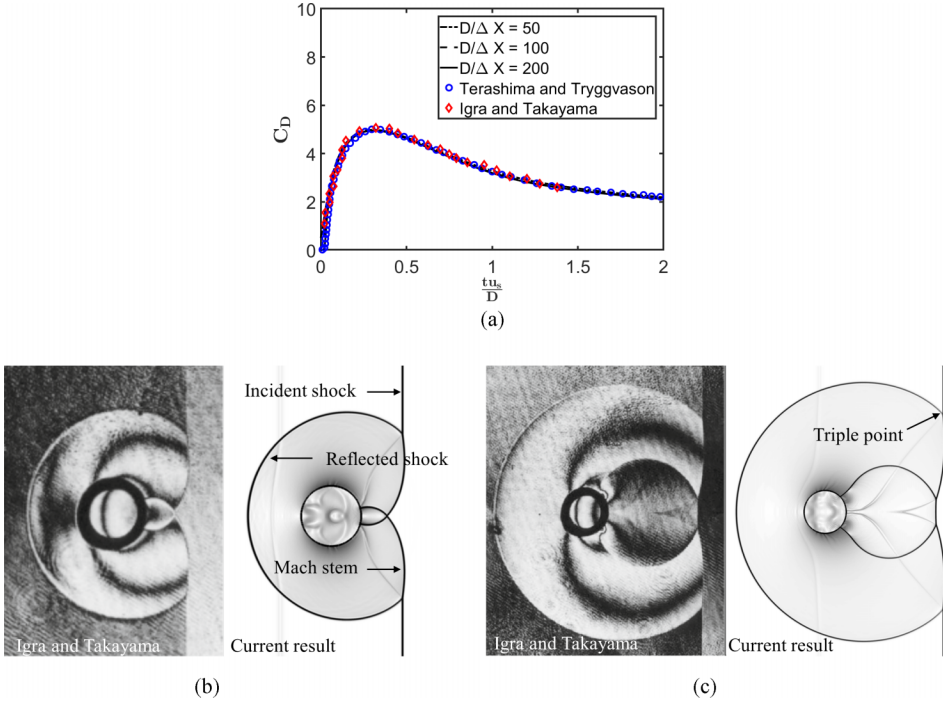
FIG. 2. Comparison of current and benchmark results for M_s = 1.47 shock interaction with a cylindrical water particle of 4.8 mm in diameter. The drag coefficient obtained from the current calculations using three different mesh resolutions ( \frac{D}{\Delta x} = 50, 100 , and 200 ) are compared with benchmark numerical results obtained by Terashima and Tryggvason [60] and Igra and Takayama [67] in (a). The numerical Schlierens are compared with the experimental results at time \frac{tu_s}{D} = 1.7 and 3.38 in (b) and (c) respectively. Images in (b) and (c) are reprinted from [59] with permission from Springer.
