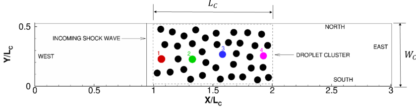
FIG. 6. The initial computational setup for the numerical calculations of shock interaction with a reacting Al particle cluster.
