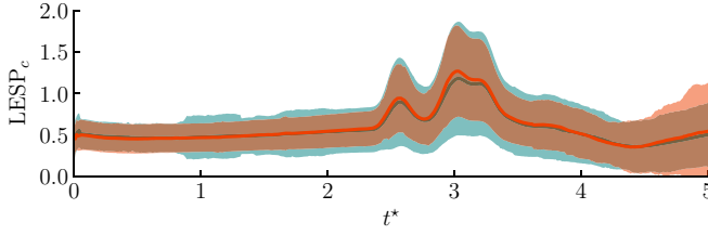
FIG. 7. Time history of the ensemble mean value of the LESPc of an impulsively translating plate at 20^\circ subject to actuation, averaged over 100 realizations, from the inviscid vortex model with sEnKF (teal line) and the inviscid vortex model with ETKF (orange line). Shaded areas show the 95% confidence interval for the inviscid vortex model with sEnKF and ETKF.
