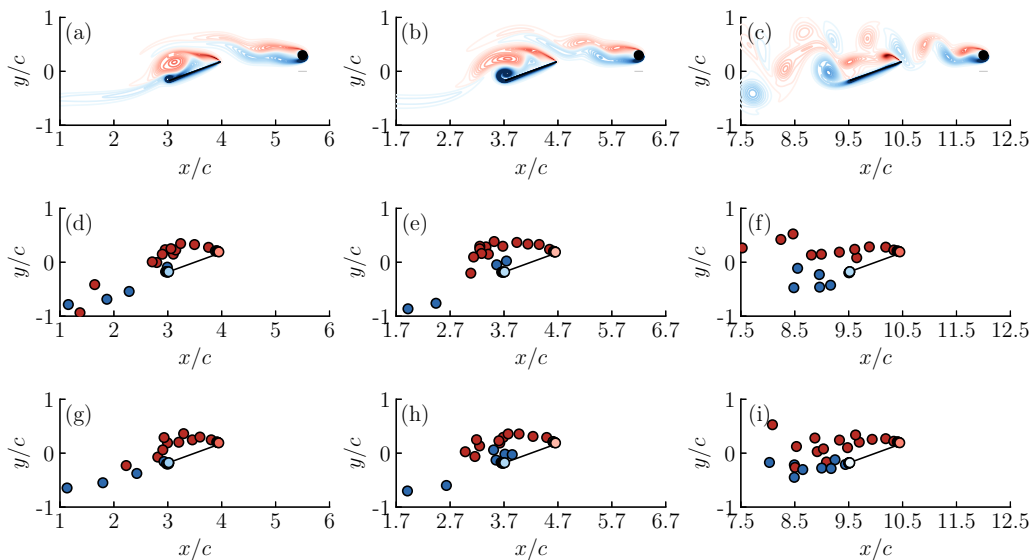
FIG. 12. Snapshots of the vorticity distribution at t^* = 3.5 (left column), t^* = 4.2 (middle column), and t^* = 10.0 (right column) for an impulsively translating plate at 20^\circ in a cylinder wake, predicted from (a)–(c) high-fidelity numerical simulation at Reynolds number 500, (d)–(f) inviscid vortex model with sEnKF, and (g)–(i) inviscid vortex model with ETKF.
