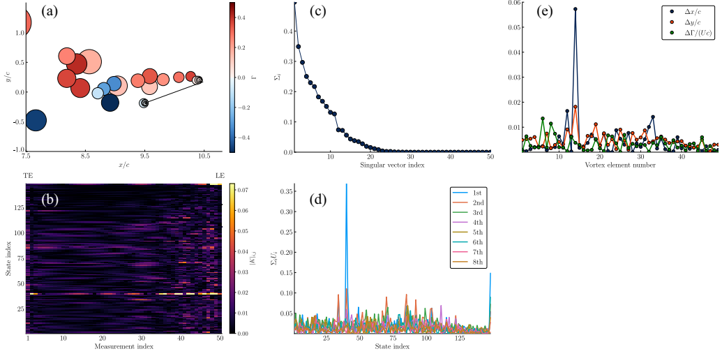
FIG. 17. Study of the analysis step at t^* = 10 for the impulsively translating plate in the cylinder wake. (a) Vorticity distribution from the discrete vortex model with ETKF. Sizes indicate “age” of the vortices (large means old). Colors indicate vorticity sign (blue is negative). (b) Elementwise magnitude of the Kalman gain. (c) Singular values of the Kalman gain. (d) First eight left singular vectors of the Kalman gain scaled by their associated singular value. (e) Mean difference of x , y position and circulation of vortices during the analysis step.
