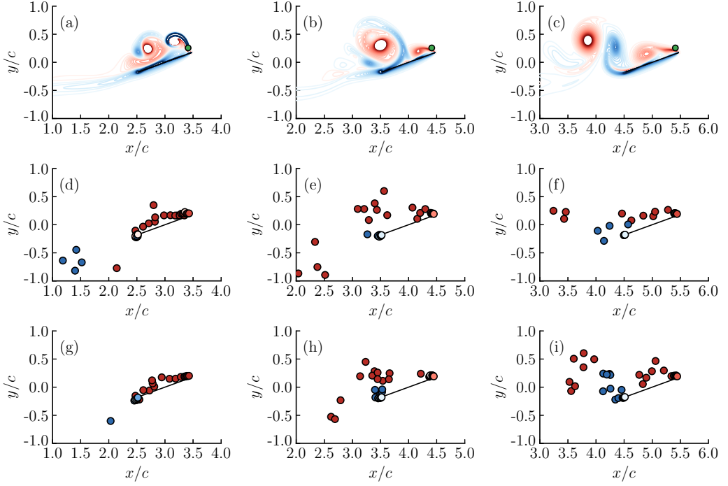
FIG. 6. Snapshots of the vorticity distribution at t^* = 3.0 (left column), t^* = 4.0 (middle column), and t^* = 5.0 (right column) for an impulsively translating plate at 20^\circ subject to actuation, predicted from (a)–(c) high-fidelity numerical simulation at Reynolds number 500, (d)–(f) inviscid vortex model with sEnKF, and (g)–(i) inviscid vortex model with ETKF.
