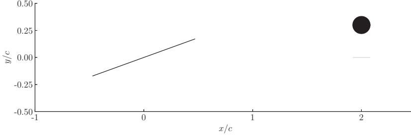
FIG. 10. Schematic of a plate at 20^\circ behind a cylinder. The plate and cylinder translate to the right at uniform speed.
