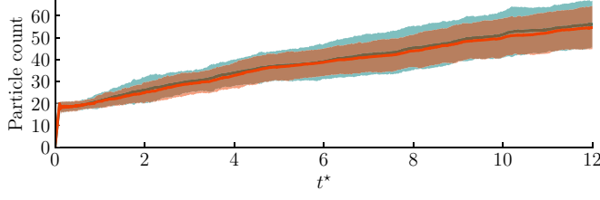
FIG. 15. Time history of the particle count for an impulsively translating plate at 20^\circ in a cylinder wake, averaged over 100 realizations, from the inviscid vortex model with sEnKF (teal line) and the inviscid vortex model with ETKF (orange line). Shaded areas show the 95% confidence interval for the inviscid vortex model with sEnKF and ETKF.
