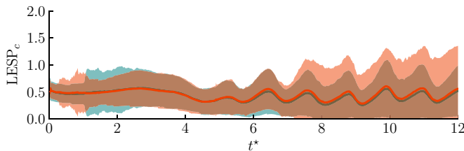
FIG. 14. Time history of the ensemble mean value of the LES P_c of an impulsively translating plate at 20^\circ in a cylinder wake, averaged over 100 realizations, from the inviscid vortex model with sEnKF (teal line) and the inviscid vortex model with ETKF (orange line). Shaded areas show the 95% confidence interval for the inviscid vortex model with sEnKF and ETKF.
