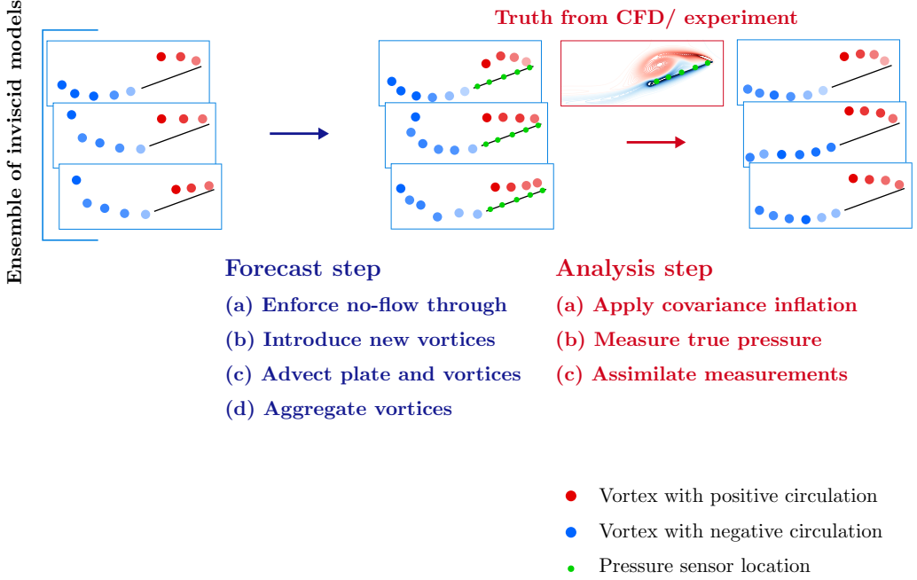
FIG. 2. One time step of the data-assimilated aggregated vortex model.
