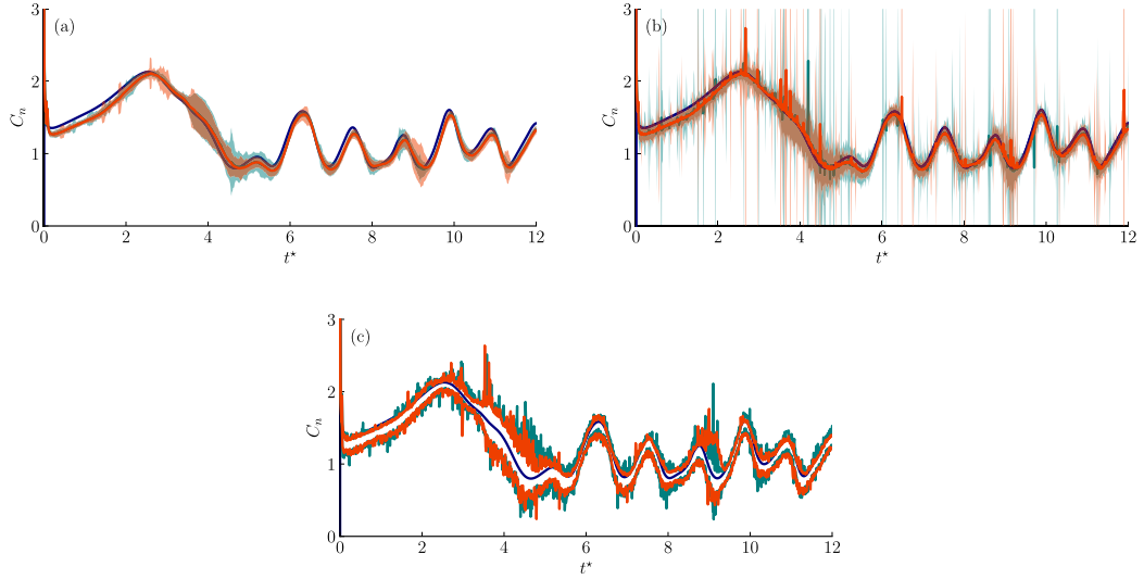
FIG. 13. Top left panel (a): Normal force coefficient of an impulsively translating plate at 20^\circ in a cylinder wake, from high-fidelity numerical simulation at Reynolds number 500 (blue line), mean over 100 realizations of the inviscid vortex model with sEnKF (teal line), mean over 100 realizations of the inviscid vortex model with ETKF (orange line). Shaded areas show the 95% confidence interval for the inviscid vortex model with sEnKF and ETKF. Top right panel (b): Comparison with the same normal force coefficient from high-fidelity simulation, but without application of the median filter for the sEnKF (teal line) and ETKF (orange line). Lower panel (c): Comparison of the same normal force coefficient from high-fidelity simulation, with the 2.5% (lower curve) and 97.5% (upper curve) quantiles of the normal force coefficient over 100 realizations of the inviscid vortex model for the sEnKF (teal line) and ETKF (orange line) without application of the median filter.
