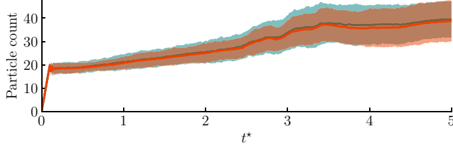
FIG. 8. Time history of the particle count for an impulsively translating plate at 20^\circ subject to actuation, averaged over 100 realizations, from the inviscid vortex model with sEnKF (teal line) and the inviscid vortex model with ETKF (orange line). Shaded areas show the 95% confidence interval for the inviscid vortex model with sEnKF and ETKF.
