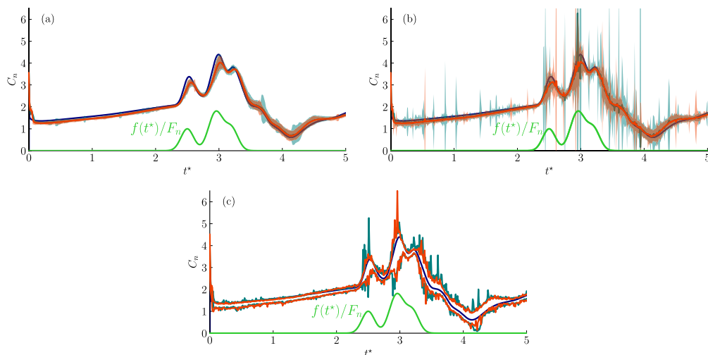
FIG. 5. Top left panel (a): Normal force coefficient of an impulsively translating plate at 20^\circ subject to actuation, from high-fidelity numerical simulation at Reynolds number 500 (blue line), mean over 100 realizations of the inviscid vortex model with sEnKF (teal line), mean over 100 realizations of the inviscid vortex model with ETKF (orange line). Shaded areas show the 95% confidence interval for the inviscid vortex model with sEnKF and ETKF. Time history of the flow actuation (lime green line). Top right panel (b): Comparison with the same normal force coefficient from high-fidelity simulation, but without application of the median filter for the sEnKF (teal line) and ETKF (orange line). Lower panel (c): Comparison of the same normal force coefficient from high-fidelity simulation, with the 2.5% (lower curve) and 97.5% (upper curve) quantiles of the normal force coefficient over 100 realizations of the inviscid vortex model for the sEnKF (teal line) and ETKF (orange line) without application of the median filter.
