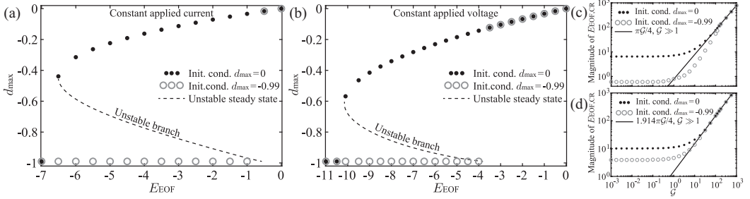
FIG. 6. Hysteresis for the onset of instability. [(a),(b)] The maximum deformation d_{\max} at steady state as a function of E_{\text{EOF}} for a constant current (a) and a constant voltage (b) actuation modes. [(c),(d)] The magnitude of the threshold elasto-electro-osmotic number E_{\text{EOF,CR}} as a function of \mathcal{G} for a constant current (c) and a constant voltage (d) actuation modes, resulting from two different initial states of the system. Black dots represent the results obtained from an initially flat elastic sheet and gray dots represent the results obtained from an initially deformed elastic sheet which adhered to the floor, corresponding to d_{\max} = -0.99 . Black dashed lines in panels (a) and (b) represent unstable equilibrium solutions obtained from Eq. (23). Black solid lines in panels (c) and (d) represent the asymptotic solutions for \mathcal{G} \gg 1 , showing that in this case |E_{\text{EOF,CR}}| scales linearly with \mathcal{G} . All calculations were performed using k = 1 , \mathcal{B} = \mathcal{G} = 0 , and h_r = 10^{-2} .
