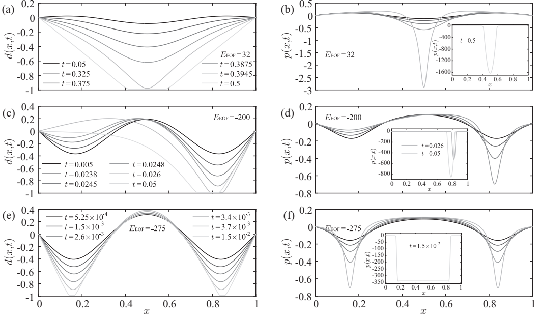
FIG. 8. Investigation of symmetric and asymmetric deformation patterns resulting from a symmetric actuation with a constant applied voltage, in the case of a strongly prestretched elastic sheet. [(a),(c),(e)] The time evolution of the deformation field for E_{\text{EOF}} = 32 (a), E_{\text{EOF}} = -200 (c), and E_{\text{EOF}} = -275 (e). [(b),(d),(f)] The time evolution of the corresponding pressure field. The insets in [(b),(d),(f)] present the pressure distribution in the fluid, as the film thickness reduces to h = h_r . All calculations were performed using k = 3 and \mathcal{B} = \mathcal{G} = 0 .
