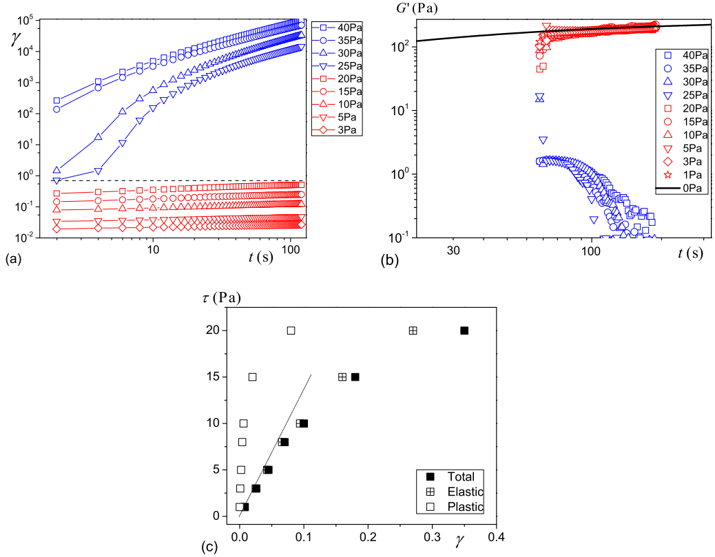
FIG. 9. Laponite suspension: (a) deformation vs time during creep tests under different stress levels; the horizontal dashed line is a guide for the eye; (b) elastic modulus under low stress oscillations during creep tests; (c) shear stress vs induced deformation during recovery tests (stress release): elastic (reversible) component, plastic (irreversible) component, and total deformation. The dotted line is the equation \tau = G_\infty \gamma , with G_\infty taken as the constant G' (135 Pa here) in small-oscillations tests. Note that for (a) the initial time is the time at which the stress is imposed, while for (b) it is the time just after preshear.
