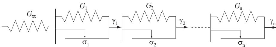
FIG. 6. Representation of the complete model (see text) in discrete form.
