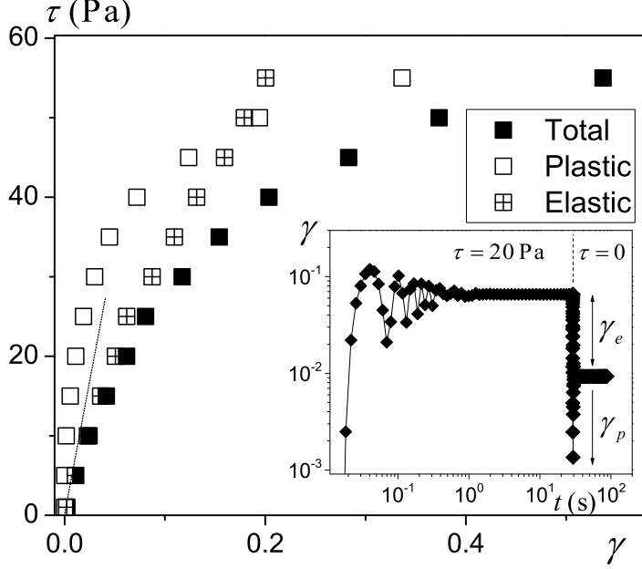
FIG. 3. Shear stress vs induced deformation during recovery tests (stress release) for the emulsion: elastic (reversible) component (crossed squares); plastic (irreversible) component (open squares); total deformation (filled squares). The dotted line is the equation \tau = G_{\infty}\gamma , with G_{\infty} taken as the constant G' (490 Pa for the emulsion) in small-oscillations tests. The inset shows a typical recovery test: deformation induced during creep test, then deformation recovery for stress release, allowing to distinguish the two (elastic and plastic) components.
