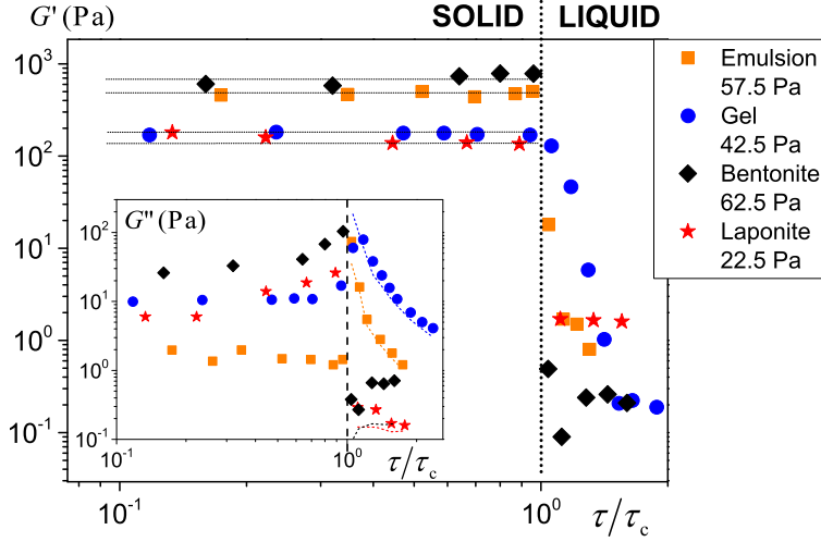
FIG. 2. Elastic modulus for low oscillations during creep tests as a function of the imposed shear stress value rescaled by the yield stress, for different materials: emulsion (orange squares), Carbopol gel (blue circles), laponite suspension (red stars), bentonite suspension (black diamonds). The legend gives the material yield stress values. The horizontal dotted lines indicate the (mean) value ( G_\infty ) retained for the elastic modulus in the solid regime for each material. The inset shows the loss modulus measured during the same creep tests by means of small oscillations (same symbols). The dashed lines in the inset correspond to the calculated G'' values at first order according to theory (see text). Note that for laponite and bentonite the moduli values are taken 20 s after the test beginning, i.e., before the significant evolutions observed later during the flow (see Appendix A).
