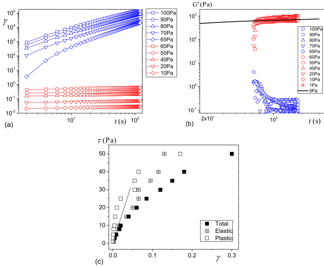
FIG. 8. Bentonite suspension: (a) Deformation vs time during creep tests under different stress levels; (b) elastic modulus under low stress oscillations during creep tests; (c) shear stress vs induced deformation during recovery tests (stress release): elastic (reversible) component, plastic (irreversible) component, and total deformation. The dotted line is the equation \tau = G_\infty \gamma , with G_\infty taken as the constant G' (680 Pa here) in small-oscillations tests. Note that for (a) the initial time is the time at which the stress is imposed, while for (b) it is the time just after preshear.
