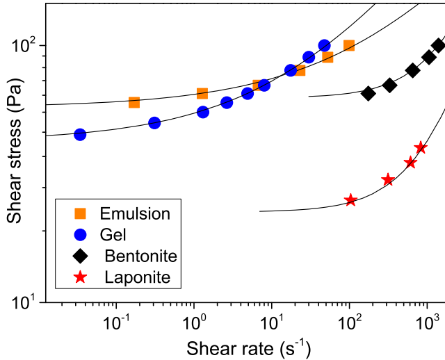
FIG. 11. Flow curve data for the different materials as deduced from steady-state flows during creep tests. The continuous lines are the Herschel-Bulkley models fitted to the different material data: emulsion ( k = 7 \text{ Pa s}^n , n = 0.38 ), gel ( k = 12 \text{ Pa s}^n , n = 0.4 ), bentonite ( k = 0.027 \text{ Pa s}^n , n = 1 ), and laponite ( k = 0.02 \text{ Pa s}^n , n = 1 ).
