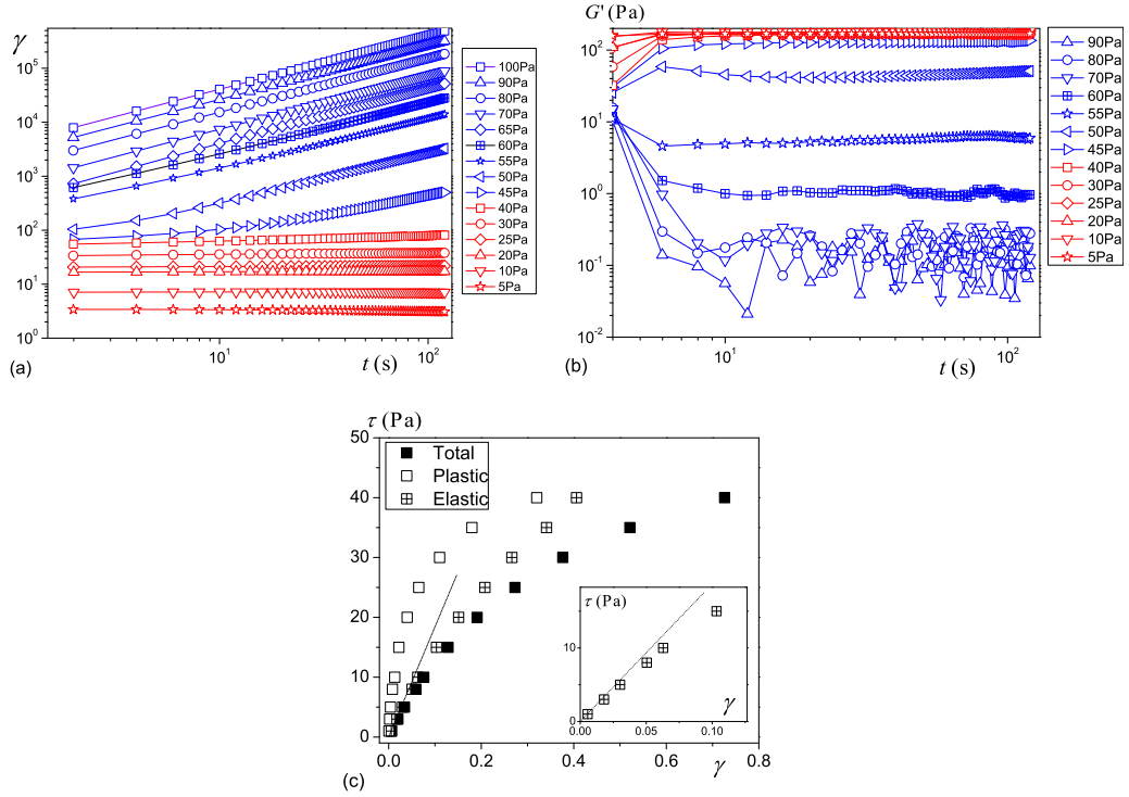
FIG. 7. Gel: (a) Deformation vs time during creep tests under different stress levels; (b) elastic modulus under low stress oscillations during creep tests; (c) shear stress vs induced deformation during recovery tests (stress release): elastic (reversible) component, plastic (irreversible) component, and total deformation. The dotted line is the equation \tau = G_\infty \gamma , with G_\infty taken as the constant G' (183 Pa here) in small-oscillations tests. The inset shows a zoom of these data on low stress values to better appreciate the deviation of elastic deformation from linearity in that range.
