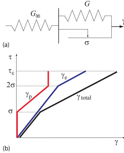
FIG. 5. (a) Representation of the simplest model reproducing the constant elastic network and some additional elastoplastic component. (b) Resulting elastic, plastic, and total deformation components when submitted to stress, then recovery, for different stress levels.
