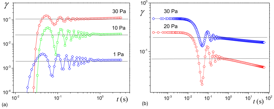
FIG. 10. (a) Deformation vs time observed for creep tests on bentonite suspension at different stress levels. The horizontal dotted lines show the level of the plateau deformation retained as the measure of the elastoplastic deformation. (b) Deformation vs time observed with Carbopol gel during recovery tests, after creep tests under different stress levels. The horizontal dotted lines show the level of the plateau deformation retained as the measure of the residual (plastic) deformation.
