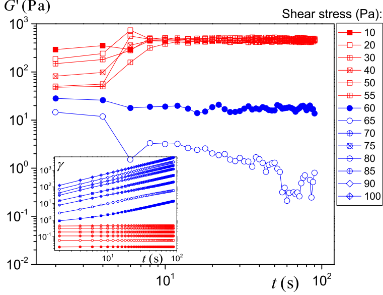
FIG. 1. Elastic modulus of the emulsion measured from oscillations under low stress amplitude as a function of time during creep tests under various shear stress values (see legend). The red squares correspond to the solid regime ( \tau < \tau_c ); the blue circles correspond to the liquid regime ( \tau > \tau_c ). The inset shows the corresponding deformation undergone by the fluid in time (same symbols).
