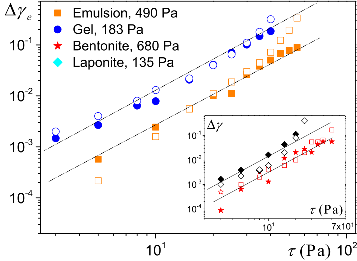
FIG. 4. Additional elastic deformation (filled symbols) with regard to the deformation of the constant elastic network, and plastic deformation (open symbols), as a function of the stress applied for different materials (same type of data in the inset). The dotted lines (of slope 2) correspond to the model fitted to data (see text) with \alpha = 0.8 (emulsion); \alpha = 1 (gel); \alpha = 0.5 [colloid (laponite)]; \alpha = 1.2 [clay (bentonite)].
