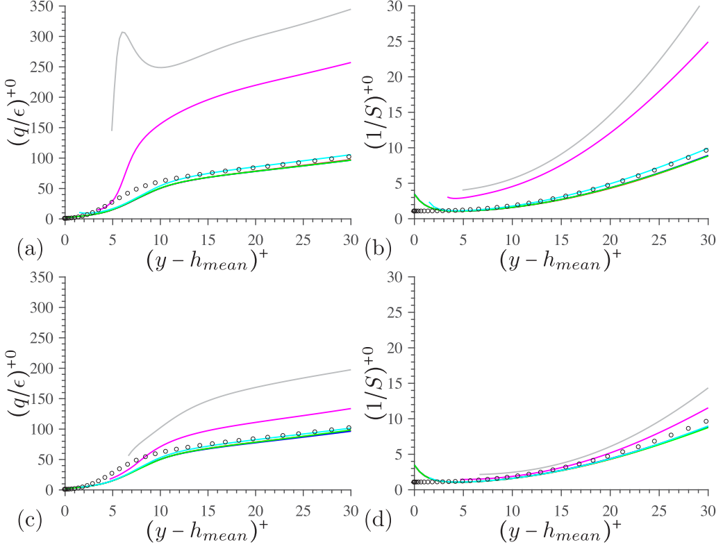
FIG. 17. (a), (c) Eddy turnover timescale, q/\epsilon , and (b), (d) mean shear flow timescale, (1/S) , for \text{Re}_\tau \approx 395 : (a), (b) m = 0.02 , (c), (d) m = 0.4 (symbols and lines as in Fig. 2).
