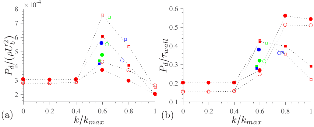
FIG. 9. (a) Form drag and (b) its contribution with respect to the total shear at the wall as function of the position of the interface: m = 0.02 (SHS, \circ ); m = 0.4 (LIS, \square ); open symbols, \text{Re}_\tau \approx 180 ; solid symbols, \text{Re}_\tau \approx 395 ; red, \text{We}^+ = 0 , green, \text{We}^+ \approx 10^{-2} ; and blue, \text{We}^+ \approx 10^{-3} .
