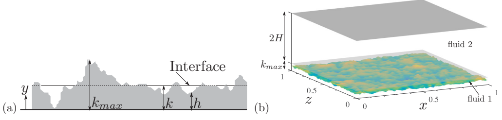
FIG. 1. (a) Sketch of the surface and definitions of k , k_{max} , and h . (b) A portion of the computational domain showing the substrate, the interface between the two fluids, and the definition of H .
