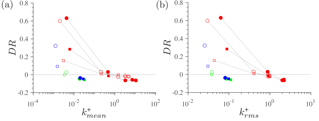
FIG. 10. Drag reduction as a function (a) of the mean surface above the interface normalized in wall units and (b) of its rms for We = 0 : m = 0.02 (SHS, \circ ); m = 0.4 (LIS, \square ); open symbols, Re_\tau \approx 180 ; solid symbols, Re_\tau \approx 395 .
