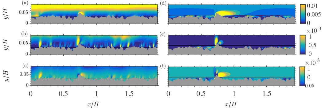
FIG. 11. Color contours of the variance of (a), (d) streamwise velocity fluctuations \langle uu \rangle , (b), (e) wall-normal velocity fluctuations \langle vv \rangle , and (c), (f) covariance of streamwise and wall-normal velocity fluctuations \langle uv \rangle in a vertical section at z/H = 0.56 : the interface positions (a)–(c) k/k_{\max} = 0.6 and (d)–(f) k/k_{\max} = 0.8 ; in both cases \text{Re}_\tau \approx 180 and m = 0.02 .
