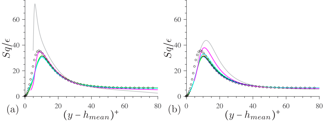
FIG. 15. Shear rate parameter ( Sq/\epsilon ) for (a) m = 0.02 (SHS) and (b) m = 0.4 (LIS) with Re_\tau \approx 395 and We = 0 for different interface positions (symbols and lines as in Fig. 2).
