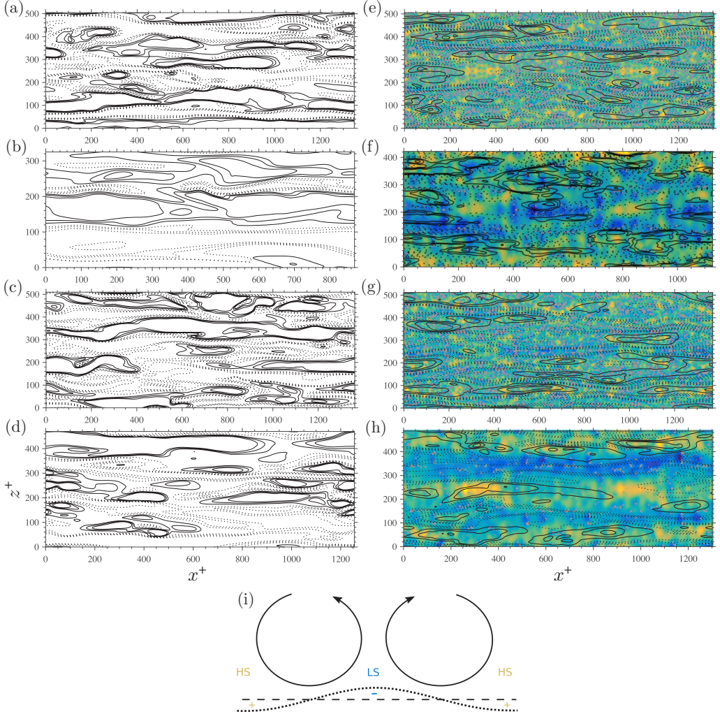
FIG. 13. Isocontours of streamwise velocity fluctuations at Re = 2800 and We = 0 : (a), (c) k = 0.6 and (b), (d) k = 0.8 . For (e), (g) We = 10^{-2} and (f), (h) We^+ \simeq 10^{-3} , the isocontours of streamwise velocity fluctuations are superposed to the displacement of the interface with respect to its time-averaged position (e), (g) \bar{k} = 0.6154 , (f), (h) \bar{k} = 0.76 . Two viscosity ratios are shown, (a), (b), (e), (f) m = 0.02 and (c), (d), (g), (h) m = 0.4 , which mimic idealized SHSs and LISs, respectively. A sketch of streamwise vortices, low and high speed streaks, and deformed interface (dotted line) with respect to the mean interface position \bar{k} is included as a reference.
