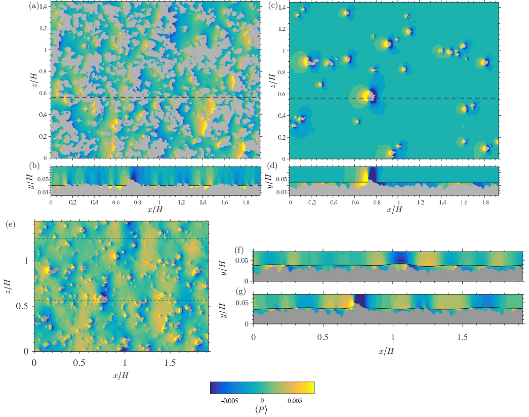
FIG. 4. Color contours of time-averaged pressure: (a)–(d) Re = 2800 , m = 0.02 (SHS), and We = 0 ; (e)–(g) Re = 2800 , We = 40 , and \bar{k}/k_{\max} = 0.75 . For We = 0 , two interface positions are shown: (a), (b) k/k_{\max} = 0.6 and (c), (d) k/k_{\max} = 0.8 . Vertical sections are shown at (b), (d) z/H = 0.56 for We = 0 , and (f), (g) z/H = 0.56 and 1.25 for We = 40 .
