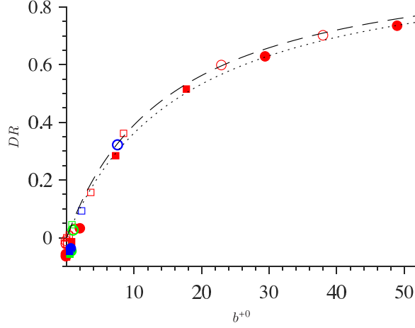
FIG. 7. Drag reduction as a function of the slip length b^{+0} in wall units: m = 0.02 (SHS, \circ ); m = 0.4 (LIS, \square ); open symbols, Re_{\tau} \approx 180 ; solid symbols, Re_{\tau} \approx 395 ; (— — —) analytic result with Re_{\tau} = 180 and (....) with Re_{\tau} = 395 from Ref. [10]; red, We = 0 ; green, We^+ \approx 10^{-2} ; and blue, We^+ \approx 10^{-3} .
