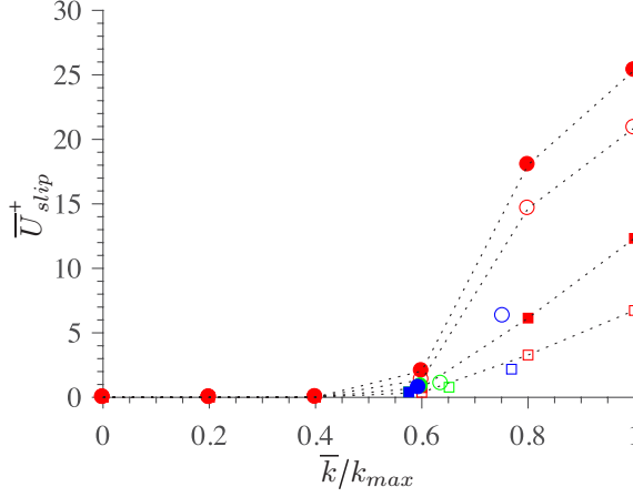
FIG. 3. Slip velocity in wall units as a function of the mean interface position: m = 0.02 (SHS, \circ ); m = 0.4 (LIS, \square ); open symbols, \text{Re}_\tau \approx 180 ; solid symbols, \text{Re}_\tau \approx 395 ; red represents \text{We} = 0 , green \text{We}^+ \approx 10^{-2} , and blue \text{We}^+ \approx 10^{-3} .
