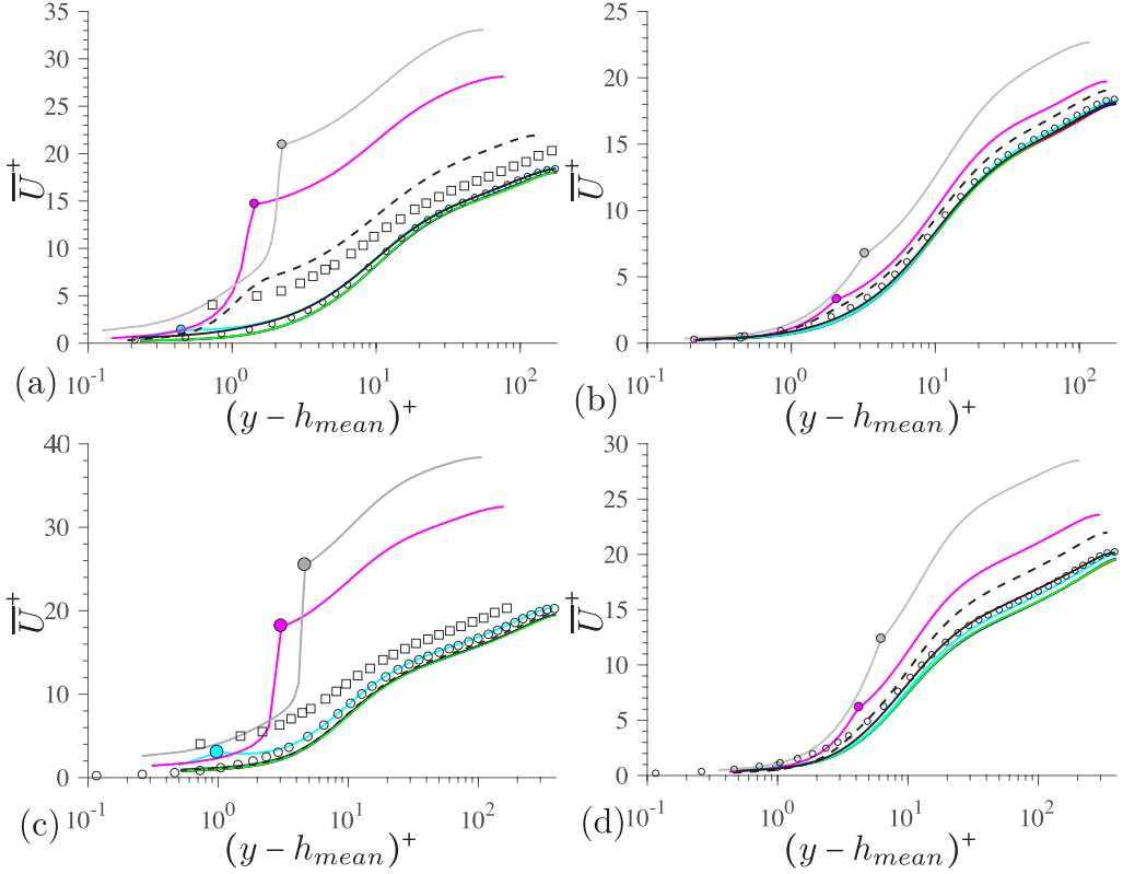
FIG. 2. Mean velocity profiles in wall units for (a), (c) m = 0.02 and (b), (d) m = 0.4 at (a), (b) Re_\tau = 180 and (c), (d) Re_\tau \approx 395 (the Re_\tau of each case is provided in Table II) for We = 0 : k/k_{\max} = 0 (—), k/k_{\max} = 0.2 (—), k/k_{\max} = 0.4 (—), k/k_{\max} = 0.6 (—), k/k_{\max} = 0.8 (—), k/k_{\max} = 1 (—); for We^+ \approx 10^{-3} : \bar{k}/k_{\max} = 0.755 (---) and for We^+ \approx 10^{-2} : \bar{k}/k_{\max} = 0.637 (—). Velocity profiles of a smooth channel flow with the corresponding Re_\tau from Moser et al. [25] ( \circ ) and over SHS etched sandblasted aluminum (SB-AL) at Re_\tau \approx 700 from Ling et al. [26] ( \square ) are included as a reference. The interface position is indicated with \bullet . For the cases k/k_{\max} < 0.6 the interface is not shown in the figure because it is below (y - h_{\text{mean}})^+ = 0.1 .
