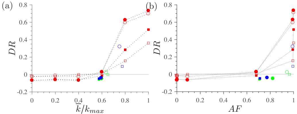
FIG. 8. Drag reduction (a) as a function of the mean interface position, \bar{k} , and (b) as a function of the area fraction: m = 0.02 (SHS, \circ ); m = 0.4 (LIS, \square ); open symbols, Re_{\tau} \approx 180 ; solid symbols, Re_{\tau} \approx 395 ; red, We = 0 ; green, We^+ \approx 10^{-2} ; and blue, We^+ \approx 10^{-3} .
