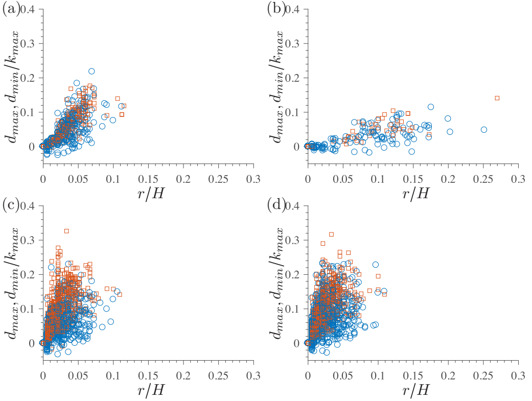
FIG. 6. Maximum and minimum time-averaged displacement with respect to the closest asperity as a function of the equivalent width of the valleys: (a), (b) Re = 2800 , (c), (d) Re = 6900 ; (a), (c) We = 400 , (b), (d) We = 40 ; \circ , m = 0.02 (SHS), and \square , m = 0.4 (LIS).
