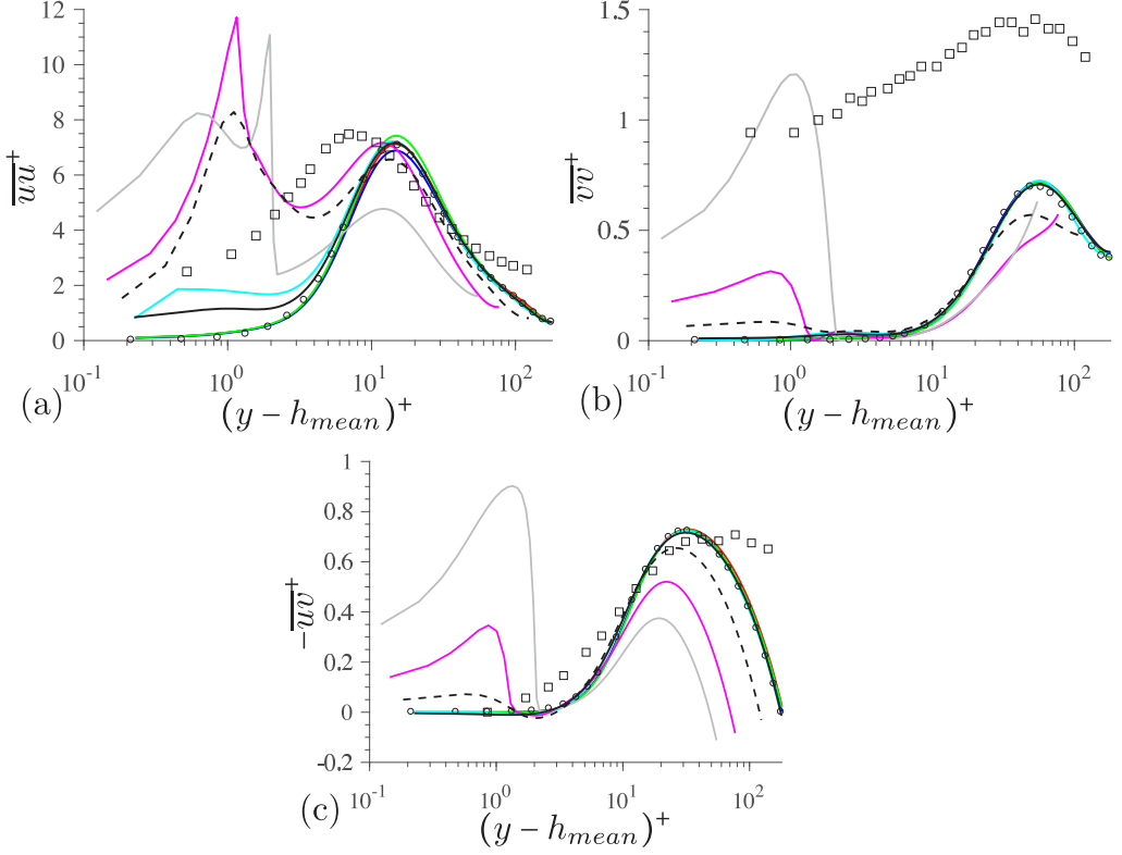
FIG. 12. (a) Variance of streamwise velocity fluctuations, (b) variance of wall-normal velocity fluctuations, and (c) Reynolds shear stress for SHS with Re_\tau \approx 180 (symbols and lines as in Fig. 2).
