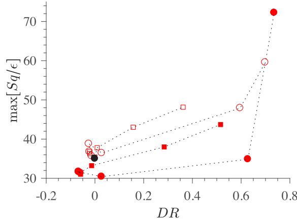
FIG. 16. Maximum of shear rate parameter Sq/\epsilon as a function of drag reduction for We = 0 : m = 0.02 (SHS, \circ ); m = 0.4 (LIS, \square ); open symbols, Re_\tau \approx 180 ; solid symbols, Re_\tau \approx 395 ; the black dot is the smooth wall.
