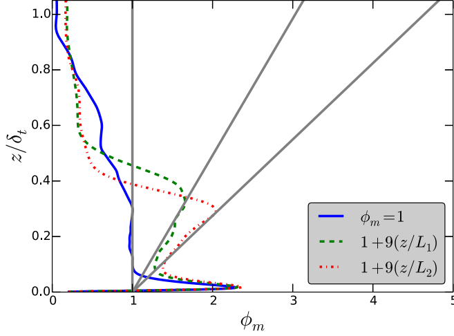
FIG. 2. Mean nondimensional velocity gradient \phi_m . Solid gray lines show the neutral boundary-layer constant nondimensional velocity gradient ( \phi_m = 1 ), and the gradients predicted by MOST, \phi_m = 1 + 9\frac{z}{L} . The colored lines are the corresponding simulated profiles, where the solid blue line is for neutral conditions, the dashed green line for Ri_b = 0.100 (with Obukhov length L_1 ), and the dot-dashed red line for Ri_b = 0.200 (with Obukhov length L_2 ).
