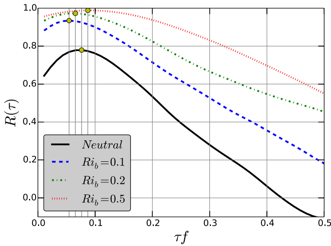
FIG. 3. Lagged correlation between TKE production and dissipation for neutral and stable cases Ri_b = 0.1, 0.2, 0.5 , versus the nondimensional time lag \tau f . Vertical lines with filled circles depict the locations of maximum correlation.
