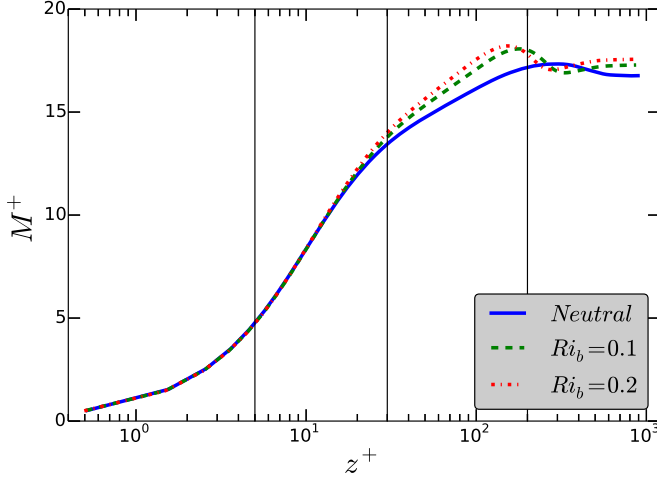
FIG. 1. Plot of mean velocity in inner coordinates, M^+ = M/u_* . Vertical black lines delimit the viscous sublayer ( z^+ \leq 5 ), buffer layer ( 5 < z^+ \leq 30 ), and logarithmic layer ( 30 < z^+ \leq 200 ) for neutrally stratified boundary layers.
