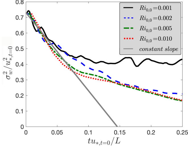
FIG. 4. Decay of the normalized vertical velocity variance with time normalized by L/u_{*,t=0} at different stabilities at z^+ \approx 50 . Note that u_{*,t=0} is the same for all cases since it is the neutral friction velocity. Linear decay as predicted by Flores and Riley [13] is shown with a solid gray line.
