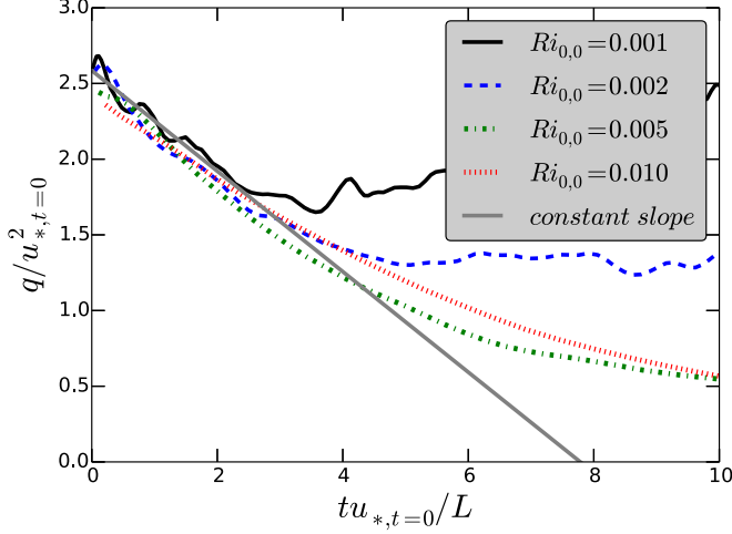
FIG. 5. Decay of normalized TKE ( q/u_{*,t=0}^2 ) with time normalized by L/u_{*,t=0} at different stabilities at z^+ \approx 50 . Note that u_{*,t=0} is the same for all cases since it is the neutral friction velocity. Linear decay rate is shown with a gray solid line.
