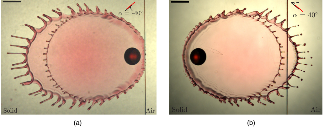
FIG. 19. (a) Formation of fingers on inclined surfaces, leading to (b) an additional droplet ejection mechanism for substrates inclined downward. The time superposition of a drop impacting at We \simeq 2115 , taken at 0, 4, and 9 ms from impact, is shown for (a) \alpha = -40^\circ and \delta \simeq 1 and (b) \alpha = 40^\circ and \delta \simeq 0.9 . The scale bar is 5 mm.
