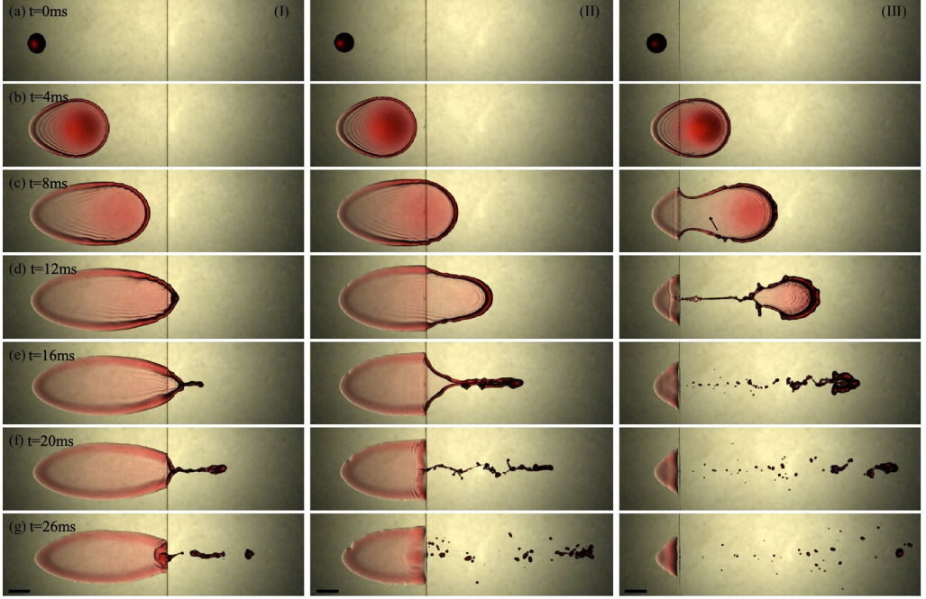
FIG. 4. Time evolution of the liquid sheet for d/R_0 = 12 , 7.3, and 1.6 (left to right). The substrate inclination is \alpha = 60^\circ and the Weber number is We \simeq 565 . Each column corresponds to an experiment illustrating a different sheet scenario (I, II, and III, from left to right). Snapshots in the same row are taken at the same time t from impact indicated in the leftmost snapshot [16]. Row (a) illustrates the position of the drops right before their impact, with respect to the edge. The scale bars are 5 mm. The arrow in (c), column, III indicates the position of a tiny air bubble trapped at early impact and then advected with the sheet.
