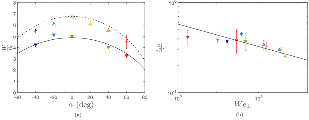
FIG. 7. (a) Semiminor axis W of the ellipse (normalized by R_0 ) obtained by fitting the envelope of the spreading liquid rim on the substrate as a function of \alpha for both We \simeq 565 ( \blacktriangledown ) and We \simeq 2115 ( \triangle ). The solid (dashed) lines correspond to Eq. (8) for We = 565 ( We = 2115 ). (b) Time t_{sM} (normalized by t_c ) at which spreading in the direction tangent to the edge reaches its maximum value W , as a function of We_{\perp} . The symbols have the same meaning as in (a), with the color representing \alpha . The solid line is Eq. (9) with c_1 = 1.5 . In both (a) and (b), error bars represent the standard deviation over all experiments at a given (We, \alpha) .
