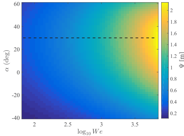
FIG. 24. Colormap of the maximum horizontal distance \Psi (in m) traveled by the ejected droplets, estimated theoretically for various We and \alpha , for an incoming raindrop of radius R_0 = 2.36 mm with \delta = 0 . The dashed line corresponds to the angle \alpha = 30^\circ that yields the maximum distance for a given We .
