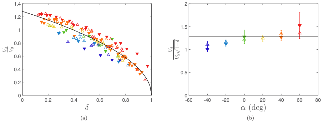
FIG. 12. (a) Normalized speed V_d of the liquid rim at sheet birth, as a function of \delta . (b) Same speed V_d , now normalized by V_0 \sqrt{1 - \delta} and then averaged over \delta . In both (a) and (b), the solid line corresponds to Eq. (16) with c = 1.28 . Symbols represent different Weber numbers We \simeq 565 ( \blacktriangledown ) and We \simeq 2115 ( \triangle ). Each symbol color corresponds to a different \alpha , as given in (b).
