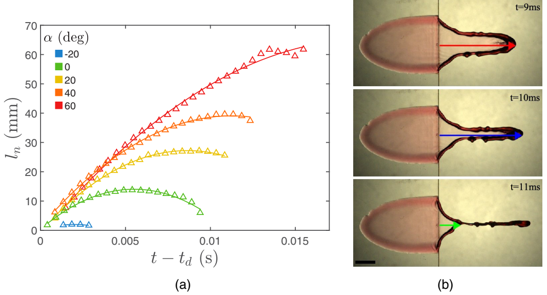
FIG. 11. (a) Extension l_n of the liquid sheet normal to the edge, as a function of the time t - t_d since the liquid reached the edge. These five experiments at We \simeq 2115 , \delta = 0.2 , and various \alpha (see the legend) correspond to the snapshots of Fig. 5. Symbols correspond to experimental measurements, while the solid lines are the approximations by Eq. (15). (b) Snapshots of a collapse of the sheet in the direction tangent to the edge at We \simeq 565 and \alpha = 60^\circ . The normal extension l_n(t) experiences a sharp decrease. Only values of l_n(t) before such collapse are considered. The scale bar is 5 mm and the time t from impact is indicated on each snapshot.
