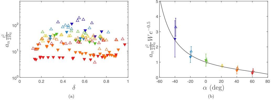
FIG. 13. (a) Normalized deceleration a_n of the rim, as a function of \delta . (b) Average of a_n t_c^2 / 2R_0 over \delta as a function of \alpha , normalized by We^{0.5} . The solid line is Eq. (18). The error bar is the standard deviation over the same population. Symbols correspond to different Weber numbers We \simeq 565 ( \blacktriangledown ) and We \simeq 2115 ( \triangle ). Each symbol color corresponds to a different \alpha , as given in (b).
