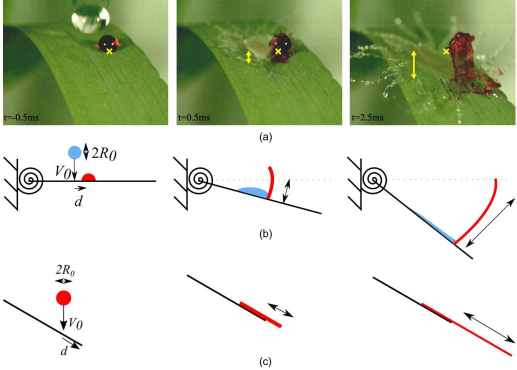
FIG. 2. (a) A clear water drop impacts on a graminea leaf on which a dyed drop has been deposited. Upon impact, the leaf deflects downward and stretches the liquid sheet. The time t from impact is indicated on each snapshot [16]. The yellow crosses and the double arrow indicate the original position of the leaf and the deflection from impact, respectively. (b) Schematic of the stretching of the crescent-moon liquid sheet due to the deflection of a leaf. The sheet is formed by the impact of a drop of radius R_0 and speed V_0 at a distance d from another sessile drop. (c) Schematic of the stretching of the liquid sheet following the impact of a single drop of radius R_0 and speed V_0 on an inclined substrate, at a distance d from its edge.
