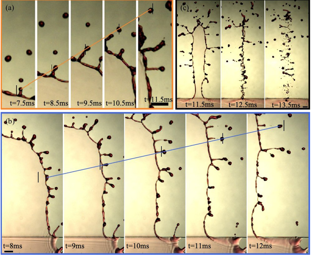
FIG. 18. Mechanisms of droplet ejection, illustrated for \alpha = 40^\circ , \delta = 0.5 , and We \simeq 2115 . (a) Radial ejection from the rim. The ejection direction of the highlighted droplet is \theta_v \simeq 6^\circ , which is here perpendicular to the rim. (b) Tangential ejection from the rim. The ejection direction of the highlighted droplet is \theta_v \simeq 15^\circ , which is here much more aligned with the rim. (c) Ejections during the collapse of the sheet. In (a)–(c) the scale bars are 2 mm and the time t from impact is indicated on each snapshot. The orange and blue solid lines join the center of mass of the ejected droplets across frames. The vertical black lines are at fixed position, so they help visualize the left-to-right motion of the droplets.
