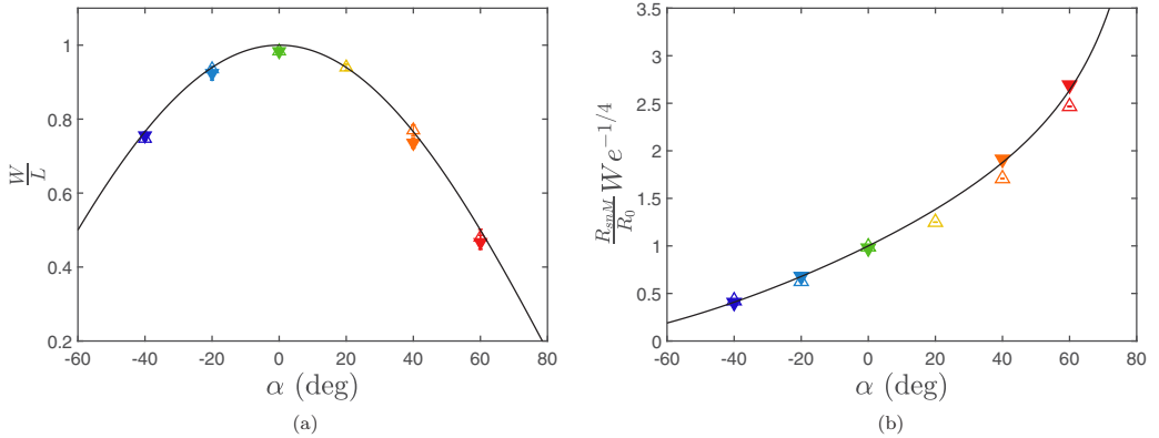
FIG. 9. (a) Aspect ratio W/L of the ellipse made by the spreading envelope and (b) maximal spreading distance R_{snM} in the direction normal to the edge, both as functions of \alpha , for We \simeq 565 ( \blacktriangledown ) and We \simeq 2115 ( \triangle ). The solid lines in (a) and (b) are Eqs. (11) and (12), respectively.
