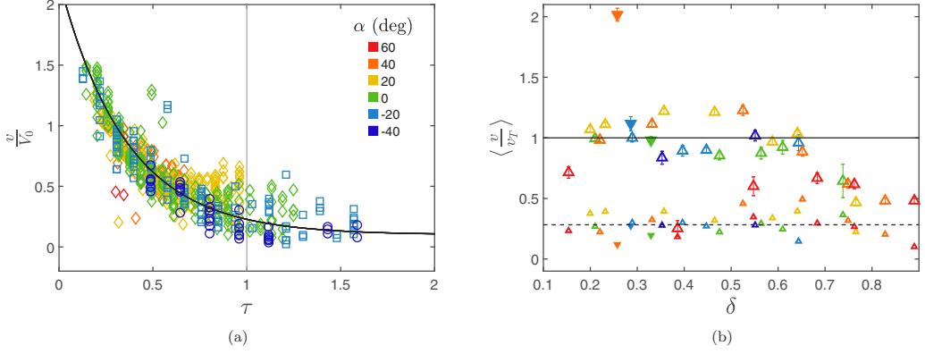
FIG. 20. (a) Droplet ejection speed v , normalized by the speed V_0 of the impacting drop, as a function of the normalized time \tau < \tau_r . Each data point corresponds to a single ejected droplet, issued from six experiments (one per \alpha ; see the legend for color definitions) at We \simeq 2115 and \delta \in [0.1, 0.3] . The vertical gray line indicates the time of maximum sheet extension normal to the edge. The solid curve represents Eq. (28). Sheet scenarios I, II, and III are represented by circles, squares, and diamonds, respectively. (b) Average (large symbols) and standard deviation (small symbols) of v/v_T over the sheet expansion, i.e., \tau < \min(1, \tau_r) , as a function of \delta for We \simeq 565 ( \blacktriangledown ) and We \simeq 2115 ( \triangle ) and various \alpha [colors as defined in legend of (a)]. The solid line is v = v_T , according to Eq. (28). The dashed line is the average of the standard deviations (small symbols) over all We , \alpha , and \delta .
