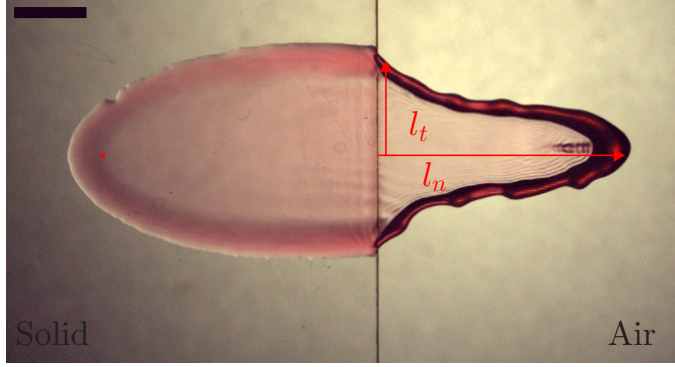
FIG. 10. Main variables l_t and l_n that characterize the liquid sheet kinematics in directions tangent and normal to the edge, respectively. The scale bar is 5 mm and the snapshot is taken at 14.5 ms after impact, at We \simeq 565 and \alpha = 60^\circ .
