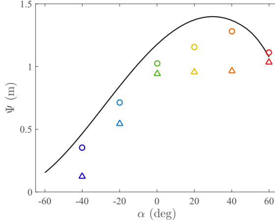
FIG. 23. Maximum distance traveled by the droplets ejected at We \simeq 2115 , for various \alpha , and all \delta pooled together. Circles represent the quantile 99% of the distance traveled by droplets ejected at \tau < \tau_r . Triangles represent the quantile 99% of the distance traveled by droplets ejected at \tau > \tau_r . The solid line is the theoretical prediction corresponding to Fig. 24.
