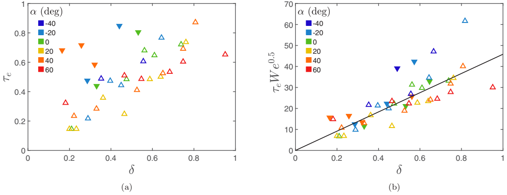
FIG. 21. (a) and (b) Normalized time \tau_e of first ejection along the rim as a function of \delta , for We \simeq 565 ( \blacktriangledown ) and We \simeq 2115 ( \triangle ) and for various \alpha (color defined in legend). In (b) the time is further multiplied by We^{0.5} . The black solid line corresponds to Eq. (29).
