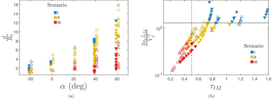
FIG. 16. Scenarios of the liquid sheet (illustrated in Fig. 4): (a) in a diagram (\alpha, d/R_0) and (b) in a diagram representing the competition of the timescale \tau_{tM} and length scale 2a_n l_{tM}/V_d^2 . Closed symbols (open symbols) correspond to We \simeq 565 ( We \simeq 2115 ), while color indicates the scenario (see the legend). In (b) the horizontal solid line is in 2a_n l_{tM}/V_d^2 = 1.3 . The vertical dashed line is in \tau_{tM} = 0.5 .
