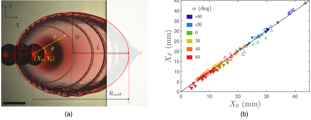
FIG. 6. (a) Time superposition of the spreading following an impact at coordinates (X_0, Y_0) on an inclined substrate ( \alpha = 40^\circ , We \simeq 565 , and d/R_0 \simeq 7.0 ). The spreading envelope is approximated by an ellipse of minor axis W and major axis L , with one of the foci in (X_F, Y_F) . Polar coordinates (\varrho, \theta) are centered on the impact point. The scale bar is 5 mm. (b) Parity plot showing that X_F and X_0 are almost identical for both We \simeq 565 ( \blacktriangledown ) and We \simeq 2115 ( \triangle ) and for \alpha \in [-40^\circ, 60^\circ] (colors defined in the legend).
