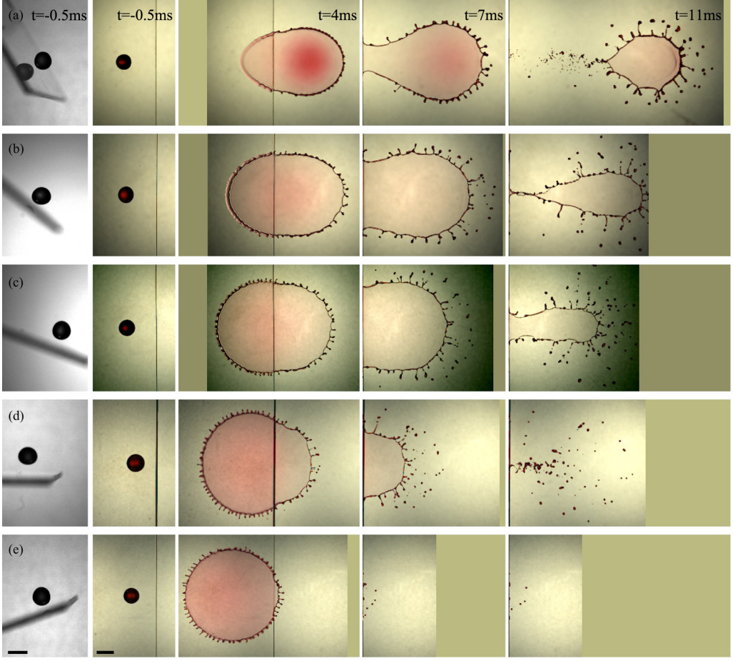
FIG. 5. Time evolution of the sheet for inclination (a) \alpha = 60^\circ , (b) 40^\circ , (c) 20^\circ , (d) 0^\circ , and (e) -20^\circ with similar d/R_0 \in [2, 3.6] and We \simeq 2115 . Scenario III is observed in rows (a)–(c), while scenarios II and I are observed in rows (d) and (e), respectively. Snapshots in the same column are taken at the same time t from impact indicated in the top row [16]. The scale bars are 5 mm.
