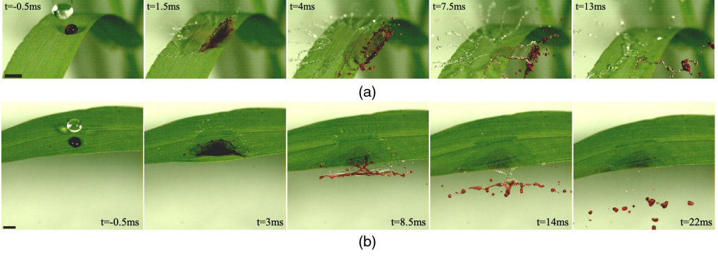
FIG. 1. (a) Crescent-moon impact where a raindrop impacts next to and pushes a sessile drop of dyed water, which is then stretched in a liquid sheet and finally fragmented in droplets. The red dye represents potential pathogens that would be present in the contaminated liquid residue on the leaf. (b) Crescent-moon impact where the dyed contaminated liquid sheet reaches the edge of the leaf. In both (a) and (b) the scale bar is 4 mm and the time t from impact is indicated on each snapshot [16].
