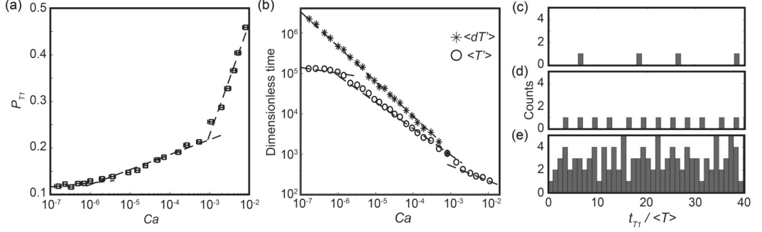
FIG. 4. (a) Scaled T1 event count P_{T1} as a function of Ca . (b) Time between two successive T1 events dT' as a function of Ca in a logarithmic scale. The results of \langle T' \rangle in Fig. 3(b) are also shown for a direct comparison. The dashed line shows a fit to the dT' data. It has a logarithmic slope of -0.86 . (c)–(e) Distribution of event onset time t_{T1} normalized by \langle T' \rangle at (c) \langle Ca \rangle = 2.5 \times 10^{-7} , (d) \langle Ca \rangle = 2.4 \times 10^{-5} , and (e) \langle Ca \rangle = 1.4 \times 10^{-3} , respectively.
