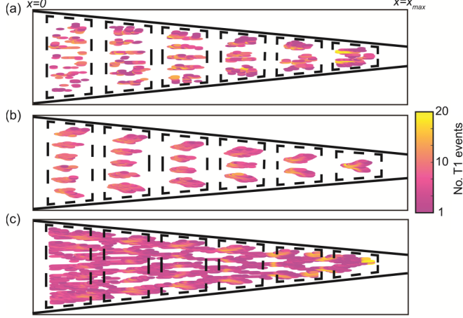
FIG. 5. (a)–(c) Spatial distribution of T1 events for Ca ranges of (a) 1.1 \times 10^{-7} < \text{Ca} < 1.6 \times 10^{-6} (within regime 1), (b) 8.5 \times 10^{-6} < \text{Ca} < 6.3 \times 10^{-5} (within regime 2), and (c) 7.9 \times 10^{-4} < \text{Ca} < 8.5 \times 10^{-3} (within regime 3), respectively. The Ca range is measured from the left edge ( x = 0 ) to the right edge ( x = x_{\max} ) of the channel. To obtain the spatial distribution, we generated 10 \times 10 \mu\text{m} mesh grids in the field of view and counted the number of T1 events that occurred within each grid. The location of each marker represents the center of a grid. The color of the markers represents the number of T1 events that occurred in the corresponding grid. The white space between the markers has no recorded T1 events. Each plot was generated by tracking a total of 2000 drops advected through the field of view. The dashed box marks the boundaries of the control volume (CV).
