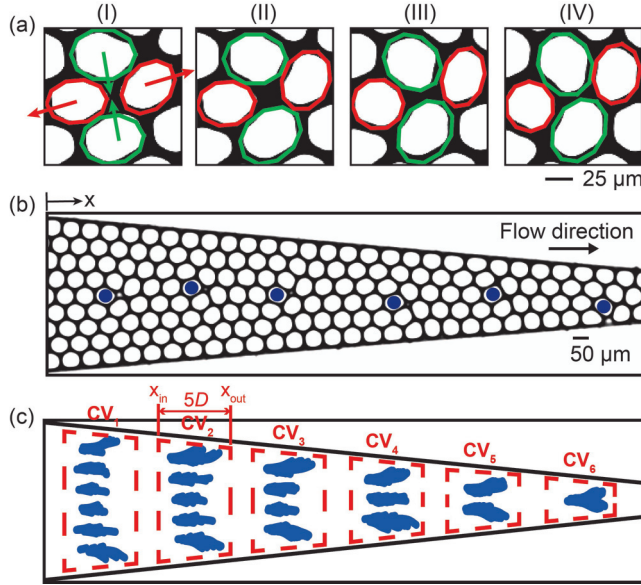
FIG. 1. (a) Progression of a T1 event. The green circles highlight a converging pair of droplets. The red circles highlight a diverging pair. The time interval between two snapshots is 0.05 s. (b) Microscopic image of the emulsion flowing in the tapered microchannel. x = 0 is set as the left boundary of the field of view shown. The blue dot represents the center of the five-edge Voronoi cell, which approximates the location of a T1 event. (c) Definition of control volume (CV). The blue markers (overlaid on top of each other) represent the locations of T1 events after 2000 drops advected through the field of view. Each red dashed box highlights a CV that has a width of 5 droplet diameters.
