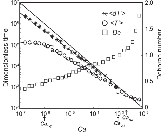
FIG. 7. dT' , T' , and De as a function of Ca . Ca_{1-2} , Ca_{2-3} , and Ca_{S-L} represent the transition between regimes 1 and 2, the transition between regimes 2 and 3, and the solidlike to liquidlike transition when De = 1 , respectively.
