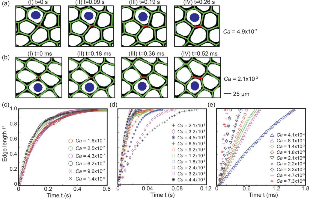
FIG. 2. (a),(b) Voronoi tessellation during a T1 event at (a) Ca = 4.9 \times 10^{-7} and (b) Ca = 2.1 \times 10^{-3} , respectively. The green lines represent the Voronoi cell edges. The red line segment represents the growing edge shared by a pair of converging drops during the T1 events. The blue dots represent the centers of five-edged Voronoi cells. (c)–(e) Length of the growing edges as a function of time for (c) 10^{-7} < Ca < 10^{-6} , (d) 10^{-6} < Ca < 10^{-3} , and (e) 10^{-3} < Ca < 10^{-2} . Each set of symbols represents the measurement of one T1 event at a given Ca .
