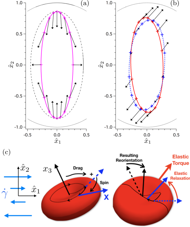
FIG. 4. Example of closed orbits (followed in the clockwise direction) for a fluid ellipsoid in shear flow ( a_1 = a_2 = 4.2375 \mu\text{m} , a_3 = 1.2511 \mu\text{m} , C = 0.01 , \lambda = 5 ), projected in the shear plane. The circle of radius 1 is shown in dotted lines. (a) Cases Ca = 0 (i.e., solid ellipsoid, black dashed line) and Ca = +\infty (i.e., fluid ellipsoid without membrane elasticity, solid magenta line). Vectors \dot{\omega}_{\text{Visc. Circ.}} are displayed at 16 evenly spaced instants over the period. (b) Case Ca = 0.013 : trajectory of (e_3)_{\hat{R}} (solid red line) and (\xi)_{\hat{R}} (blue dashed line). Vectors \dot{\omega}_{\text{Elast.}} are displayed. (c) Schematic of the drift due to the elastic torque.
