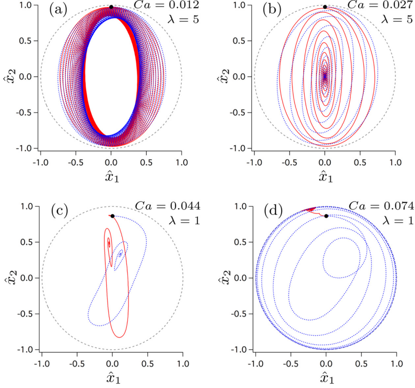
FIG. 3. Dynamics of a fluid ellipsoid ( a_1 = a_2 = 4.2375 \mu\text{m} , a_3 = 1.2511 \mu\text{m} , C = 0.01 ), in shear flow shown by the trajectories projected in the shear plane of (e_3)_{\hat{R}} (solid red line) and (\xi)_{\hat{R}} (blue dotted line). The circle of radius 1 is also shown; black dots mark the initial orientation. Dynamics (see movies in the Supplemental Material [22]) for different values of \lambda and Ca : flipping with (a) orbit selection, (b) rolling, (c) frisbee, and (d) transient kayaking and swinging.
