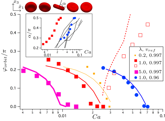
FIG. 2. Orbital drift of a RBC with Ca in shear flow varying \lambda and membrane energy barrier. Comparison of \varphi_{orbit} from simulations (solid symbols) and low-order model (solid lines). The energy barrier is modified in the simulations by changing v_{ref} (0.997 and 0.96) and adjusted in the model [Eq. (3)] by changing C (0.006 25 and 0.0175, respectively) based on the data at \lambda = 5 and \lambda = 1 , respectively. Frisbee angles are also displayed for v_{ref} = 0.997 and \lambda = 1 (open symbols for simulations and dashed line for the model). Inset: angle \alpha between the flow axis and the small axis when the RBC is on the edge while flipping; experiments for different RBCs in phosphate-buffered saline-dextran solutions with a dextran molecular weight of 10^5 g/mol (solid lines) [5] and simulations at \lambda = 1 (symbols).
