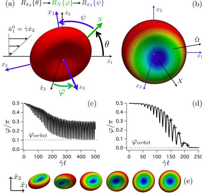
FIG. 1. Geometry and variables of interest (a), (b) and examples of dynamics in shear flow (c)–(e). (a) The orientation of the body frame ( \hat{x}_i ) with respect to the fixed frame ( \hat{x}_i ) is defined by the Euler angles [22]. (b) The membrane tank-treading is defined in the body frame by the tank-treading rate vector \dot{\Omega} and the small axis of the reference shape X . The RBC is colored by the reference shape radius (radial distance to the cell center), from blue (low values, small axis) to red (large values, long axes). (c) Simulation of an orbit selection ( \lambda = 1 , \text{Ca} = 0.016 , v_{\text{ref}} = 0.997 ): \varphi along time. The minimum angle in the stationary state \varphi_{\text{orbit}} characterizes the limit orbit. (d), (e) Simulation from flipping to rolling ( \lambda = 1 , \text{Ca} = 0.025 , v_{\text{ref}} = 0.997 ): \varphi along time (d) and corresponding sequence (e) of the simulated RBC colored as in (b). The + in (d) mark the instants when the shapes are displayed in (e).
