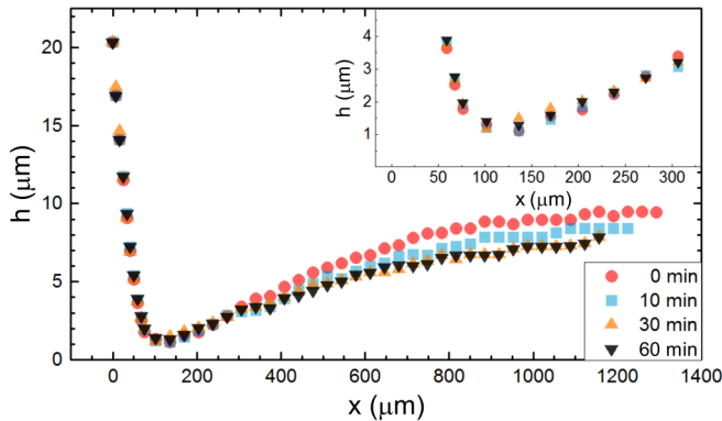
FIG. 4. Silicone oil meniscus \eta = 50 mPa s at rest in the flow cell. When stopping movement of the meniscus, the local minimum film height h_{\text{min}} in front of the meniscus and the concave curvature remained constant over the follow-up period of 60 min. Inset: magnification of the film profile at h_{\text{min}} . The gradual decrement of the film height can be associated with the capillary suction of the liquid in the meniscus of the oil plug and in the menisci at the walls of the flow cell.
