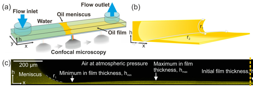
FIG. 2. Silicone oil meniscus advancing over the pre-existing silicone oil film in the flow cell. (a) Schematic illustration of the flow cell (length, x = 17 \text{ mm} ; width, y = 3.8 \text{ mm} ; height, h = 0.5 \text{ mm} ) setup on the confocal microscope. The oil meniscus ahead of water front is driven to the right. (b) Schematic drawing of the advancing oil meniscus and the film profile in the middle of the cell. r_1 and r_2 indicate curvature of the meniscus. (c) A confocal microscopy image compiled from individual vertical micrographs in xh plane (side-view) shows the meniscus and the film profile advancing in the flow cell at v \approx 15 \mu\text{m/s} ( h_0 \approx 11 \mu\text{m} , h_{\min} \approx 3.5 \mu\text{m} , and h_{\max} \approx 17 \mu\text{m} ). The micrograph reveals approximately 1/3 ( \sim 170 \mu\text{m} ) of the total height of the flow cell. Time resolution for the confocal microscopy was 0.85 \text{ s} .
