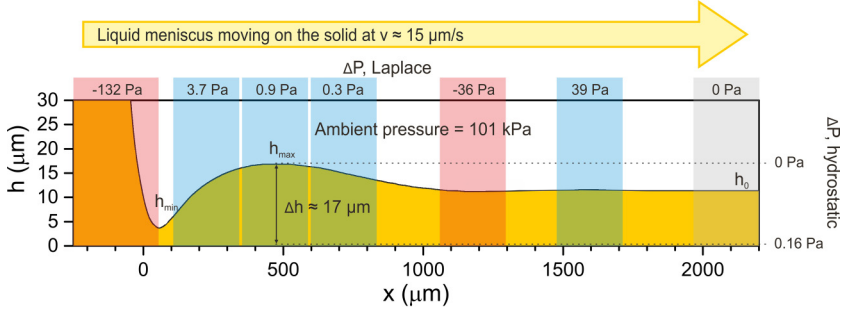
FIG. 3. Approximated Laplace and hydrostatic pressures acting at the silicone oil meniscus \eta = 50 mPa s and the curved oil film while advancing in the flow cell at v \approx 15 \mu\text{m/s} . Curvature of the oil meniscus is characterized by two negative radii (Fig. 2), vertical r_1 \approx -190 \mu\text{m} and horizontal r_2 \approx -1100 \mu\text{m} yielding approximated Laplace pressure of -132 Pa. Elsewhere in the film the effect of r_2 is considered to be negligible, thus the curvature r_1 determines the Laplace pressure at the given areas from left to right in the image as follows (calculated Laplace pressure, related curvature r_1 ): 3.7 Pa, 5700 \mu\text{m} ; 0.9 Pa, 24000 \mu\text{m} ; 0.3 Pa, 60000 \mu\text{m} ; -36 Pa, -590 \mu\text{m} ; 39 Pa, 540 \mu\text{m} . At the smooth film region, where the curvature of the oil interface is zero, the Laplace pressure is zero.
