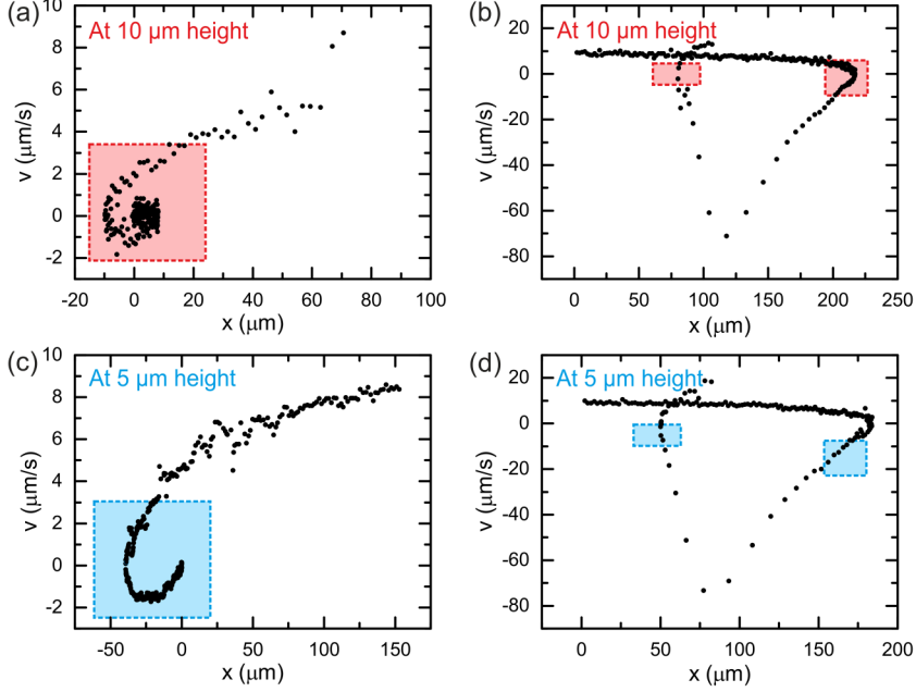
FIG. 7. Hydrodynamic flow at different heights in the silicone oil film. Oil viscosity \eta = 50 mPa s, meniscus velocity v \approx 15 \mu\text{m/s} , and initial film thickness h_0 = 11 \mu\text{m} . The coordinates of 1 \mu\text{m} polystyrene tracer microparticles in the oil film were monitored by confocal microscopy. The data was collected with the focal plane set at 10 and 5 \mu\text{m} above the glass substrate using the confocal microscope transmission channel. The data reveals two backflows in the film: (a), (c) over the secondary minimum and (b), (d) over the primary minimum in film thickness. (a), (b) Red and (c), (d) blue rectangles correspond to the data acquired at \sim 10 \pm 1 \mu\text{m} and \sim 5 \pm 1 \mu\text{m} heights in the film, respectively, using the confocal microscope fluorescent channel.
