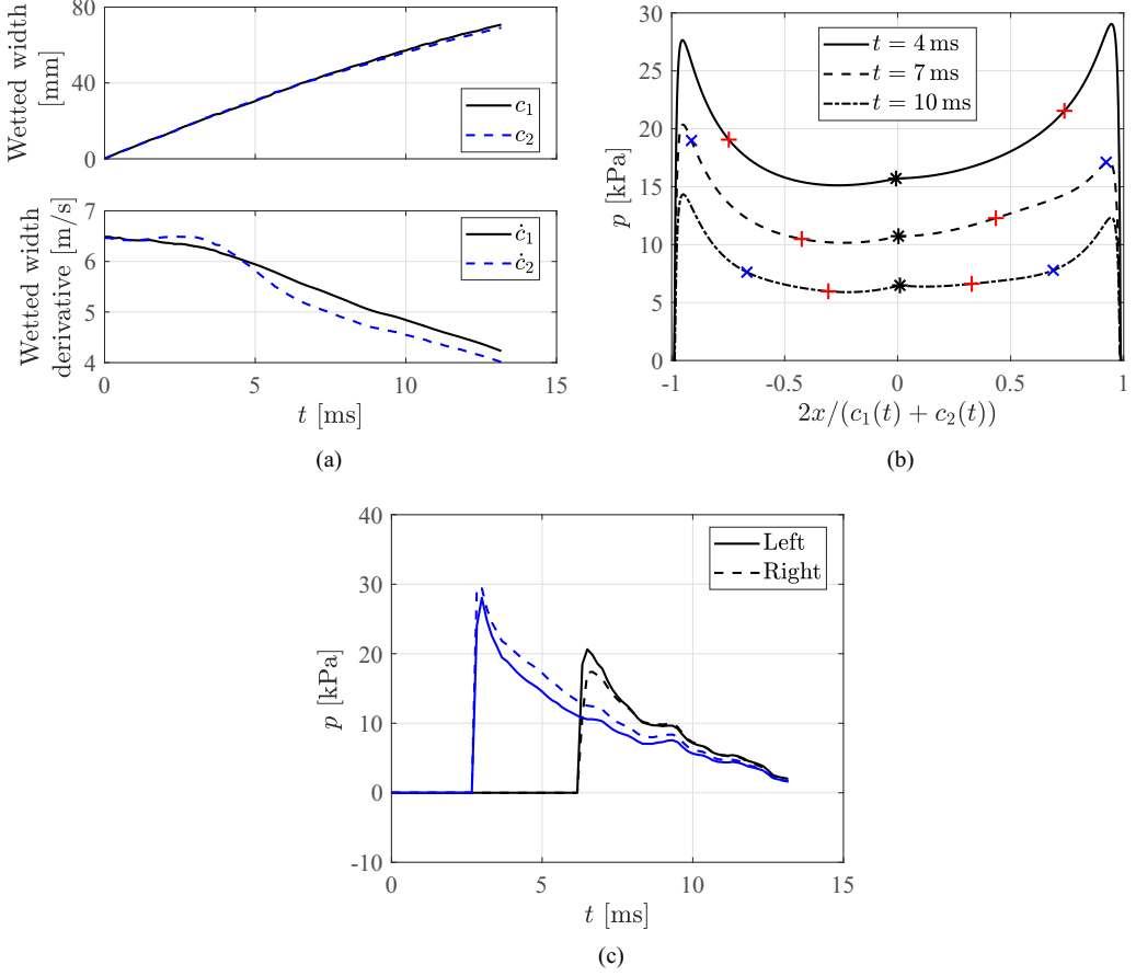
FIG. 6. (a) Time histories of the left c_1 and right c_2 wetted widths (top) and their derivatives \dot{c}_1 and \dot{c}_2 (bottom) from the MLM. (b) Pressure profile on the wedge wetted surface from the MLM; the location of the keel and the pressure sensors are highlighted by * (keel), + (sensors at L_s = 22 mm), and \times (sensors at L_s = 47 mm). (c) Pressure time histories at L_s = 22 mm (blue) and L_s = 47 mm (black) on the left- (solid line) and right- (dashed line) hand sides of the wedge from the MLM.
