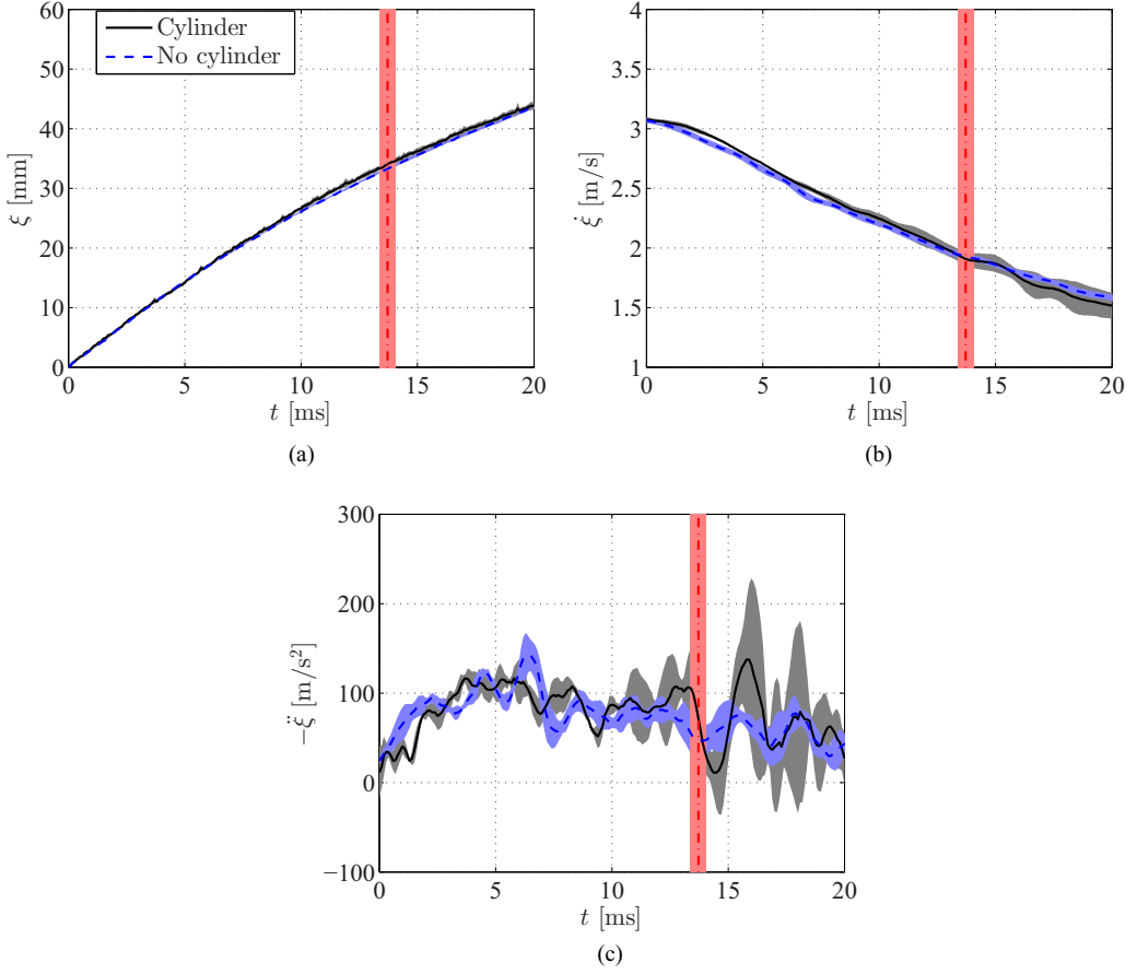
FIG. 2. (a) Entry depth \xi , (b) velocity \dot{\xi} , and (c) acceleration \ddot{\xi} of the wedge from experiments in the presence (solid black line) and in the absence (dashed blue line) of the cylinder (results reproduced from [28]) as functions of time. The time instant of the contact between the wedge and the cylinder is highlighted by a vertical red line. Results are averaged across repetitions and presented with their corresponding standard deviations.
