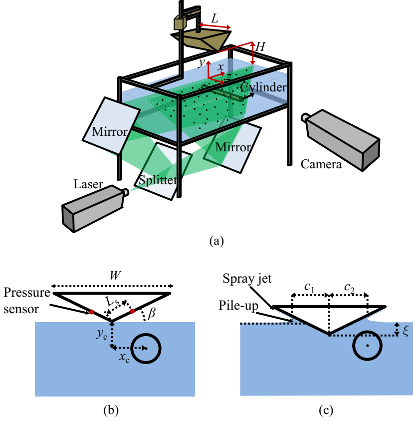
FIG. 1. Schematics of the problem and definition of significant quantities. (a) Experimental apparatus and data acquisition system. The wedge, fluid, and cylinder are shown at (b) the onset of the impact (red markers label the location of the pressure sensors) and (c) a few milliseconds into the entry.
