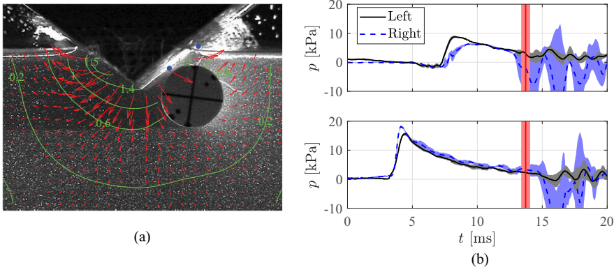
FIG. 3. (a) Particle image velocimetry images overlaid with velocity vectors and contour plot of the velocity magnitude in m/s at 7.5 ms; the blue markers identify the location of the pressure sensors on the right-hand side of the wedge. (b) Pressure time histories at the locations of the pressure sensors at L_s = 22 mm (bottom) and 47 mm (top). (Pressure measurements should be considered valid only after the sensor touches the water surface. The initial difference in the pressure readings is likely due to the combination of measurement uncertainty and variations in the installation process. Similar results were in fact noted in [28], without the presence of a cylinder.) The time instant of the contact between the wedge and the cylinder is highlighted by a vertical red line. Note that the results in (b) are averaged across the repetitions and presented with their corresponding standard deviations.
