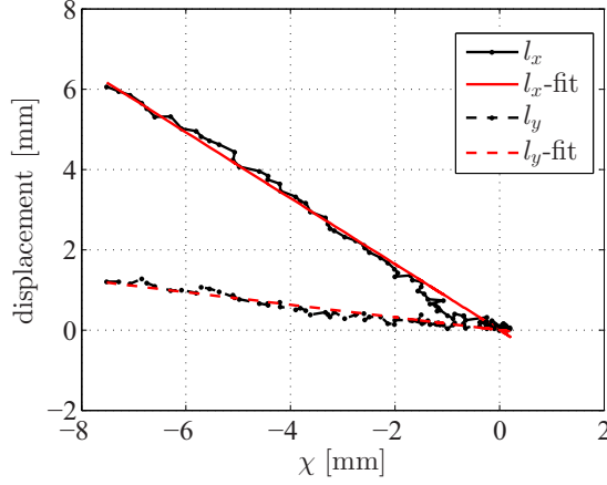
FIG. 5. Experimental results for the horizontal l_x and vertical l_y cylinder displacements versus \chi , together with their corresponding linear fits.
