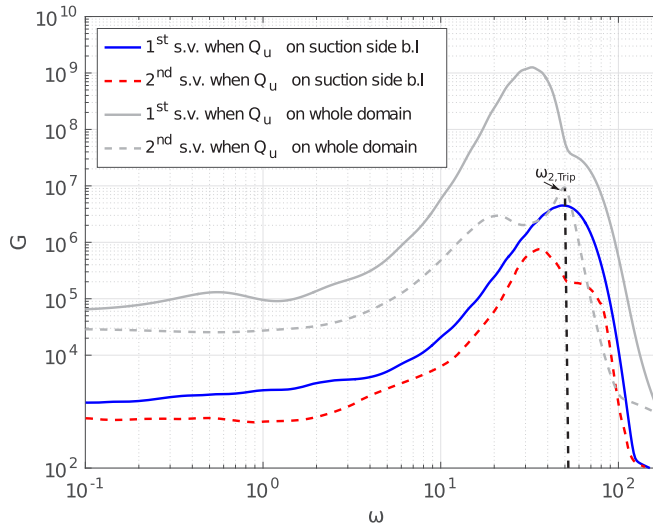
FIG. 20. Resolvent spectra with different optimization domains. The gray lines correspond to optimization over the whole domain, while the colored lines correspond to a domain on the suction side of the airfoil.
