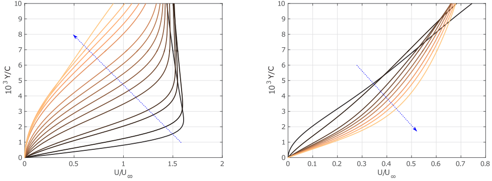
(a) Velocity profiles at x/c=0.01, 0.02, 0.05, 0.1, 0.12, 0.14, 0.16, 0.18, 0.22, 0.24, 0.26, 0.28, 0.32 . (b) Velocity profiles at x/c=0.40, 0.44, 0.48, 0.50, 0.52, 0.54, 0.56, 0.58, 0.62
