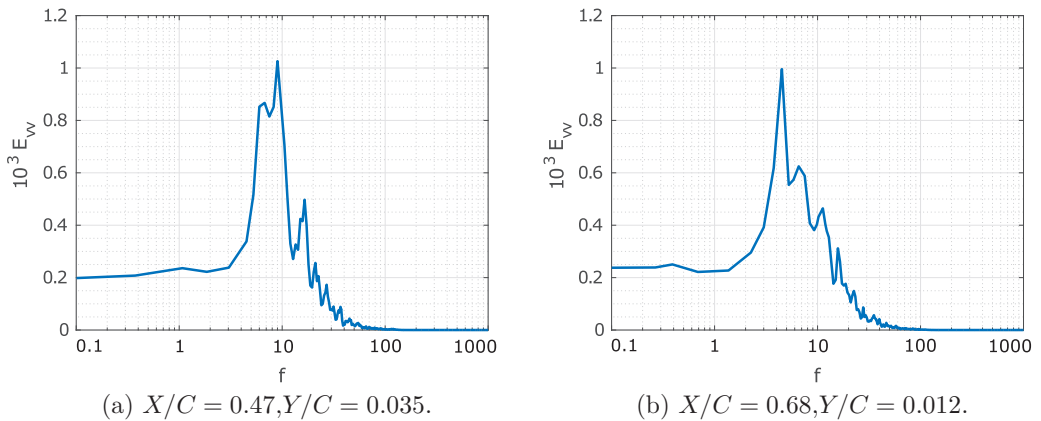
FIG. 14. Cross-stream velocity spectra at two locations on the suction' side boundary layer.
