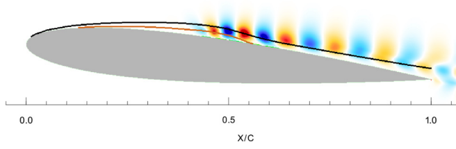
FIG. 6. Cross-stream component of the optimal response at frequency \omega_p at the suction side of the airfoil. The solid black line shows the displacement thickness of the boundary layer while the solid brown line is the zero-streamwise mean velocity contour. The contours range is [-4.17, 4.17] .
