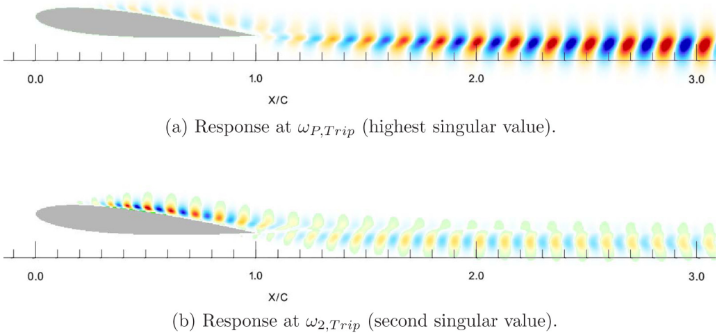
FIG. 18. Cross-stream components of responses at frequencies \omega_{P,Trip} and \omega_{2,Trip} . The contours in Fig. 18(a) range between [-3.6, 3.6] while in Fig. 18(b) [-9.8, 9.8] .
