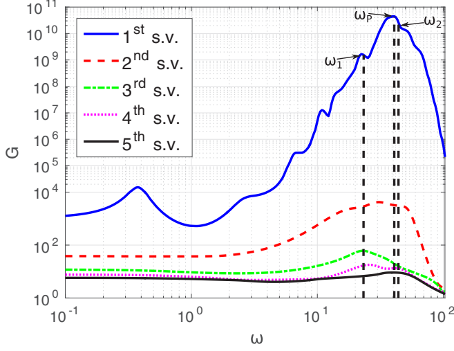
FIG. 4. Spectrum of the resolvent operator for the naturally developing flow around a NACA-0012 with straight trailing edge. The first five gain values of the operator are plotted against the angular frequency \omega .
