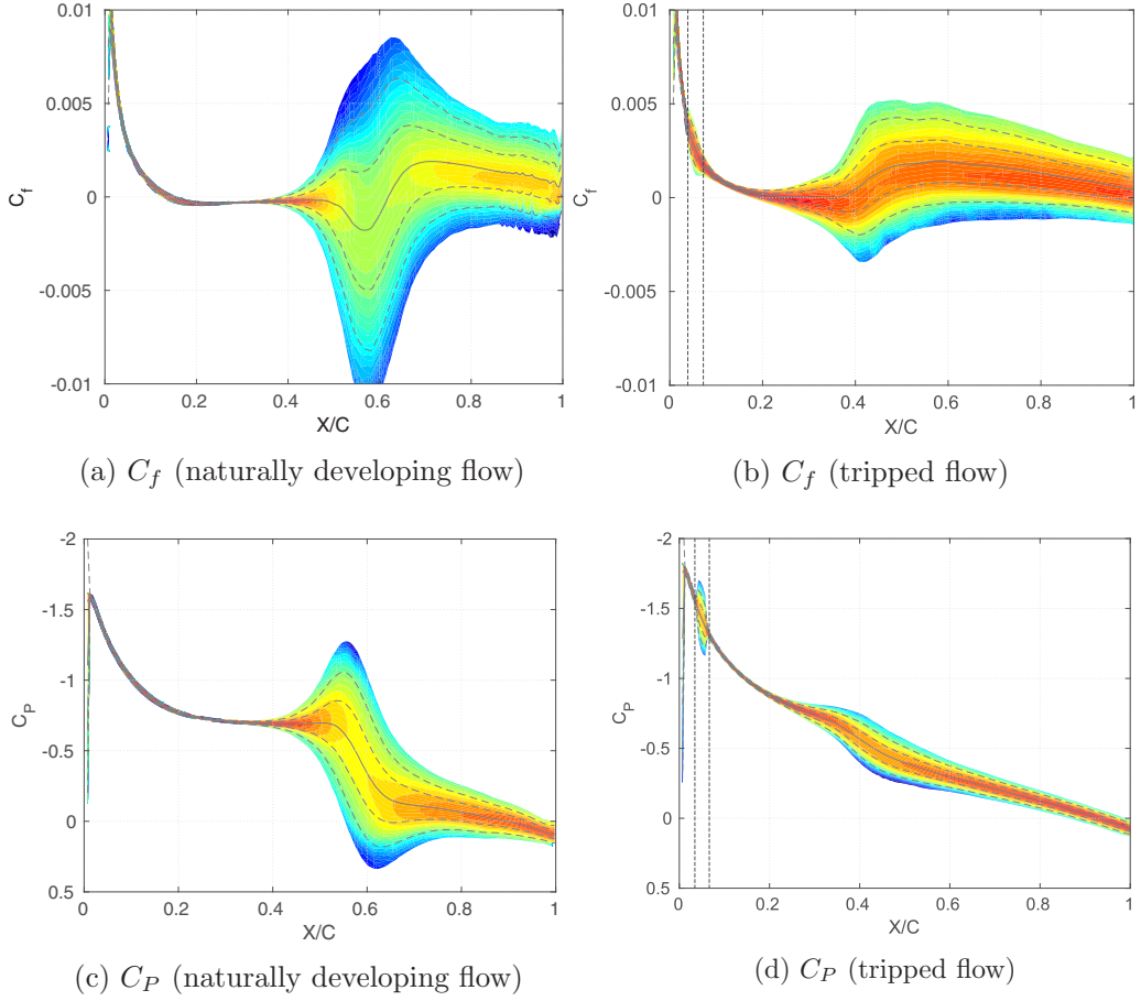
FIG. 12. Probability density function of C_f and C_P for the naturally developing (left column) and tripped (right column) flows. The solid line in each plot denotes the mean value, while the dashed lines bracket the \pm 1\sigma and \pm 2\sigma ranges around the mean. The vertical dashed lines in Figs. 12(b) and 12(d) indicate the thin strip where tripping was applied.
