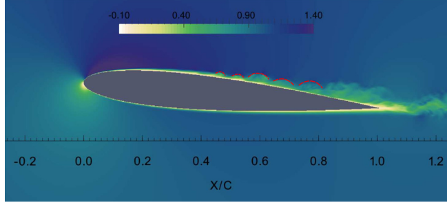
FIG. 15. Instantaneous streamwise velocity field. The red curves delineate large scale structures.
