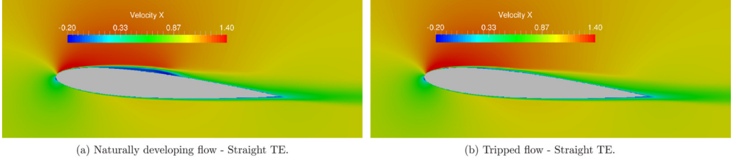
FIG. 1. Mean streamwise velocity field for the naturally developing and tripped flows around the straight trailing edge airfoil.
