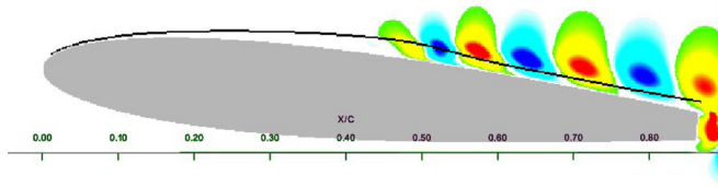
FIG. 11. Cross-stream component of the optimal response at the suction side of the airfoil at frequency \omega_{SH} . The solid black line shows the displacement thickness of the boundary layer. The contours range is [-0.8, 0.8] .
