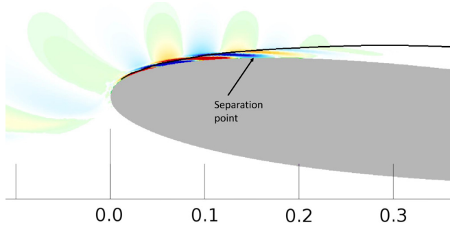
FIG. 5. Streamwise component of the optimal forcing \hat{f}_x at frequency \omega_P at the leading edge with the displacement thickness of the boundary layer superimposed. The contours range is [-72, 72] .
