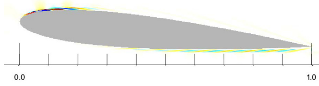
FIG. 17. Optimal forcing in the cross stream direction at frequency \omega_{P,Trip} . The contours range is [-69.2, 69.2]
