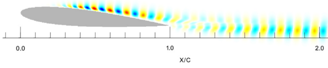
FIG. 21. Cross-stream component of the optimal response at the frequency \omega_{2,\text{Trip}} when the domain shown in Fig. 19 is used in the optimization process. The contours range is [-7.7, 7.7] .
