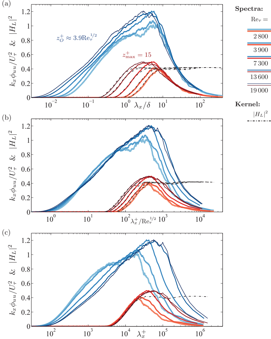
FIG. 10. Premultiplied spectra of the streamwise velocity fluctuations at an outer-region position z_O^+ \approx 3.9 Re_\tau^{1/2} for five values of Re_\tau . Alongside are the premultiplied spectra of the superposition IOIM component at z_{max}^+ = 15 , which equal the outer-region spectra multiplied by the gain squared of the kernel between z_{max}^+ = 15 and z_O^+ (indicated with the dash-dotted line). The panels sequentially employ an (a) outer, (b) log, and (c) inner scaling of the wavelength axes on the abscissae.
