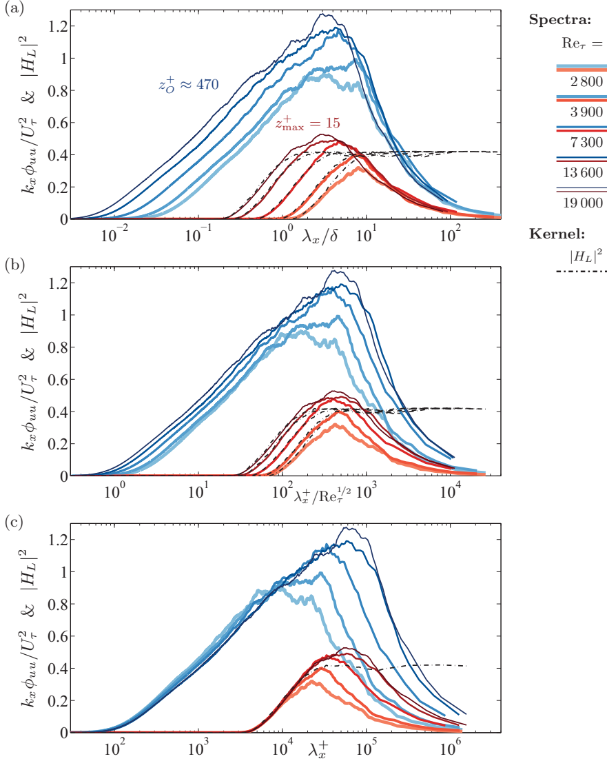
FIG. 11. Similar to Fig. 10 but now for z_O^+ \approx 470 . Note that the gain squared of the kernel, |H_L|^2 , is the same as in Fig. 10 and that this kernel was derived from a calibration experiment at Re_\tau \approx 13\,300 , for which z_O^+ \approx 3.9 Re_\tau^{1/2} \approx 470 .
