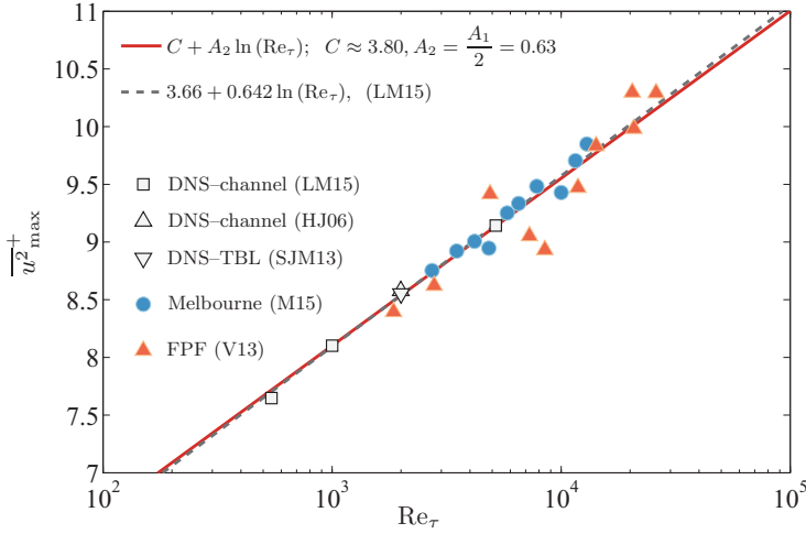
FIG. 8. Peak in the streamwise turbulence intensity, \overline{u^2}_{\max}^+ , as a function of \text{Re}_\tau . DNS data of (LM15) Lee and Moser [17] at \text{Re}_\tau \approx 550, 1000 , and 5200 (channel), (HJ06) Hoyas and Jiménez [16] at \text{Re}_\tau \approx 2000 (channel), and (SJM13) Sillero, Jiménez, and Moser [56] at \text{Re}_\tau \approx 2000 (TBL). Experimental data of (M15) Marusic et al. [78], acquired in Melbourne’s boundary layer facility, and of (V13) Vincenti et al. [81], acquired in the Flow Physics Facility (FPF).
