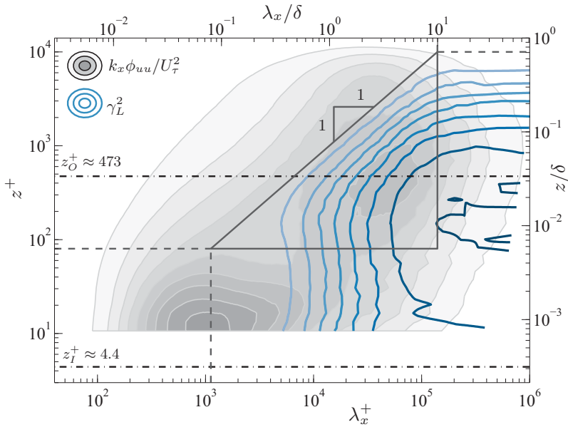
FIG. 2. Premultiplied energy spectrogram k_x \phi_{uu}/U_\tau^2 (levels: 0.2:0.2:1.8) at \text{Re}_\tau \approx 14\,000 with an overlaid coherence spectrogram \gamma_L^2(z, z_I; \lambda_x) relative to the reference location z_I^+ \approx 4.4 (levels: 0.1:0.1:0.9), following Baars et al. [1]. The hypotenuse of the triangle equates to \lambda_x/z = 14 and spans from z^+ = 80 up to z/\delta \approx 0.71 (the right-hand side is located at \lambda_x/\delta = 10 ).
