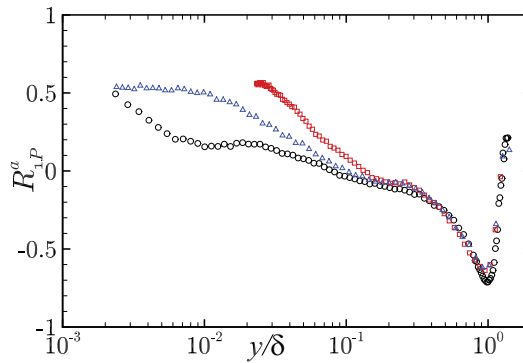
FIG. 5. The zero-time-delay AM correlation coefficient, R_{1P}^a|_{\tau=0} , as defined by Mathis et al. [15], as a function of the wall-normal position. \circ : smooth; \square : Rough (LMP); \triangle : Rough (HMP).
