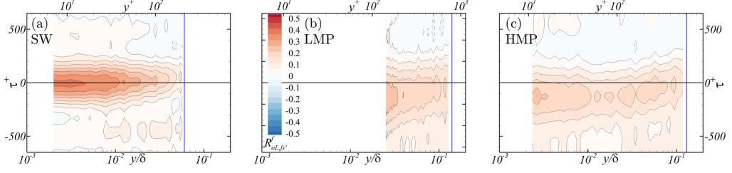
FIG. 11. Two-probe FM correlation maps, R_{2p}^f , for (a) smooth and (b, c) rough-wall flow at an LMP and a HMP, respectively. The blue lines indicate the location of the outer probe for each case.
