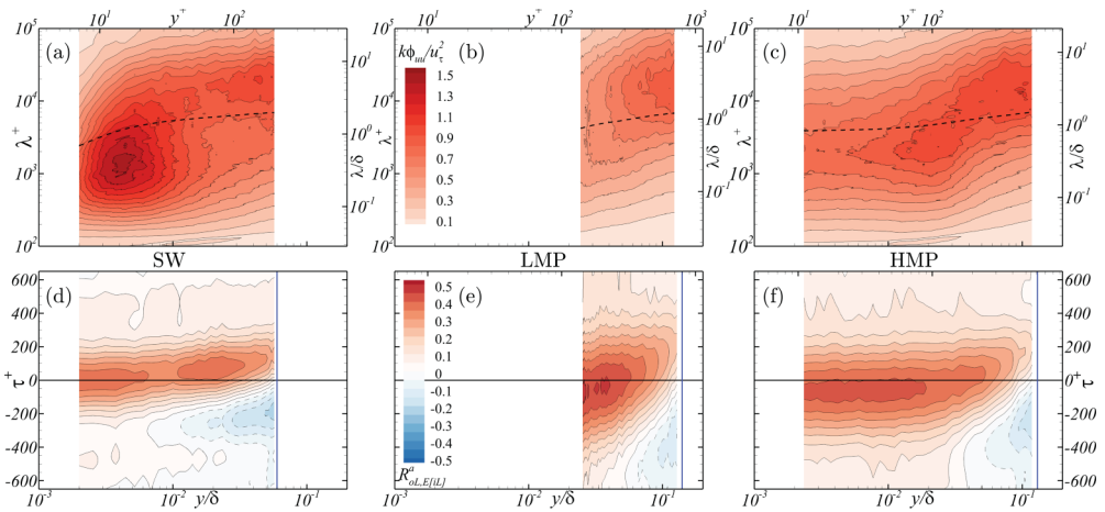
FIG. 6. (a–c) Premultiplied streamwise TKE spectrograms (dashed horizontal line corresponds to \lambda_x^+ = 7000 —the cutoff wavelength) and (d–f) two-point AM correlation coefficients, R_{2P}^a , for smooth- and rough-wall flow at an LMP and a HMP, respectively. The blue lines in (d–f) indicate the location of the outer probe for each case.
