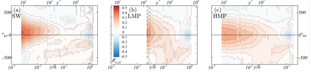
FIG. 9. One-probe FM correlation maps, R_{1P}^f , for (a) smooth and (b, c) rough-wall flow at an LMP and a HMP, respectively.
