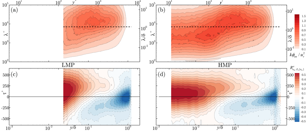
FIG. 4. (a, b) Premultiplied streamwise TKE spectrograms (dashed horizontal line corresponds to \lambda_x^+ = 7000 —the cutoff wavelength) and (c, d) single-point AM correlation coefficients, R_{1P}^a , for rough-wall flow at an LMP and a HMP, respectively.
