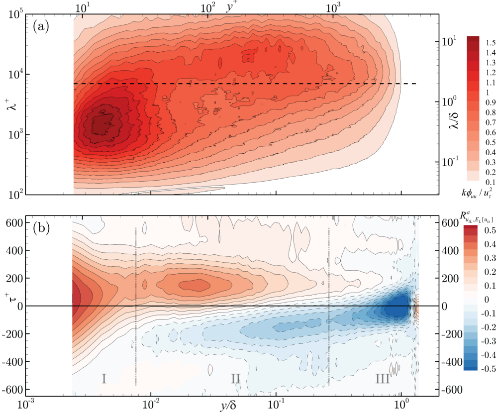
FIG. 3. (a) Premultiplied streamwise TKE spectrogram (dashed horizontal line corresponds to \lambda_x^+ = 7000 —the cutoff wavelength) and (b) single-point AM correlation coefficient, R_{1P}^a (regions I, II, and III marked in the correlation map) for smooth-wall flow.
