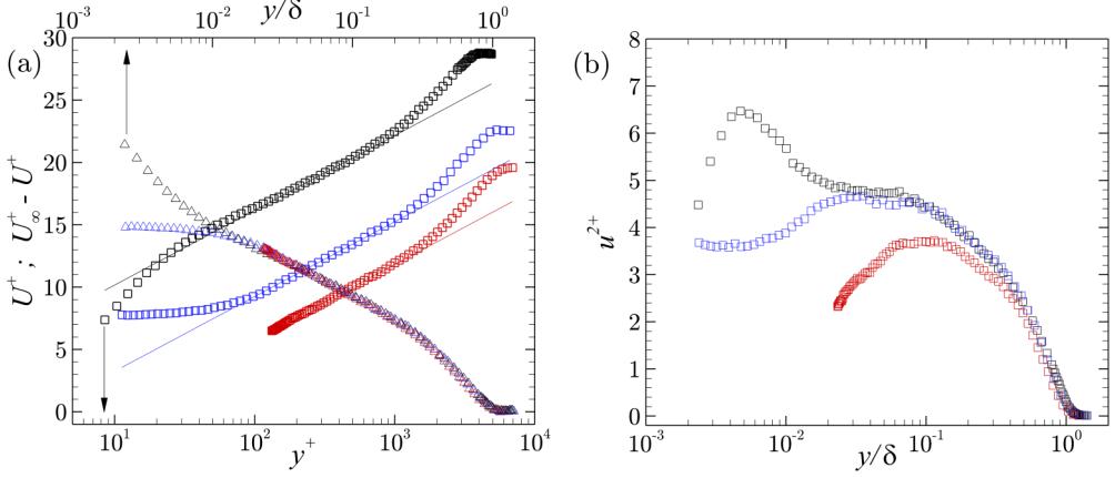
FIG. 2. (a) Profiles of mean velocity normalized in inner units (squares), and in defect form with y -normalized in outer units (triangles). Also shown are logarithmic profiles with \kappa = 0.384 . (b) Corresponding mean streamwise turbulent kinetic energy profiles. Smooth; rough (LMP); rough (HMP).
