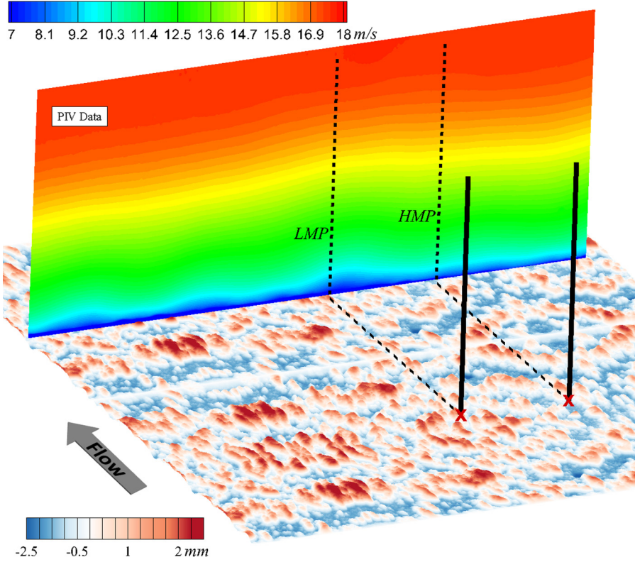
FIG. 1. A true-scale schematic of the hot-wire measurement locations relative to the complex roughness shown in perspective view. The mean streamwise velocity is presented in a cross-flow plane (measured using sPIV), highlighting the spanwise positions of the current hot-wire measurements (denoted with “X”) at an LMP (left) and HMP (right), as previously identified by Barros and Christensen [43]. The current measurement points are 150 mm upstream of the PIV plane indicated and distributed on the solid line.
