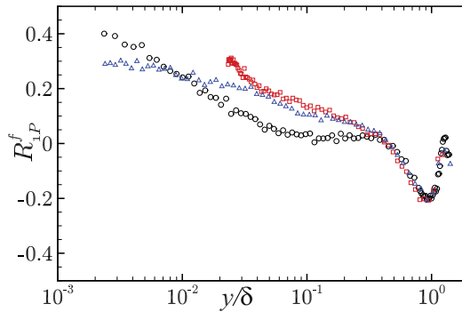
FIG. 10. The zero-time-delay FM correlation coefficient, R_{1P}^f|_{\tau=0} , as a function of the wall-normal position. \circ , smooth; \square , rough (LMP); \triangle , rough (HMP).
