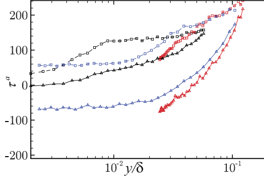
FIG. 7. Time delay for maximum AM correlation coefficient. \square : one probe; \triangle : two probe. Smooth; rough (LMP); rough (HMP).
