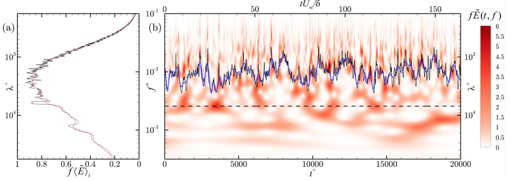
FIG. 8. Premultiplied wavelet power spectrum (WPS) ( f\tilde{E} , right) of a velocity time series measured over smooth-wall flow at y^+ = 9 . The time series on the plot mark the corresponding instantaneous frequencies, f_s and f_{sL} , and the cutoff frequency, f_c (dashed). The time average of the WPS ( f\langle\tilde{E}\rangle_t ) is compared with corresponding smoothed premultiplied power spectrum ( k\phi_{uu} ) on the left—both of which are measures of average distribution of energy among various scales.
