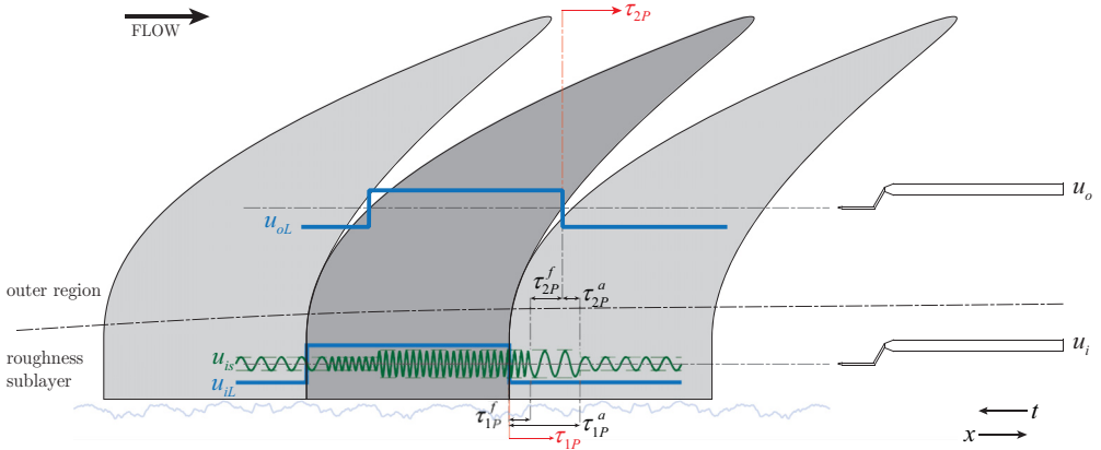
FIG. 12. A schematic representation of inner–outer interactions that was originally presented by Baars et al. [29], but modified to represent the current experiments and observations.
