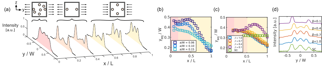
FIG. 2. Experimental particle equilibrium locations in a TFF channel. (a) One experiment showing the distribution of particles along the length of the channel ( x/L ) and (top) a corresponding schematic illustrating the influence of permeate flow direction on cross-sectional distribution of particles. At the entrance (left), the particles are dispersed and unfocused. In the outward permeate flow region, the particles are moving towards the wall, and so the equilibrium position is closer to the wall, and the out-of-plane equilibrium positions are unstable. In the inward permeate flow region, the equilibrium position shifts away from the wall, due to the fluid from the permeate channels flowing into the main channel, and the out-of-plane equilibrium positions regain stability. (b) Streamwise equilibrium positions for the three different particle sizes, all at a Reynolds number of 138 and a \beta of 1.0. (c) Experiments showing the effect of \beta at a Re of 138 and a/W of 0.15. This graph also superimposes results from a straight channel device (SC) where the equilibrium position is constant throughout the channel. (d) Particle intensity distributions at the end of the channel ( x/L = 1 ) for different \beta and a Re = 138 . Here we see that as \beta decreases the out-of-plane equilibrium point disappears because more flow is diverted towards the wall, even at the end of the channel.
