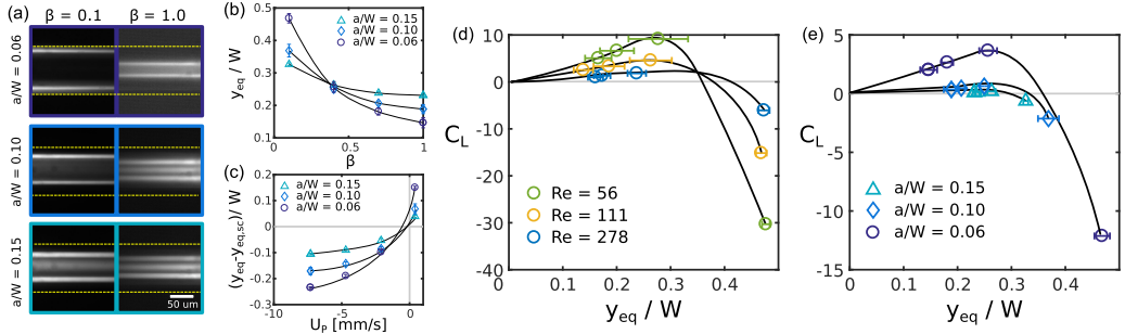
FIG. 4. (a) Gray-scale streaklines of the particle focusing with three different channel sizes and two values of \beta . (b) Endpoint equilibrium locations vs \beta for three different particle sizes ( Q_F = 50 ml/h at x/L = 1 ). (c) The difference between measured equilibrium locations for a TFF channel and straight channel (SC) as a function of the local permeate velocity ( U_P ) at the wall for Q_F = 50 ml/h at x/L = 1 . The presence of a transverse permeate flow causes inertially focused particles to deviate from their SC equilibrium location. Smaller particles are more susceptible to permeate flow as characterized by larger deviations from the SC equilibrium for a given permeate flow. The location of the TFF equilibrium returns to that of the SC in the absence of permeate flow. Measured values of the lift coefficient ( C_L ) on particles flowing in a TFF channel for various (d) Re = 56, 11 , and 278 a/W = 0.06 and (e) particle sizes a = 5.6, 10 , and 15 \mu\text{m} ( Re = 138 ).
