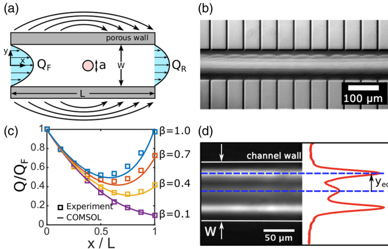
FIG. 1. (a) Schematic of TFF device with recirculating flow. (b) Image of the primary channel and several perpendicular permeate channels within a microfabricated TFF device (global view of the device can be seen in Ref. [21]). (c) Nondimensional flow rates versus channel length for varying \beta ( \beta = Q_R/Q_F = outflow and inflow). In each case, there is good agreement between COMSOL models and data. (d) (left) Long exposure image of 10\ \mu\text{m} fluorescent polystyrene particles in a 100 \times 100\ \mu\text{m} TFF channel flowing at Re = 83 . The in-plane particles equilibrate at a distance ( y_{eq} ) relative to the centerline. (right) Intensity distribution of the same image showing the intensity peaks used to determine ( y_{eq} ). Note that there are three peaks, the two larger peaks correspond to the equilibrium location of particles in-plane, and the smaller peak is attributed to the out-of-plane equilibrium location of the flowing particles.
