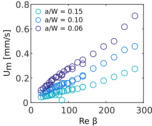
FIG. 3. Transverse migration velocities plotted against Re\beta . The linear results indicate that the migration is largely dominated by viscous forces; however, inertial aspects are apparently important since there is a dependence on particle size (i.e., data do not collapse).
