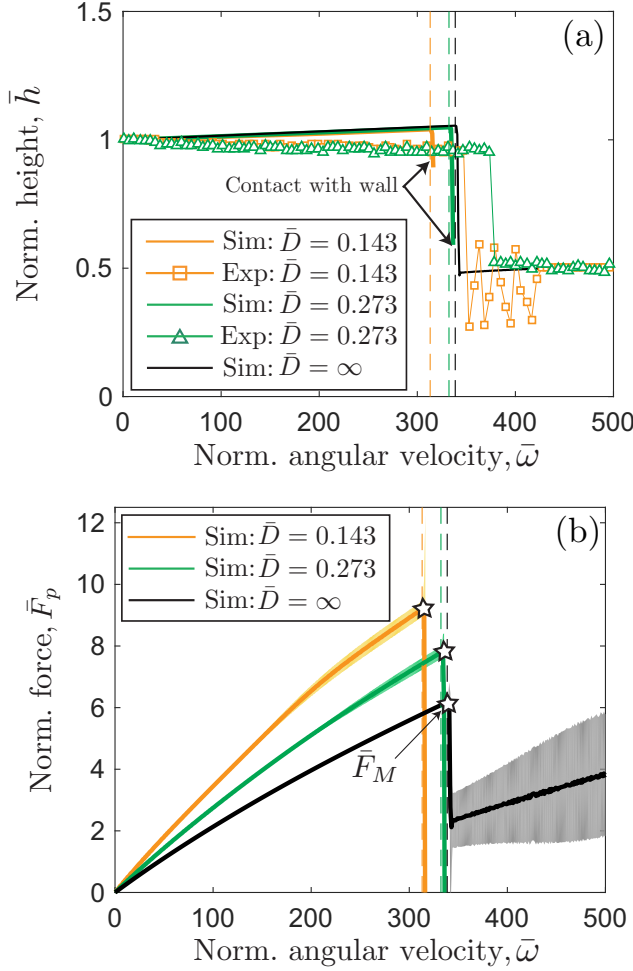
FIG. 5. (a) Steady-state values of the normalized suspended height, \bar{h} , as a function of normalized angular velocity \bar{\omega} , at three different values of the boundary distance, \bar{D} = \{0.143, 0.273, \infty\} , from experiments and simulations (see legend). The normalized buckling velocity, \bar{\omega}_b , from the simulations is represented by the vertical dashed lines. (b) Normalized propulsive force, \bar{F}_p , as a function of \bar{\omega} obtained from the numerical simulations. The shaded region corresponds to the standard deviation of the force signal.
