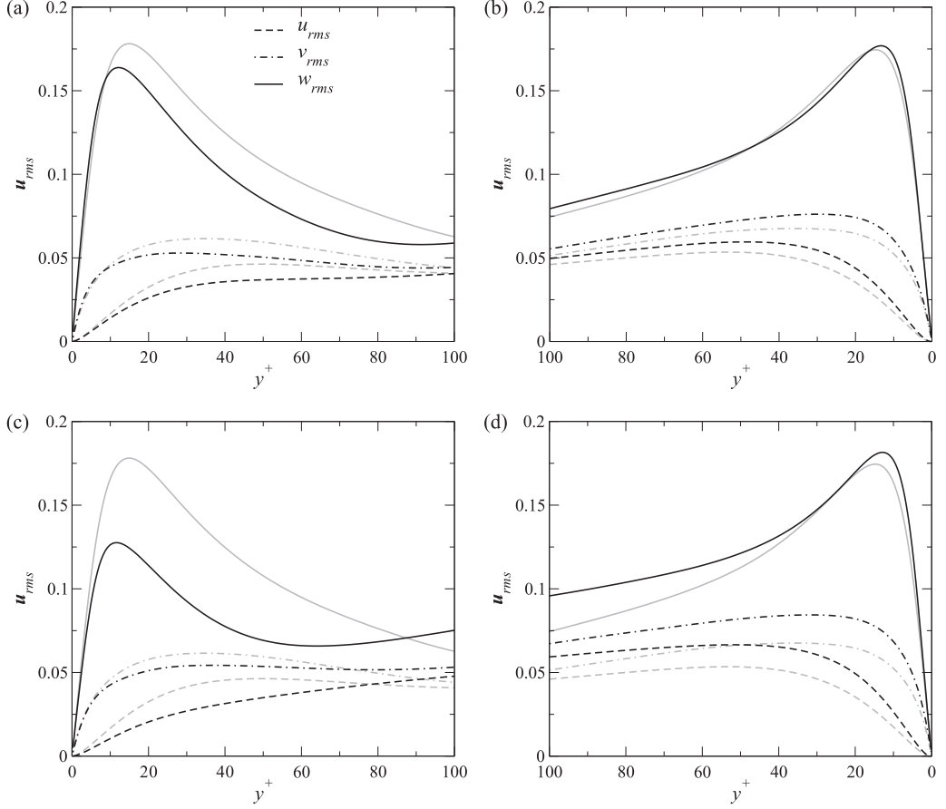
FIG. 6. Root mean square values of the velocity fluctuations. (a) forced convection sCO 2 case, inner wall region, (b) forced convection sCO 2 case, outer wall region, (c) mixed convection sCO 2 case, inner wall region, and (d) mixed convection sCO 2 case, outer wall region. The gray lines indicate rms values of the velocity fluctuations of the reference case.
