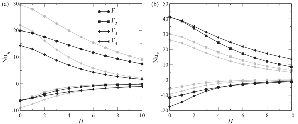
FIG. 17. Contributions of the turbulent heat flux events as a function of the hole size H in the mixed convection s\text{CO}_2 case (II) (black) and the reference case (I) (gray). (a) hot inner wall, (b) cold outer wall.
