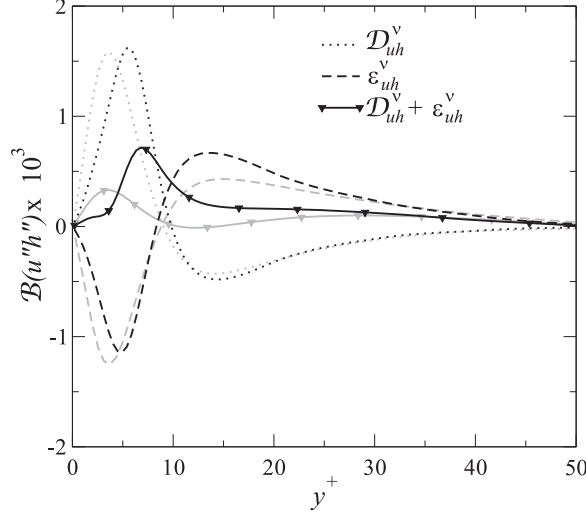
FIG. 13. Viscous parts of the diffusion and dissipation terms of the radial turbulent heat flux for reference case (I) and the forced convection sCO 2 case. The results of the reference case (I) are in gray.
