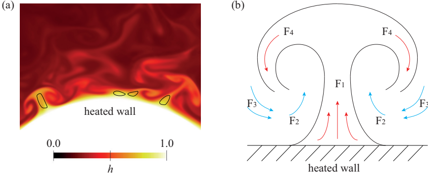
FIG. 14. (a) Typical mushroom structures near the hot wall of the annulus in the forced convection \text{sCO}_2 case. The black contour lines denote low-speed fluid regions (streaks). (b) A physical interpretation of the flux quadrants using the mushroom structure as an example.
