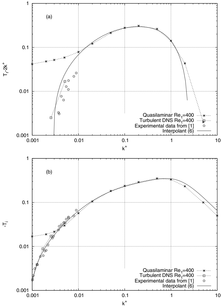
FIG. 2. Interpolation of the response function through a Padé approximant.
