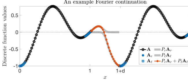
FIG. 13. An example illustration of the Fourier continuation method for a nonperiodic function A(x) = 1 - x^2 \sin(2\pi x - \pi/2) , x \in [0, 1] . The operators P_\ell , P_r construct extensions that blend to zero via a basis of continuations that are precomputed. The resulting function is discretely periodic on the marginally larger interval given by [0, 1 + d] .
