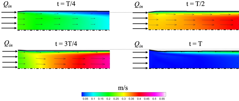
FIG. 16. Spatial distribution (pseudocolor plot) of fluid velocity amplitude simulated by the reference 3D axisymmetric ALE solver. Velocity vectors are overlaid as arrows. T represents the length of a full cycle and the dashed horizontal line represents the axis of symmetry. Results correspond to a flow source at a frequency of f = 5 Hz and DC = 1 .
