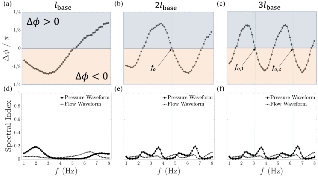
FIG. 6. The pressure-flow phase delay between (top row) and the spectral index (bottom row) as a function of inflow frequency for baseline primary tube lengths [(a) and (d)], twice the baseline [(b) and (e)], and three times the baseline [(c) and (f)]. The green dashed lines demarcate the location of the optimum frequencies. For all simulations, the same inflow waveform of duty cycle DC = 1 and the same reflection coefficient of \Gamma = 0.0 have been employed.
