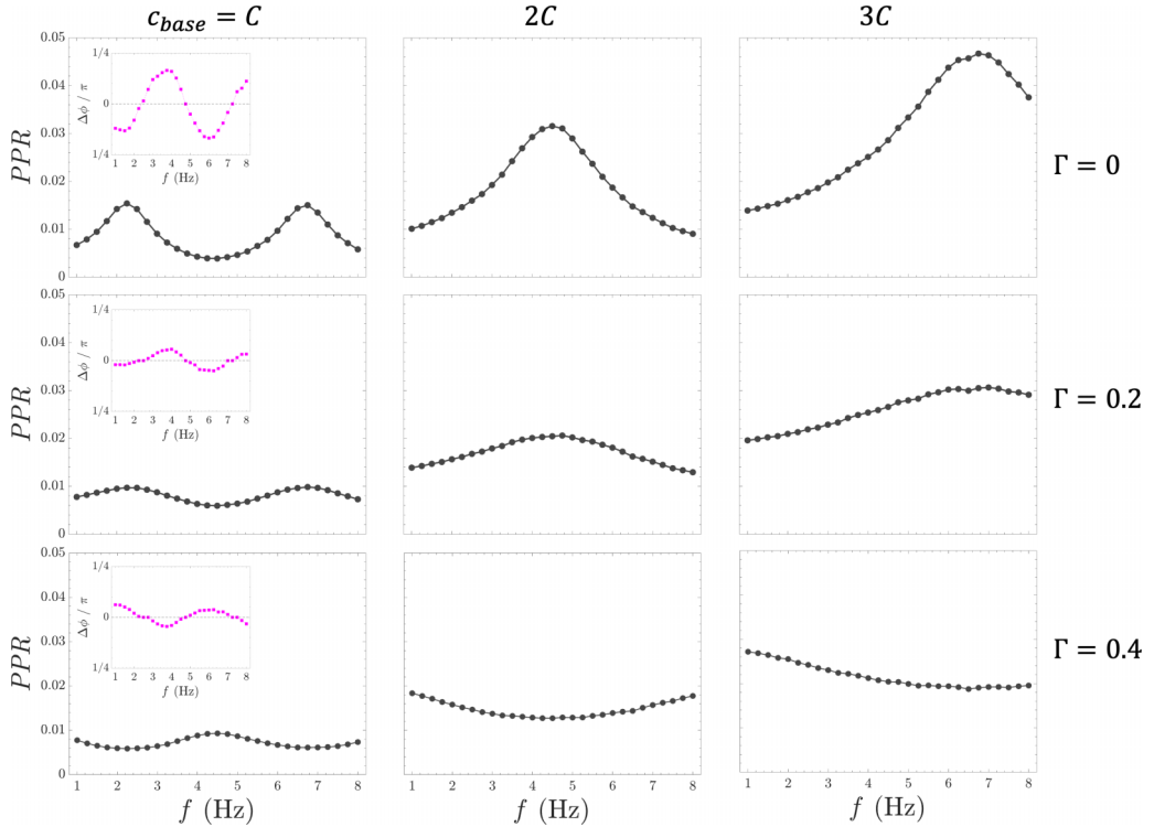
FIG. 11. Pulsatile power ratio (PPR) as a function of inflow frequency for different integer multiples of baseline primary tube wave speed (columns) and different reflection coefficients (rows). For all simulations, the same inflow waveform of duty cycle DC = 1 has been employed.
