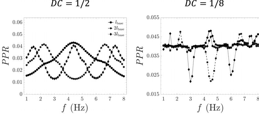
FIG. 7. The pulsatile power ratio ( PPR ) as a function of frequency f for three tube lengths that are multiplicative factors of the baseline length l_{\text{base}} given in Table I. Simulations were performed for two inflow waveform profiles with duty cycles of values DC = 1/2 and DC = 1/8 .
