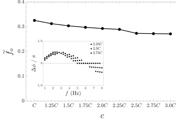
FIG. 12. The lowest value of the wave condition number (i.e., nondimensionalized optimum inflow frequency parameter) as a function of the primary tube wave speed phase delay profiles of three representative cases (inset). For all simulations, the same inflow waveform of duty cycle DC = 1 and the same reflection coefficient of \Gamma = 0.4 have been employed.
