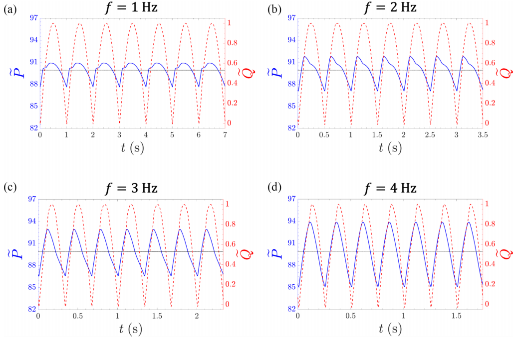
FIG. 4. Pressure (solid lines) and flow (dotted lines) waveforms at the data collection site (see Fig. 1) after reaching an oscillatory steady state for inflow frequencies of (a) 1 Hz, (b) 2 Hz, (c) 3 Hz, and (d) 4 Hz. Dotted line indicates the mean value for the pressure waveform over the cycle. Pressure is nondimensionalized by \rho U_{\max}^2 and flow is nondimensionalized by Q_{\max} .
