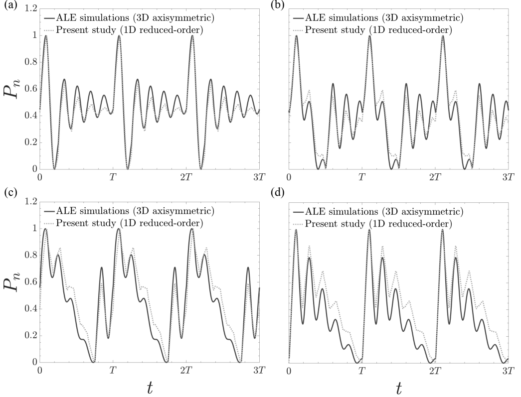
FIG. 2. Normalized pressure waveforms P_n at the inlet for a simple straight fluid-filled compliant tube simulated by the solver employed in this paper (dotted line) and by a 3D FSI solver (solid line) at duty cycles of (a) 1/4, (b) 1/2, (c) 3/4, and (d) 1. Results correspond to a flow source at a frequency of f = 1 Hz (see Fig. 1).
