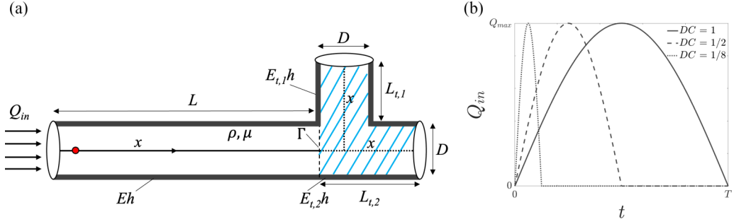
FIG. 1. (a) The physical problem of interest consisting of a straight cylindrical fluid-filled tube with the outlet connected to a reflection site (a bifurcation demarcated by a dashed line). Here, D is the diameter of the tube (and its terminals), L is the distance from the inlet to the reflection site (i.e., primary tube length), L_t is the length of the terminal tubes E (resp. E_t ) is the Young's modulus of the primary (resp. terminal), h is the tube thickness, \rho is fluid density, and \mu is fluid viscosity. The data collection site is indicated with red circle. (b) Examples for different duty cycles DC of the oscillatory time-dependent flow profiles applied at the inlet.
