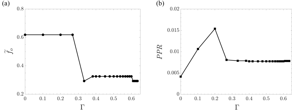
FIG. 10. (a) The lowest value of the wave condition number (i.e., the frequency at which the minimum pulsatile power is found, scaled by the ratio of the tube length to the wave speed: \tilde{f}_0 = f_0 \cdot L/c ) and (b) their corresponding pulsatile power ratios (PPRs) as a function of reflection coefficient at the primary tube outlet. For all simulations, the same inflow waveform of duty cycle DC = 1 has been employed.
