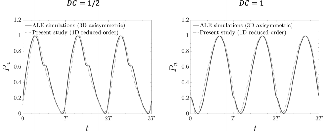
FIG. 15. Normalized pressure waveforms at the inlet for a fluid-filled compliant tube (connected to a reflection site with reflection coefficient \Gamma = 0.2 ) simulated by the solver employed in this paper (dotted line) and by a 3D FSI solver (solid line) at duty cycles ( DC ) of 1/2 and 1 .
