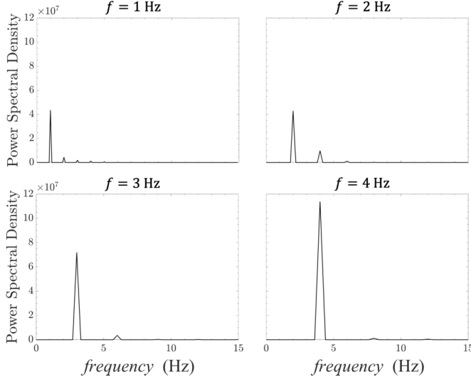
FIG. 17. The power spectral density (via FFT) of the pressure waveform at four sample inflow frequencies of f = 1 Hz, 2 Hz, 3 Hz, and 4 Hz. These curves correspond to the pressure profiles presented in Fig. 4.
