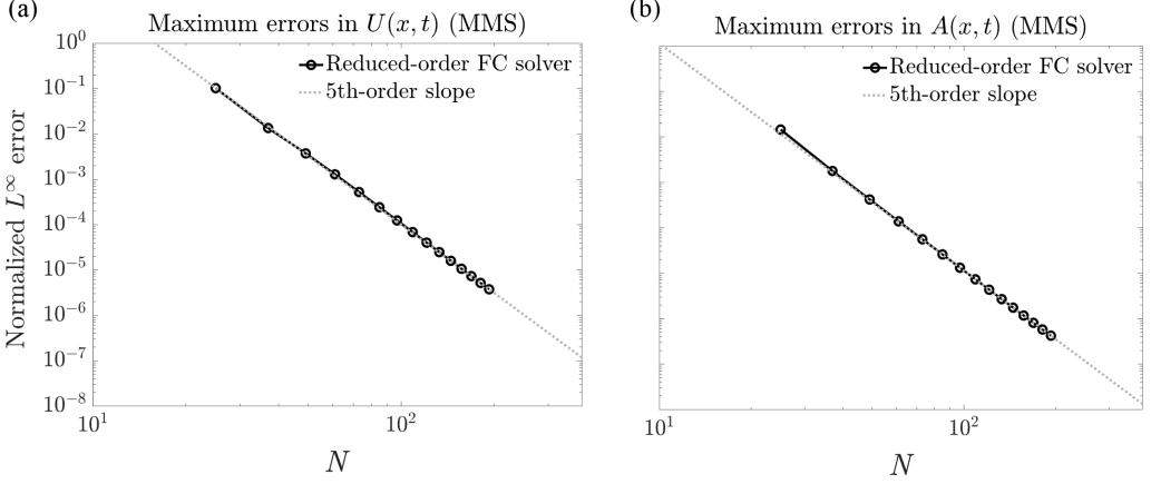
FIG. 14. Maximum errors (over all space and time) during one complete cycle ( t \in [0, 1] ) of velocity U(x, t) (left) and area A(x, t) (right) simulated by the FC solver applied to the manufactured right-hand side corresponding to the exact solution. Time steps are chosen small enough for each \Delta x so that errors are dominated by the spatial discretization (up to 64 000 time steps). The overlaid dashed lines (slopes) demonstrate the high-order accuracy (i.e., fifth order) of the numerical method employed in this work.
