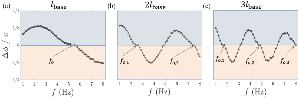
FIG. 19. The phase delay between pressure and flow at (a) baseline primary tube lengths, (b) twice the baseline primary tube length, and (c) three times the baseline primary tube length. For all simulations, the same inflow waveform of duty cycle DC = 1 and the same reflection coefficient of \Gamma = 0.5 have been employed.
