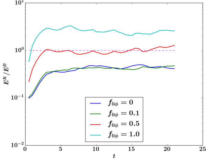
FIG. 11. The ratio of E^K to E^B for Run 1 to Run 4 supports the assumption of elastic equipartition ( \rho \langle \mathbf{v}^2 \rangle \sim \xi^2 \langle \mathbf{B}_\psi^2 \rangle ). If the forcing intensity is too strong, then the elastic forcing term in the \omega equation becomes negligible, and the system does not significantly differ from the 2D NS equation. In our study, though we tried a broad range of forcing intensity, larger forcing (than Run 5) may break the equipartition of the kinetic and magnetic energy.
