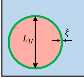
FIG. 4. The gradient length scales.
