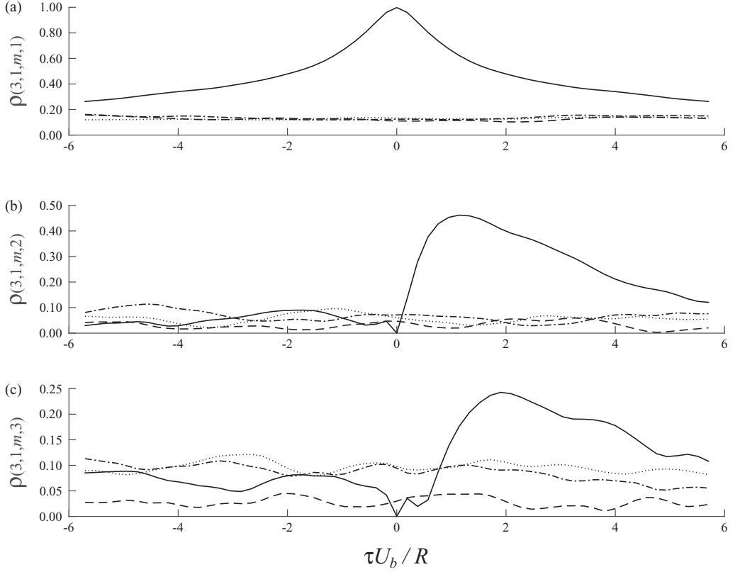
FIG. 5. Magnitude of the cross correlation of the reference POD coefficient \alpha^{(1)}(3;t) and the coefficients spanning m \in [1,4] and n \in [1,3] . Correlation is shown between the reference mode and (a) \alpha^{(1)}(m;t) , (b) \alpha^{(2)}(m;t) , and (c) \alpha^{(3)}(m;t) . The time-step offset has been scaled using the bulk velocity and pipe radius. \cdots represents m = 1 , \cdot - \cdot represents m = 2 , — represents m = 3 , and - - - represents m = 4 .
