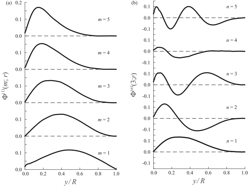
FIG. 2. Modal profile of the streamwise component of the POD modes. (a) First radial mode n = 1 and m \in [1,5] . (b) Third azimuthal mode number m = 3 and radial modes n \in [1,5] .
