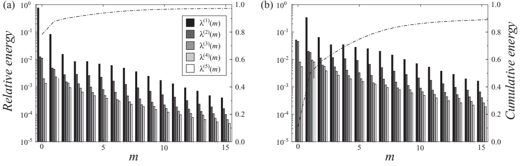
FIG. 1. Relative energy contribution of the first five POD modes n \in [1,5] , with azimuthal modes m \in [0,15] . Cumulative energy content of the first five POD modes is represented by -\cdot- . (a) Complete set of eigenvalues \lambda^n(m) , representing all deviation from the laminar flow field. (b) Same as in (a), but excluding the energy associated with the deviation of the laminar to turbulent mean velocity profile, resolved by (n,m) = (1,0) .
