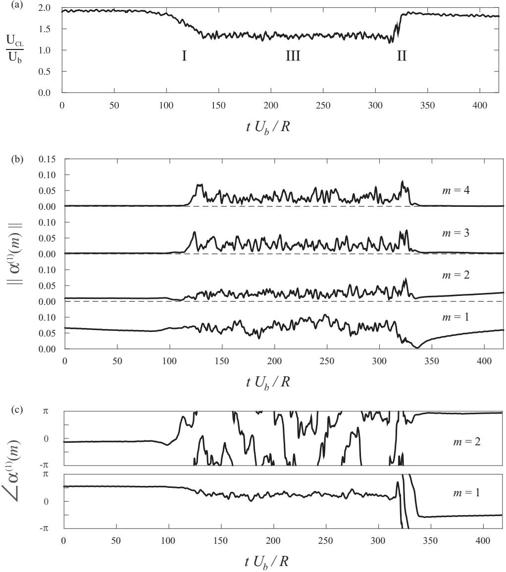
FIG. 4. Temporal activity of the flow field for data block 10. (a) Scaled centerline velocity. (b) Magnitude of POD coefficients \alpha^{(1)}(1; t) for n = 1 and m \in [1, 4] . (c) Azimuthal phase of POD coefficients \alpha^{(1)}(1; t) for n = 1 and m \in [1, 2] .
