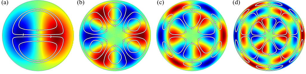
FIG. 3. Contour plots of the streamwise component of sample POD modes. Red represents positive and blue negative modal values, respectively. The streamlines indicate the in-plane components of the POD modes \Phi^{(m)}(m; r) : (a) \Phi^{(1)}(1; r) , (b) \Phi^{(1)}(3; r) , (c) \Phi^{(2)}(3; r) , and (d) \Phi^{(3)}(3; r) .
