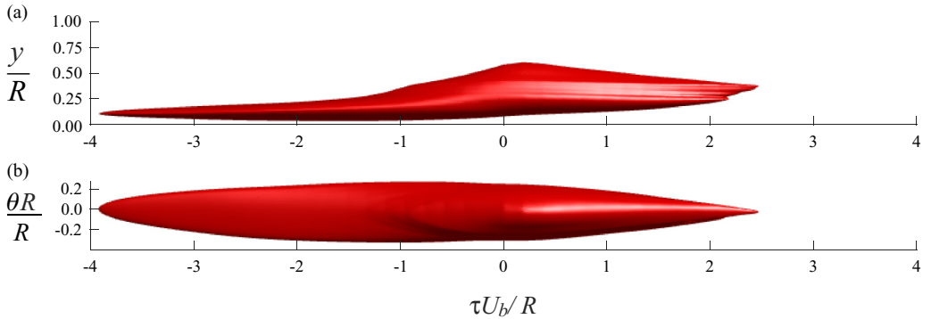
FIG. 6. Isosurface of an isolated spatiotemporal structure for m = 3 and n \in [1,5] . The isosurface value is chosen to be 50% of the maximum value. (a) Side view and (b) view from pipe centerline. Flow is from left to right.
