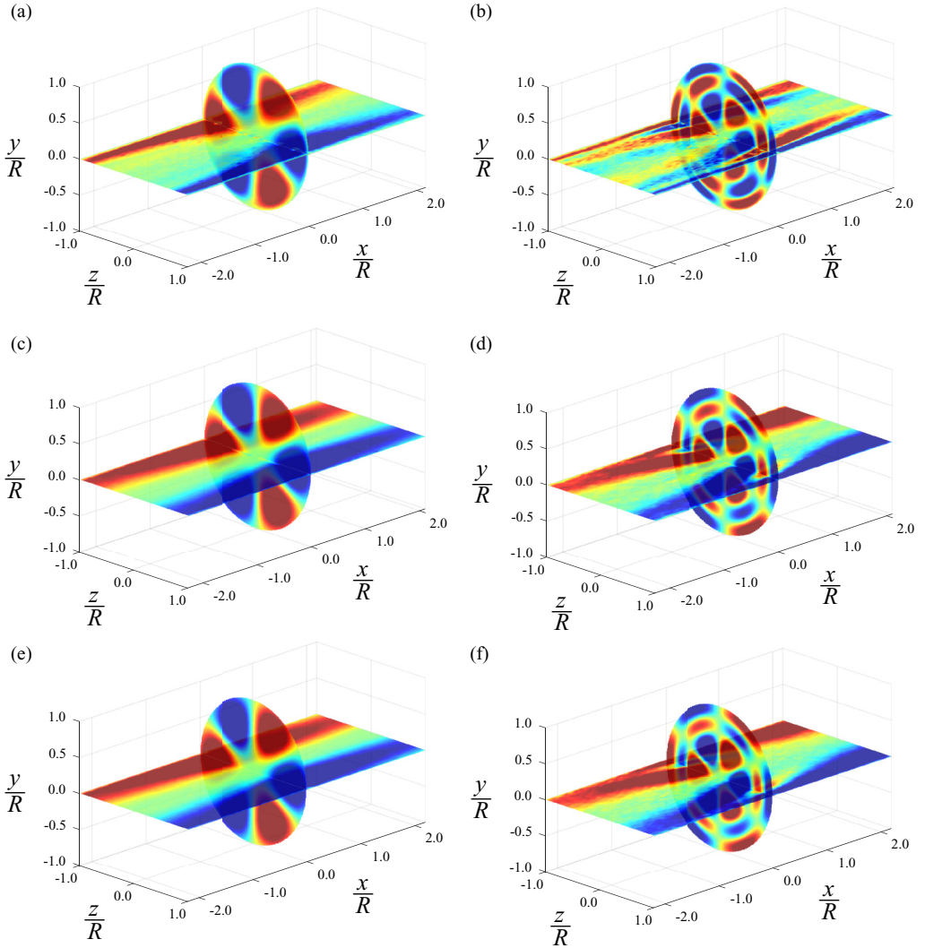
FIG. 7. Streamwise components of the dual-plane modes \Psi^{(m,n)}(\theta, r, x) : (a) \Psi^{(3,1)} and (b) \Psi^{(3,3)} at \text{Re}_D = 3440 , (c) \Psi^{(3,1)} and (d) \Psi^{(3,3)} at \text{Re}_D = 51\,700 , and (e) \Psi^{(3,1)} and (f) \Psi^{(3,3)} at \text{Re}_D = 104\,000 . Flow goes from left to right.
