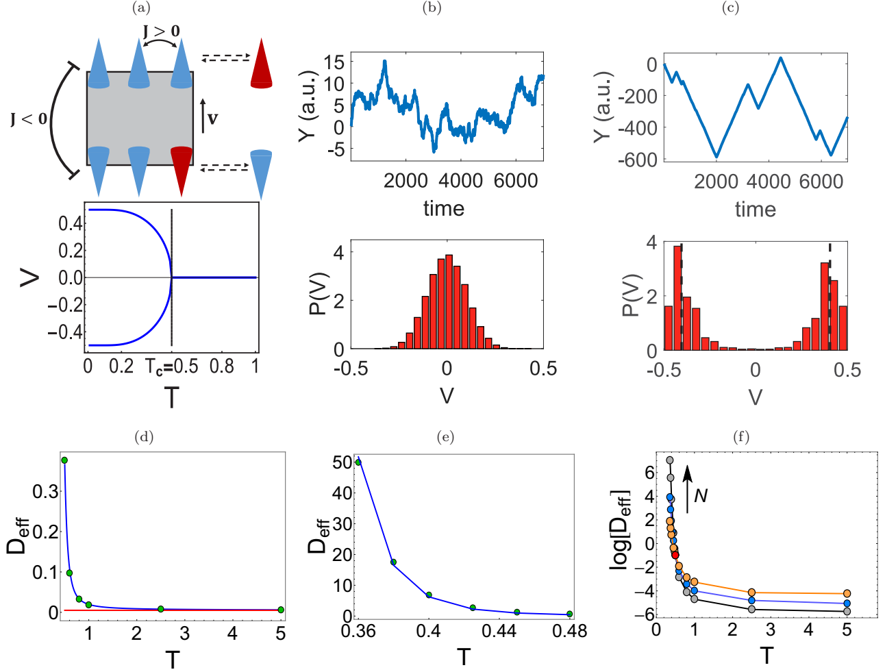
FIG. 3. (a) The upper panel is an illustration of the spin model in one dimension. The triangles represent the informed members in the group. Blue triangles represent the individuals that exert a social force ( \sigma_i = 1 ), while the red ones represent individuals that do not exert a force ( \sigma_i = 0 ) on the group [Eq. (2)]. Triangles pointing in the same direction are members of the same informed subgroup and tend to encourage each other into the pulling state [ferromagneticlike ( J_{ij} > 0 )], while they tend to suppress the members in the other subgroup into the nonpulling state [antiferromagneticlike interaction ( J_{ij} < 0 )]. In the schematic illustration there is an excess of blue members on the upper side and therefore the group moves in the positive direction, V > 0 . The lower panel shows stable solutions of Eq. (3). (b) Example of a trajectory for T = 1 > T_c and N_1 = N_2 = 25 . The motion looks like Brownian motion (top) and the velocity distribution is peaked at V = 0 (bottom). (c) Example of a trajectory for T = 0.36 < T_c and N_1 = N_2 = 25 . The motion looks like a run-and-tumble motion (top) and the velocity distribution is bimodal (bottom). Also shown (as dashed lines) are the solutions of Eq. (3) for T = 0.36 . (d) Spatial diffusion coefficient for T > T_c ( T_c = 1/2 ). Green points are estimated from simulation results. The blue curve is the numerical integration of Eq. (D12) and the red line is B/2 = (4N)^{-1} . (e) Spatial diffusion coefficient for T < T_c . Green points are estimated from simulation results. The blue curve is Eq. (6), where \alpha is estimated from simulations. (f) Spatial diffusion coefficient in semilogarithmic scale for different system sizes N = 24, 50, 100 estimated from simulation data (lines are guides to the eye). The diffusion coefficient at the critical point ( T_c = 1/2 ) is denoted by the red point and it has the same value for all the sizes [Eq. (D13)].
