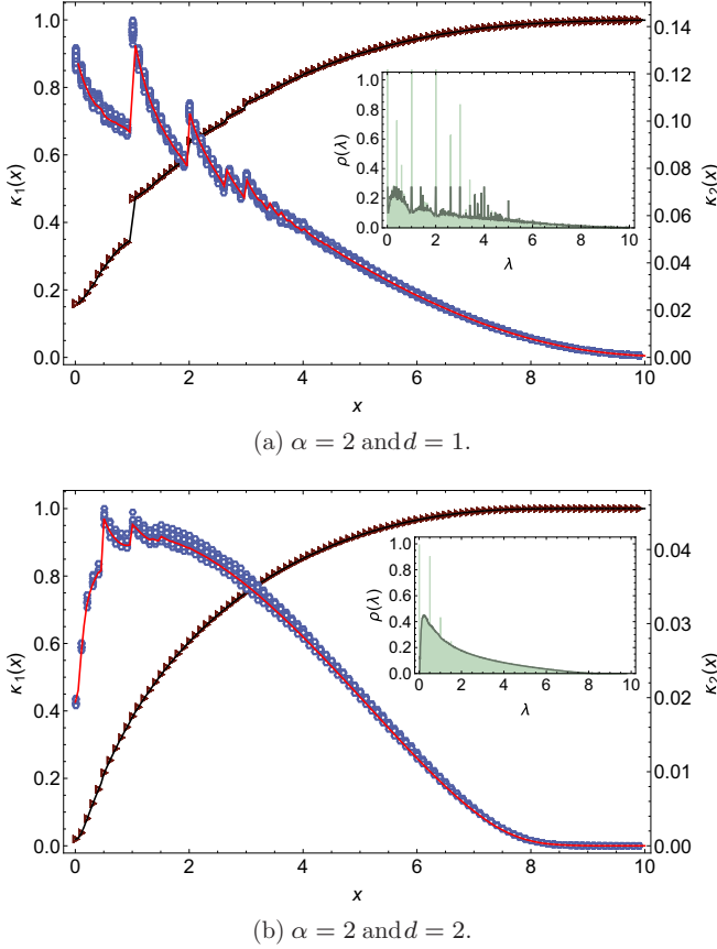
FIG. 1. The first and second cumulants of \mathcal{I}_N(x) as functions of x for different values of \alpha and d . The solid lines are obtained from the solution of Eqs. (12)–(14) using the weighted population dynamics method with \mathcal{L} = 10^7 and \epsilon = 10^{-8} (see Appendix B). The black curve is the mean value of \mathcal{I}_N(x) , whereas the red curve gives the variance of \mathcal{I}_N(x) . The markers correspond to results coming from numerical diagonalization of an ensemble with 10^4 sparse Wishart matrices of dimension N = 1000 . The insets display the average spectral density \rho(\lambda) for each pair of model parameters.
