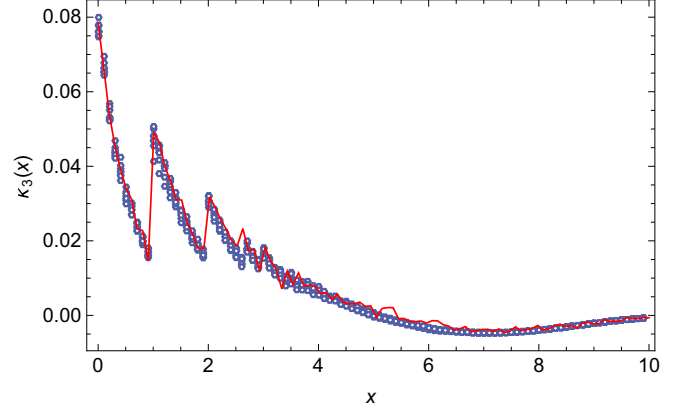
FIG. 2. The third cumulant of \mathcal{I}_N(x) as a function of x for (\alpha, d) = (2, 1) . The solid line has been obtained by evaluating the cumulant generating function \mathcal{F}_x(y) from Eq. (10) at seven points of y , followed by a finite-differences calculation of the third-order derivative of \mathcal{F}_x(y) . These results have been computed through the weighted population dynamics algorithm with \mathcal{L} = 10^6 and \epsilon = 10^{-8} . Moreover, each estimate of \mathcal{F}_x(y) has been averaged 100 times in order to reduce its fluctuations and improve the accuracy of the finite-differences calculation. The markers correspond to results coming from numerical diagonalization of an ensemble with 10^6 sparse Wishart matrices of dimension N = 300 .
