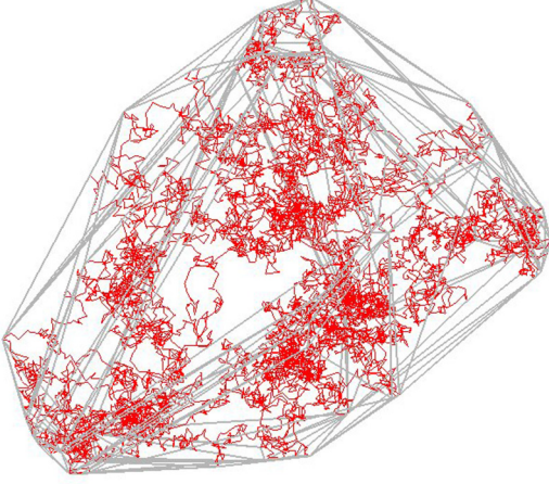
FIG. 1. A sample realization of three-dimensional Brownian motion and the facets on the boundary of its convex hull.
