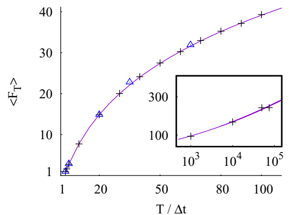
FIG. 2. Numerical simulations for the average number of triangular facets on the convex hulls of some three-dimensional Lévy processes (with 10^4 and 10^3 sample paths realizations): standard Brownian motion (pluses), and a stable process with stability index 1.5 (triangles). The solid line corresponds to the exact formula Eq. (14). The inset shows the asymptotics for large values of T/\Delta t , from Eq. (15), with numerical simulations of three-dimensional Brownian motion.
