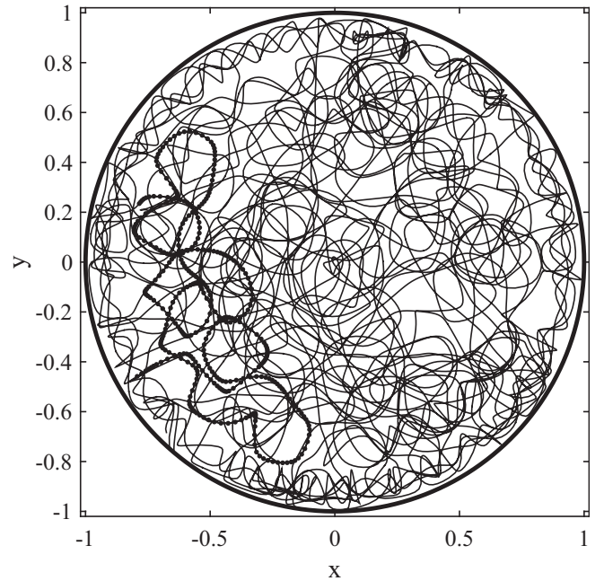
FIG. 5. Chaotic trajectory at memory M = 500 and C = 3 \times 10^{-5} . The solid line corresponds to 10 000 impacts, while the dots emphasize 380 of these successive impacts.
