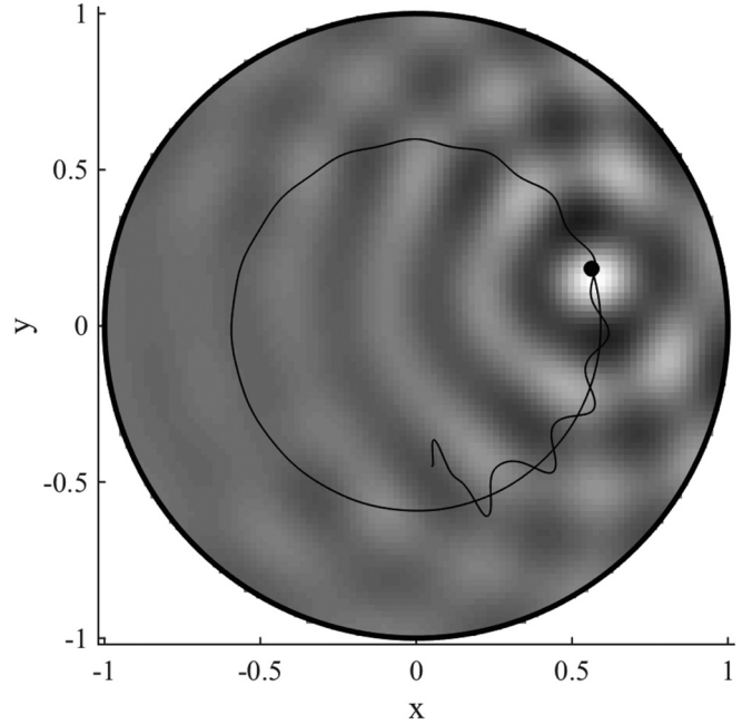
FIG. 2. Convergence to a stable circular orbit of type A ( r_1 = 0.592 , \alpha = 0.0135 ) at memory M = 7.7 and C = 3 \times 10^{-5} . The underlying wave-field corresponds to the time at which the walker is at the position indicated by the black circle ( \bullet ).
