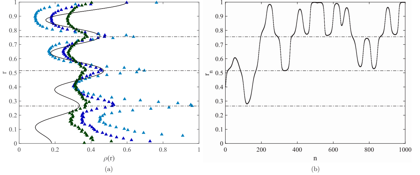
FIG. 7. (a) Probability distribution function \rho(r) of radial position r for mode subset \mathcal{S}_2 and three different values of C (Table II). The solid line corresponds to the quantum prediction given in Eq. (35). (b) An example of the time evolution of the particle's radial position for mode subset \mathcal{S}_2 and for C = 10^{-5} .
