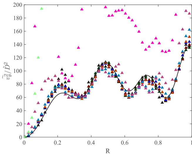
FIG. 13. Average variance of the tangential velocity \tilde{v}_\theta^2 of the walker at a given radial position r , normalized by \tilde{D}^2 , for subset \mathcal{S}_2 (Table II). The solid line corresponds to 2.0 times the quantum prediction [Eq. (44); best fit].
