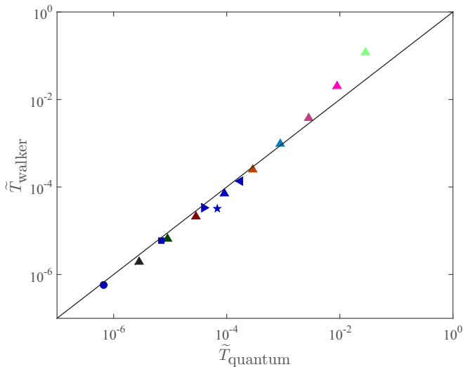
FIG. 11. Average dimensionless kinetic energy \tilde{T} of the walker, vs quantum prediction, with the equivalence B \equiv \tilde{D} . Symbols correspond to different mode subsets (Table II). The solid line is the quantum prediction [Eq. (38)].
