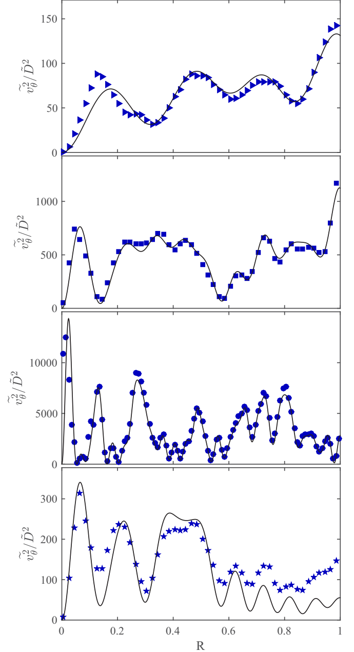
FIG. 14. Variance of the tangential velocity \tilde{v}_\theta^2 of the walker at a given radial position r , normalized by \tilde{D}^2 , for subsets \mathcal{S}_1 , \mathcal{S}_4 , \mathcal{S}_5 , and \mathcal{S}_6 , from top to bottom (Table II). The solid lines correspond respectively to 1.0, 2.1, 2.2, and 2.0 times the quantum prediction associated with each subset [Eq. (44); best fit].
