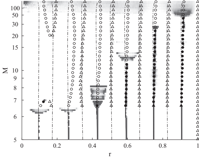
FIG. 3. Bifurcation diagram of the radial position r as a function of memory M at C = 3 \times 10^{-5} . The probability distribution function is represented in levels of gray; darker regions correspond to more frequently visited radial positions. Thick solid lines and thin dashed lines correspond to stable and unstable fixed points, respectively [Eq. (16)]. Full and empty symbols represent stable and unstable circular orbits, respectively [Eq. (15)]. Circles ( \circ ) indicate that at least one pair of eigenvalues is complex-conjugated (type A) while triangles ( \Delta ) are used when all corresponding eigenvalues are real-valued (type B).
