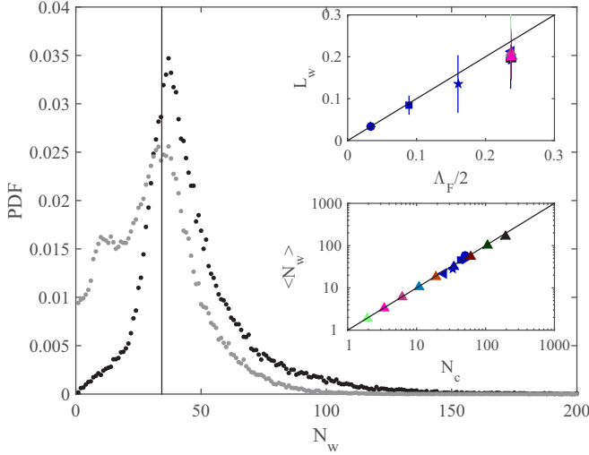
FIG. 10. Probability distribution function of the coherence time N_w for the two modes (k, \ell) = (0, 5) and (6, 3) of subset S_2 (in black and gray, respectively). The vertical line corresponds to N_w = N_c as defined in Eq. (23). Top inset shows average distance L_w traveled during a coherent segment N_w as a function of the half Faraday wavelength \Lambda_F/2 . Bottom inset shows average number of impacts \langle N_w \rangle of a coherent segment as a function of N_c . In both insets, data from all subsets are represented with different symbols (Table II), and the solid line corresponds to equal abscissa and ordinate.
