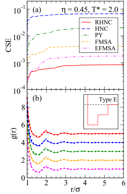
FIG. 8. (Color online) Radial distribution functions and cumulative squared errors for the type-E interaction. Series and labeling are as in Fig. 5.
