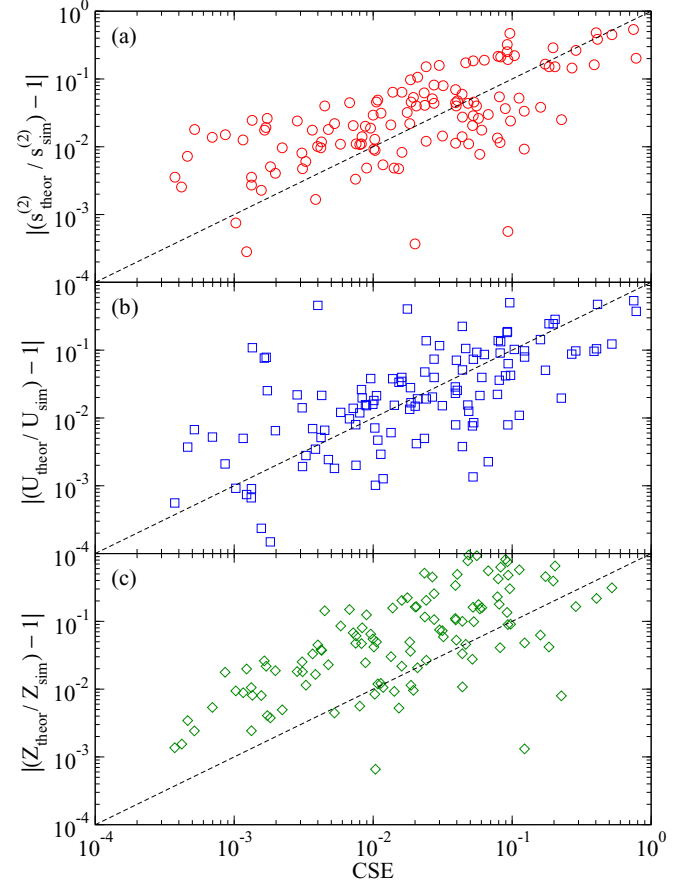
FIG. 4. (Color online) Correlations between total cumulative squared error CSE_\infty and (a) absolute normalized two-body excess entropy error (circles), (b) absolute normalized potential energy error (squares), and (c) absolute normalized compressibility factor error (diamonds) for all data collected.
