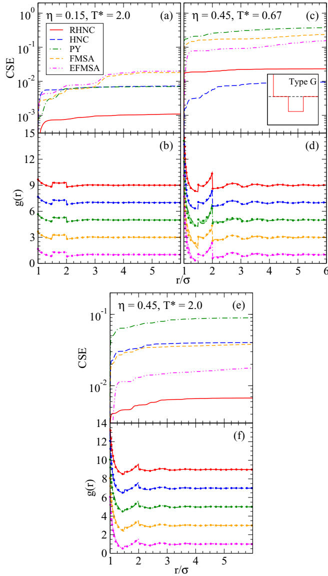
FIG. 10. (Color online) Radial distribution functions and cumulative squared errors for the type-G interaction. Series and labeling are as in Fig. 5.
