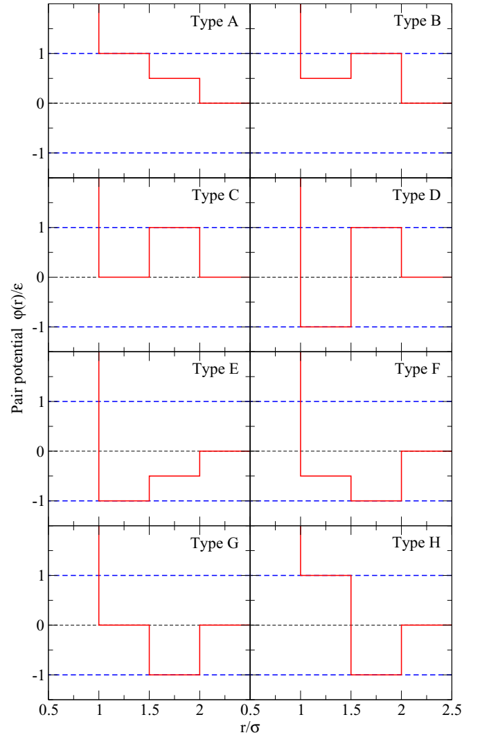
FIG. 1. (Color online) The suite of eight pair interactions considered in this study, inspired by Santos et al. [40], is topologically exhaustive (e.g., there are no other qualitative arrangements of two constant pairwise pieces that are not more appropriately labeled single wells or shoulders). For each of the eight interactions, the dimensionless pair potential is shown by the red solid line.
