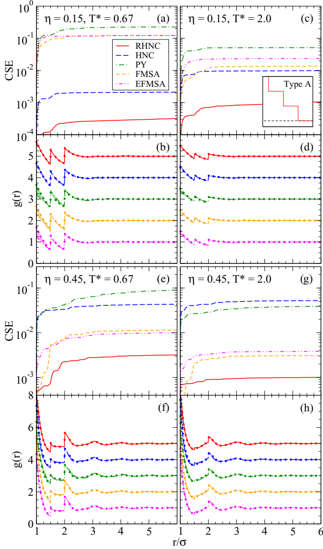
FIG. 2. (Color online) Radial distribution functions g(r) = h(r) + 1 and the associated cumulative squared errors [see Eq. (8)] predicted by the reference hypernetted-chain, hypernetted-chain, and Percus-Yevick Ornstein-Zernike closures [12,41]; the first-order mean spherical approximation solution [33]; and the simple exponential first-order mean spherical approximation [34] for the type-A pair interaction. For clarity, unit vertical offsets were applied to the RDF curves and they are stacked in the same order (top to bottom) as listed in the legend. The simulated RDF (closed circles) for this state point is reproduced five times to compare with each vertically offset theoretical RDF; shaded regions adjacent to each g(r) highlight the differences between each theory and simulation results.
