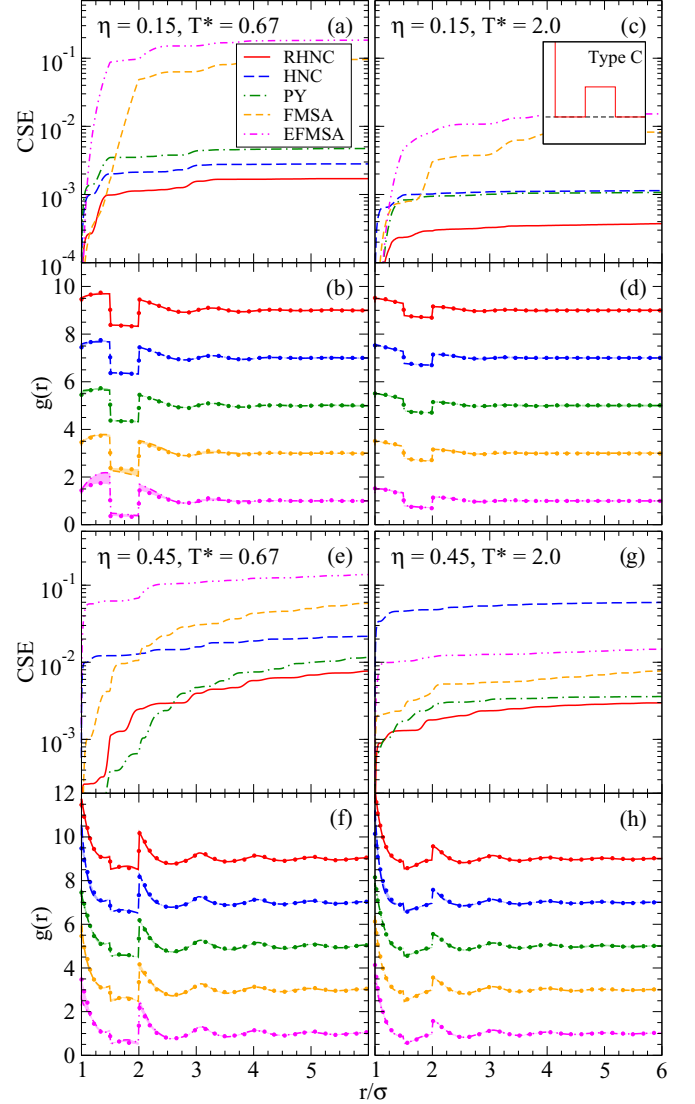
FIG. 6. (Color online) Radial distribution functions and cumulative squared errors for the type-C interaction. Series and labeling are as in Fig. 5.
