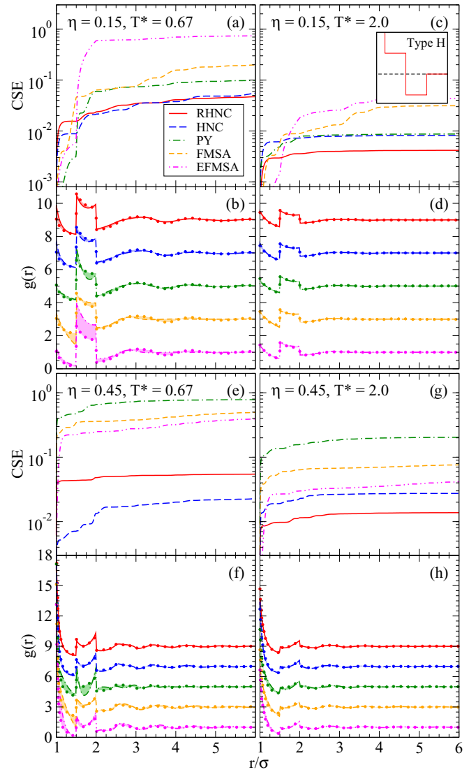
FIG. 11. (Color online) Radial distribution functions and cumulative squared errors for the type-H interaction. Series and labeling are as in Fig. 5.
