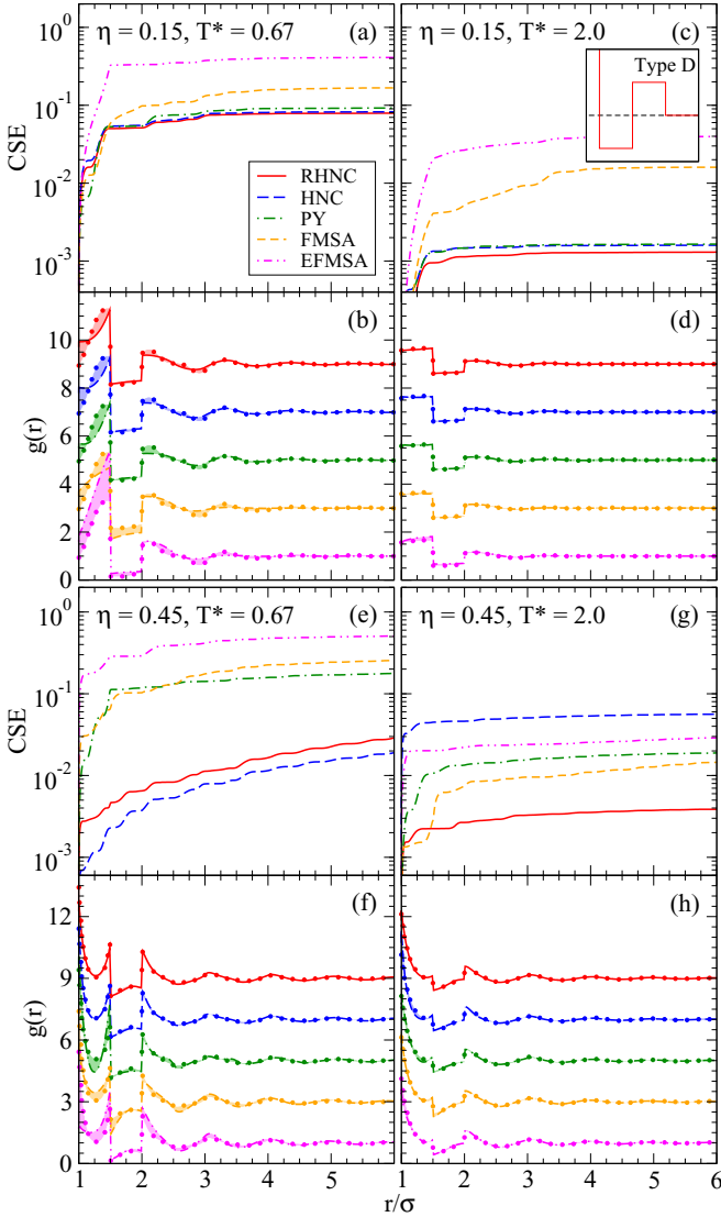
FIG. 7. (Color online) Radial distribution functions and cumulative squared errors for the type-D interaction. Series and labeling are as in Fig. 5.
