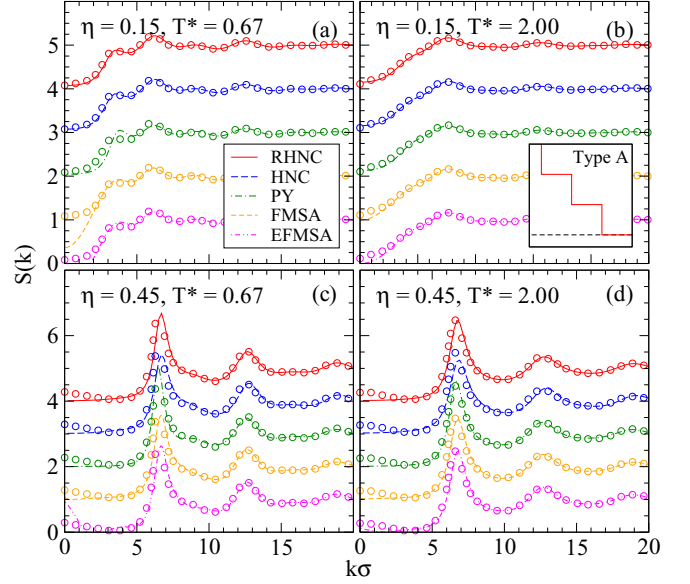
FIG. 3. (Color online) Structure factors S(k) predicted by the reference hypernetted-chain, hypernetted-chain, and Percus-Yevick Ornstein-Zernike closures [12,41]; the first-order mean spherical approximation solution [33]; and the simple exponential first-order mean spherical approximation [34] for the type-A pair interaction. For clarity, unit vertical offsets were applied to the structure factor curves and they are stacked in the same order (top to bottom) as listed in the legend. The simulated structure factor (open circles) for this state point is reproduced five times to compare with each vertically offset theoretical S(k) .
