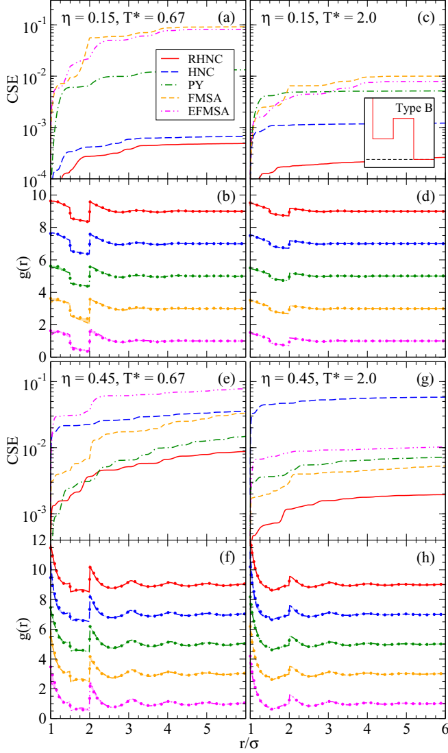
FIG. 5. (Color online) Radial distribution functions g(r) = h(r) + 1 and the associated cumulative squared errors [see Eq. (8)] predicted by the reference hypernetted-chain, hypernetted-chain, and Percus-Yevick Ornstein-Zernike closures [12,41]; the first-order mean spherical approximation solution [33]; and the simple exponential first-order mean spherical approximation [34] for the type-B pair interaction. For clarity, unit vertical offsets were applied to the RDF curves and they are stacked in the same order (top to bottom) as listed in the legend. The simulated RDF (closed circles) for this state point is reproduced five times to compare with each vertically offset theoretical RDF; shaded regions adjacent to each g(r) highlight the differences between each theory and simulation results.
