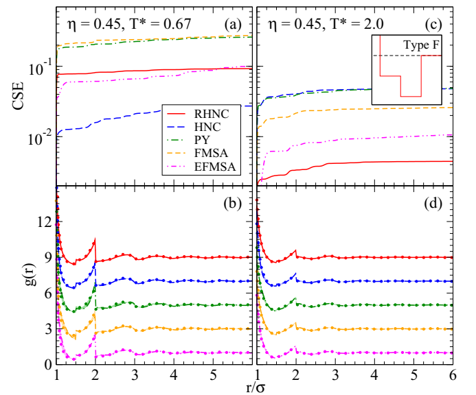
FIG. 9. (Color online) Radial distribution functions and cumulative squared errors for the type-F interaction. Series and labeling are as in Fig. 5.
