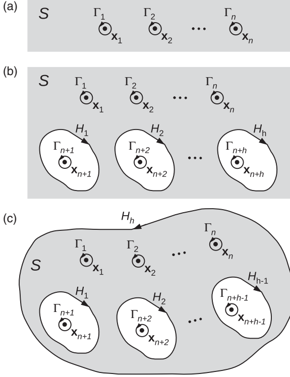
FIG. 1. Notations for (a) an unbounded planar domain, (b) an unbounded planar domain with holes, and (c) a bounded planar domain with holes. In the domain S , n phase singularities are located at \mathbf{x}_1, \dots, \mathbf{x}_n and encircled by closed contours \Gamma_1, \dots, \Gamma_n ; h holes and boundaries H_1, \dots, H_h are present, the last one being the exterior boundary (if any); arrows show the orientation of the contours \Gamma_k and H_k ; and inside each hole H_k , a “virtual” phase singularity is placed at \mathbf{x}_{n+k} and is encircled by the closed contour \Gamma_{n+k} .
