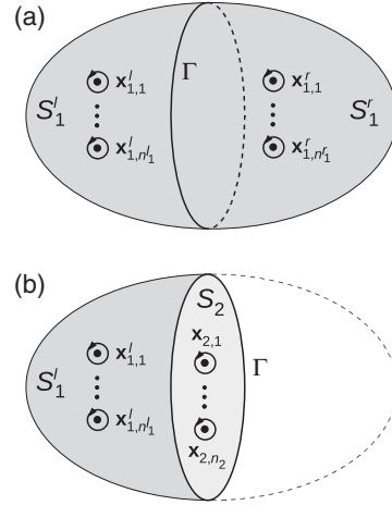
FIG. 2. Notations for a nonmanifold geometry schematically representing the atria. (a) Outer surface S_1 with spherical topology composed of a right part S_1^r and a left part S_1^l separated by the curve \Gamma ; (b) the right part is removed to make the S_2 surface (“septum”) visible. In the outer surface S_1 , n_1^r phase singularities are placed in the right part and n_1^l phase singularities are placed on the left part. The surface S_2 contains n_2 phase singularities. The curve \Gamma makes the connection between S_1 and S_2 .
