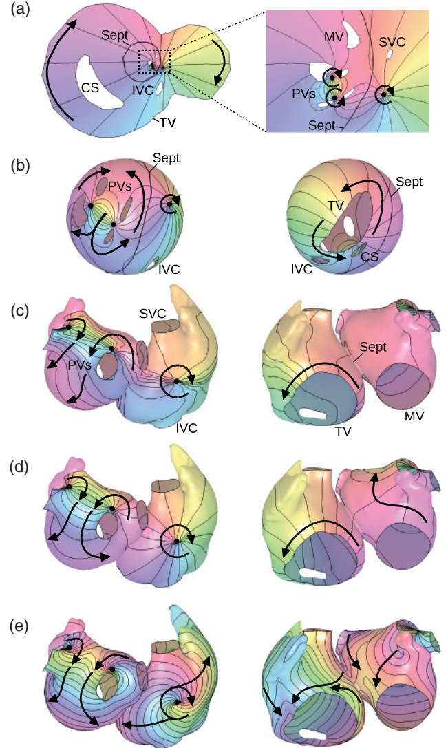
FIG. 3. (Color online) Successive steps for the generation of a phase map with three phase singularities in a surface model of the atria. (a) Phase map computed on the plane; a zoom of the central rectangular region is displayed on the right; (b) the same phase map projected on the sphere using the inverse stereographic projection; (c) the same phase map projected on the atrial surface (posterior view on the left, anterior view on the right); (d) phase map after smoothing; and (e) phase map after spirallike pattern enhancement. Phase is color coded (grayscale coded); 16 isochrones are shown as black solid lines. Arrows represent the direction of propagation (phase gradient). TV, tricuspid valve; MV, mitral valve; PVs, pulmonary veins; IVC, inferior vena cava; SVC, superior vena cava; CS, coronary sinus; Sept, septum.
