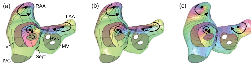
FIG. 4. (Color online) Generation of a phase map in a nonmanifold with three phase singularities in a surface model of the atria including a septal wall (front view). (a) Phase map constructed independently in the epicardium and in the septum; (b) phase map after correction for continuity; (c) phase map after smoothing and spirallike pattern enhancement. Phase is color coded (gray-scale coded); 16 isochrones are shown as black solid lines. Arrows represent the direction of propagation (phase gradient). RAA, right atrium appendage; LAA, left atrium appendage; TV, tricuspid valve; MV, mitral valve; IVC, inferior vena cava; PVs, pulmonary veins; Sept, septum; FO, fossa ovalis.
