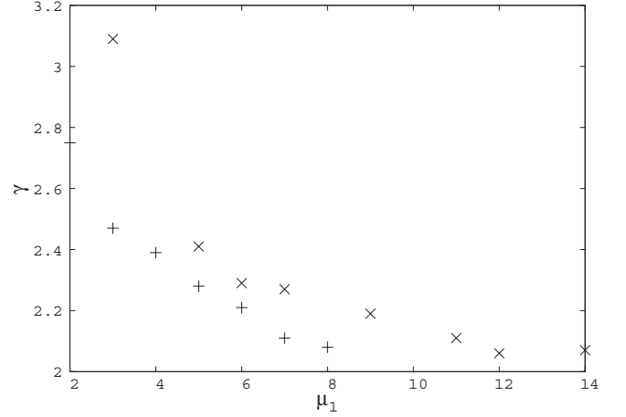
FIG. 2. Convergence of the \gamma exponent to the predicted value \gamma = 2.0 in the region above the line of the transcritical bifurcation. \mu_0 = 3 for the upper curve (x) and \mu_0 = 2 for the lower curve (+). All simulations were done for 100 000 nodes.
