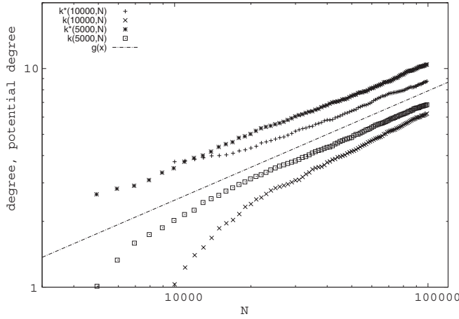
FIG. 3. Log-log plot of the degree and potential degree development with the size of the GCNN network for two different nodes ( s = 5000, 10000 ). k(s, N) [ k^*(s, N) ] is a degree (potential degree) of node s and network size N . The line has a slope \frac{1}{2} (71).
