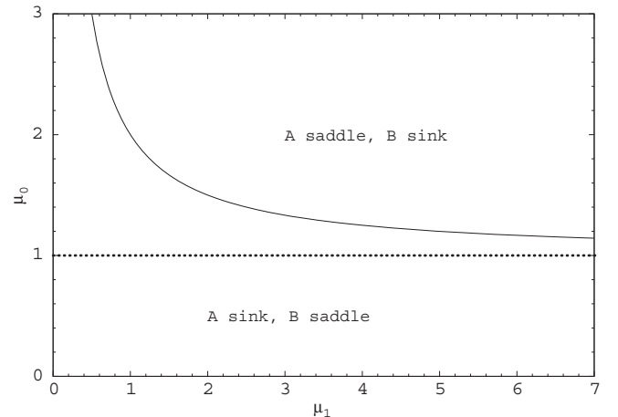
FIG. 1. Bifurcation line obtained from Eq. (32) in the parameter space of the CNN model delimiting regions of different stability types of fixed points of Eqs. (11) and (12). Dotted horizontal line indicates an asymptotic behavior when \mu_1 \rightarrow \infty .
