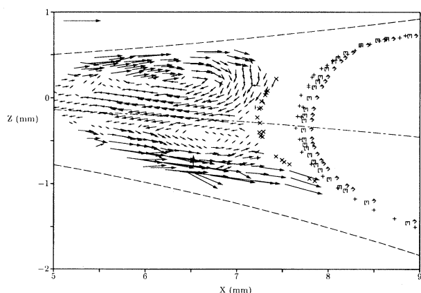
FIG. 3. Experimental 2D velocity vector plot at h_0 = 0.64 mm, Ca_1 = Ca_2 = 0.14 . The scaling vector in the upper left corner is 2 mm/s long. Meniscus shapes: PIV (crosses); laser fluorescence (pluses); numerical simulation, Q/Uh_0 = 0.65 (squares), Q/Uh_0 = 0.7 (diamonds).
