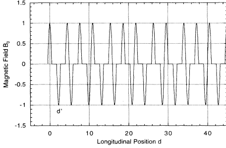
FIG. 2. Magnetic field distribution along the axis of the quasiperiodic undulator. Here B_0 denotes the peak field of the magnet block and d the length. We assume that the magnetic field in the magnet region is sinusoidal and that there is no magnetic field in spacer region.
