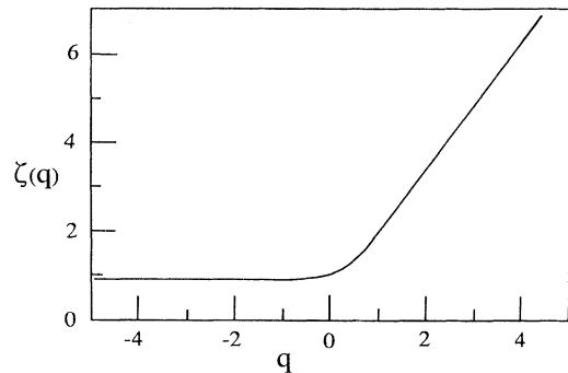
FIG. 3. Behavior of the scaling exponent \zeta(q) against q .
