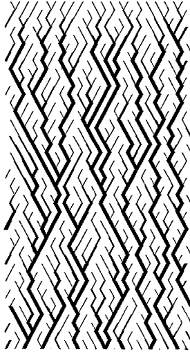
FIG. 1. Typical river-network pattern generated by the Scheidegger river-network model. This run was done on a 20 \times 40 square lattice under a periodic lateral boundary condition for an illustration. The width of lines is proportional to the flow rate through each bond where larger flow rates than 8 are indicated by the same width.
